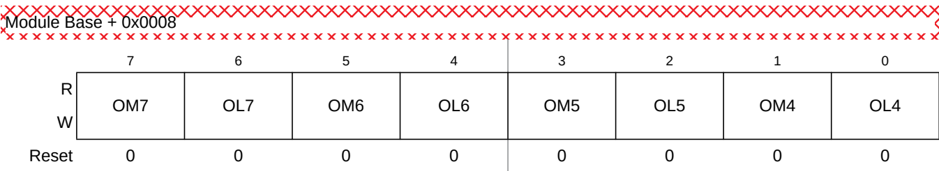
Figure 14-14. Timer Control Register 1 (TCTL1)
