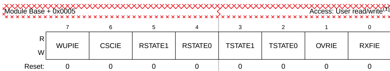
Figure 8-9. MSCAN Receiver Interrupt Enable Register (CANRIER)
