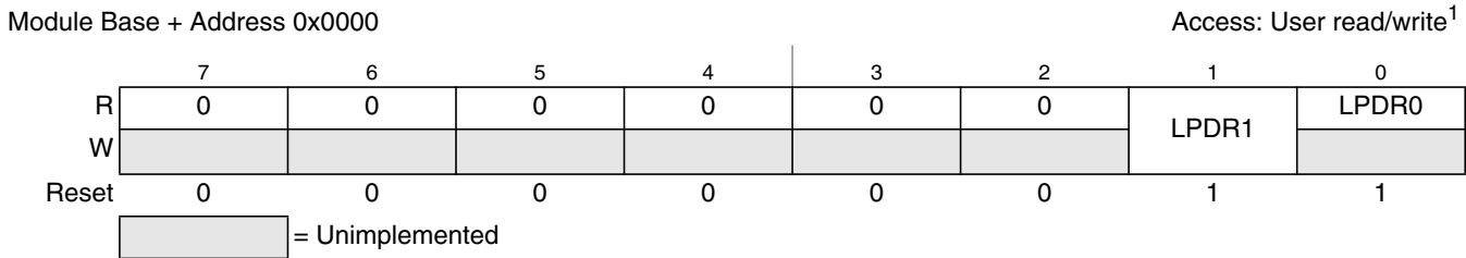
Figure 15-3. Port LP Data Register (LPDR)
