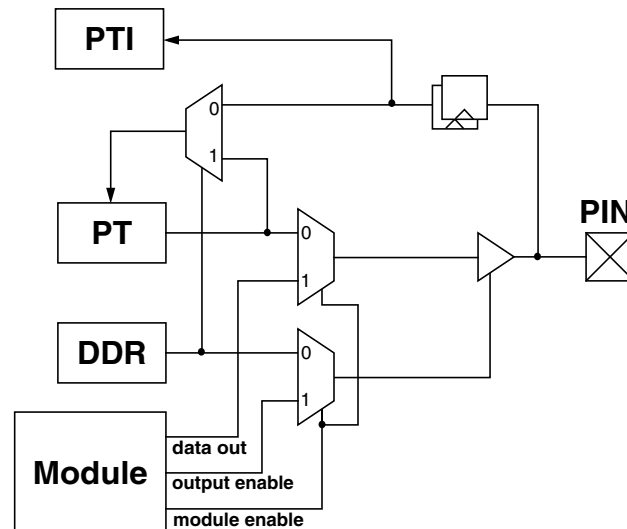
Figure 2-45. Illustration of I/O pin functionality
