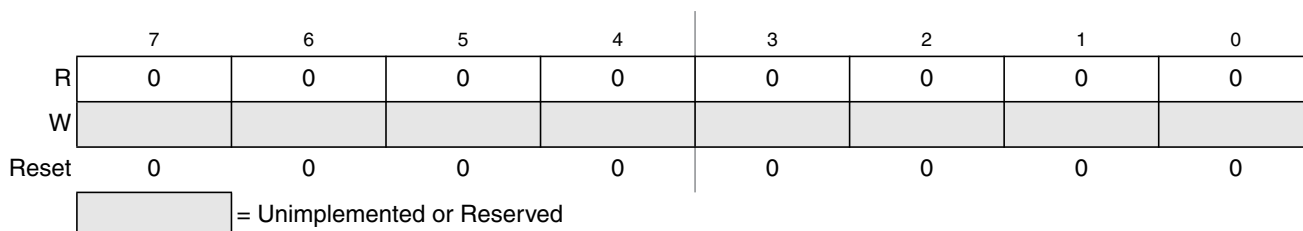
Figure 17-24. Flash Reserved7 Register (FRSV7)
