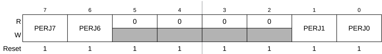
Figure 2-60. Port J Pull Device Enable Register (PERJ)
