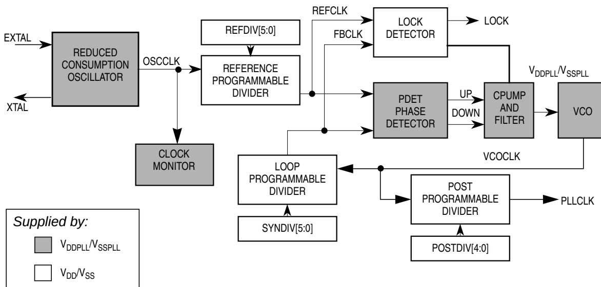
Figure 8-15. IPLL Functional Diagram
