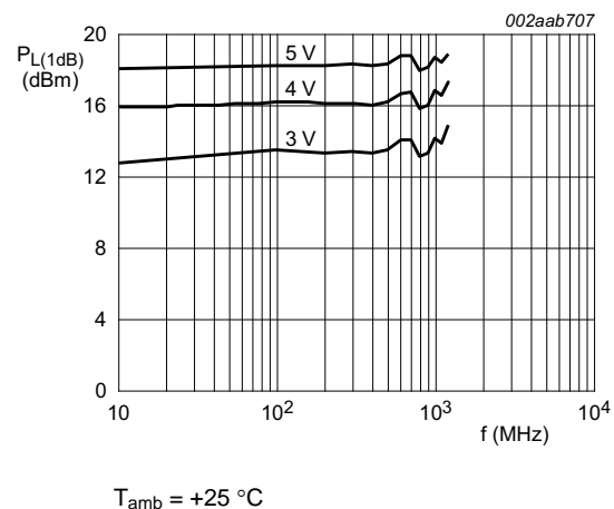
Fig 15. P_{L(1dB)} versus frequency and V_{DD}
