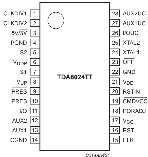
Fig 3. Pin configuration TDA8024TT
