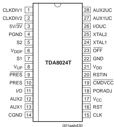
Fig 2. Pin configuration TDA8024T
