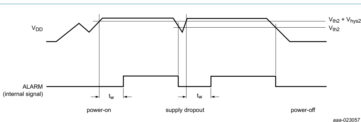
Fig 5. Voltage supervisor
