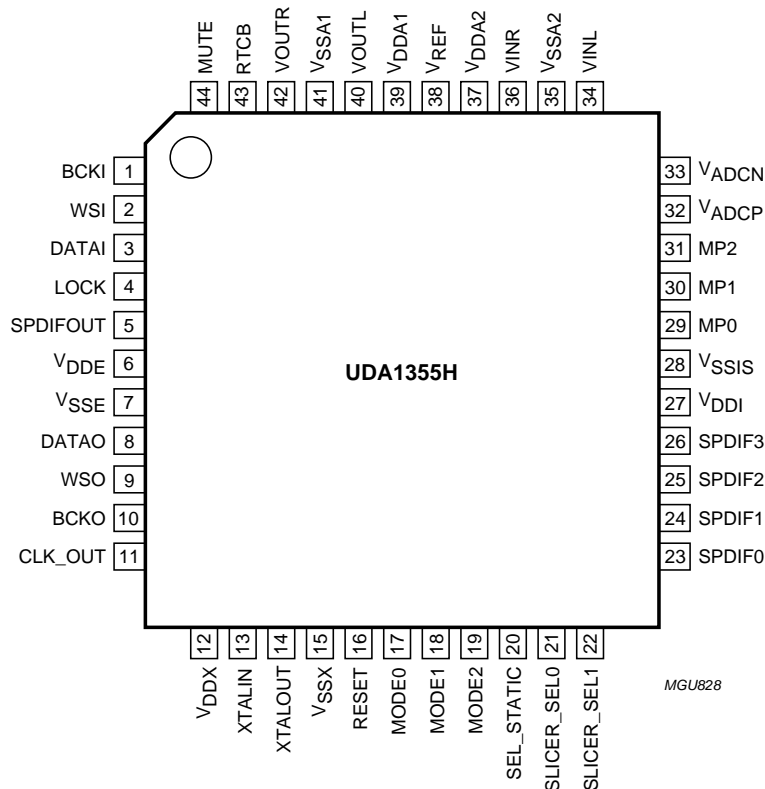
Fig.2 Pin configuration.
