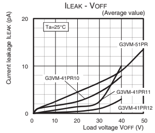
G3VM-41PR12/41PR10/41PR11/51PR
