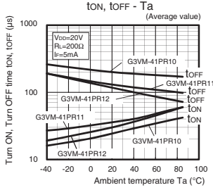
G3VM-41PR12/41PR10/41PR11
