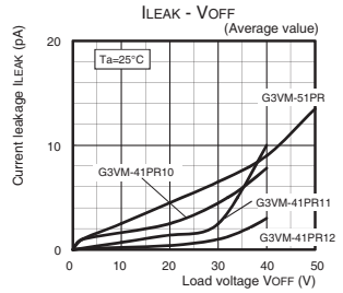
G3VM-41PR12/41PR10/41PR11/51PR
