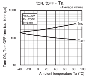
G3VM-51PR
