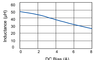
[ ETQP5M470YFK ]
