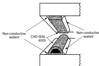
Figure 2-3. "Seal-to-seal" design incorporating CHO-SEAL 6503 conductive nickel-aluminum gaskets on both mating flange surfaces. Gaskets are bonded and edge sealed to prevent moisture from entering the gasket/flange area.
