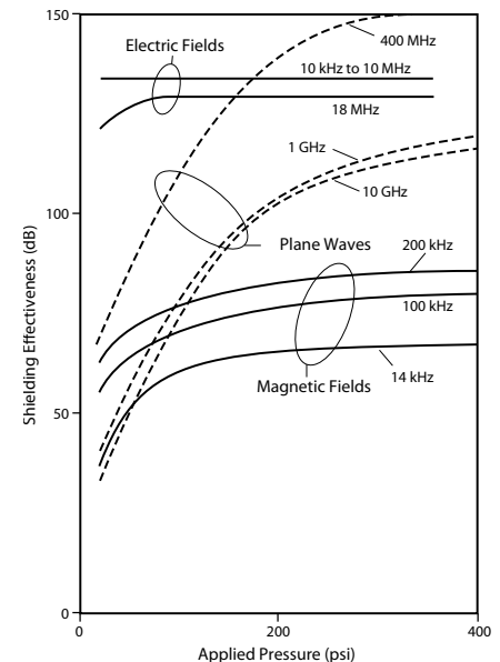
Figure 1-14. Shielding Effectiveness vs. Applied Pressure
