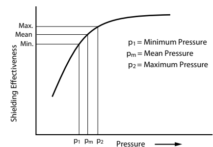
Figure 1-15. Typical Gasket Performance Curve
