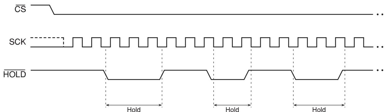
Figure 28. Hold Mode
