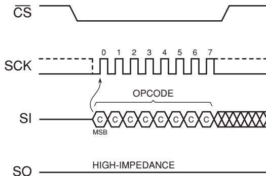
Figure 13. Chip Erase
