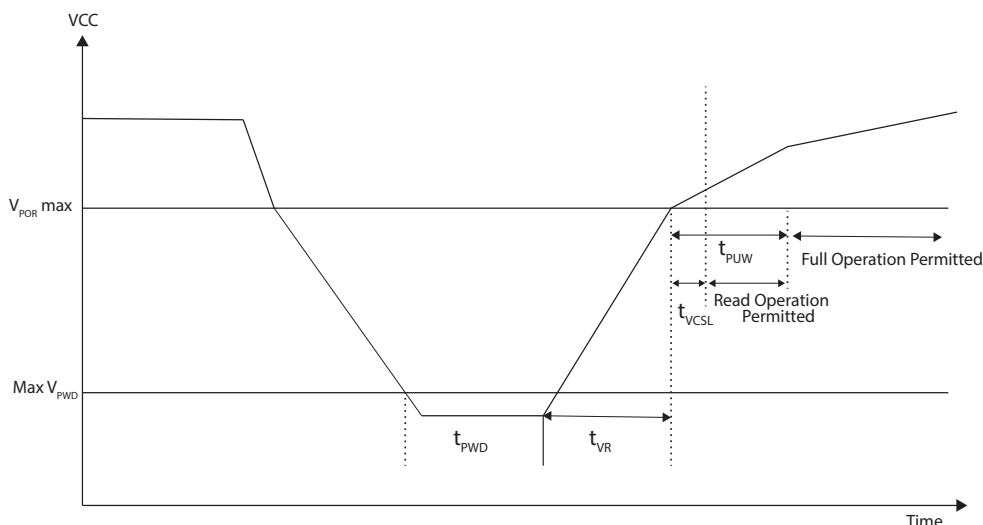
Figure 23. Power-Up Timing
