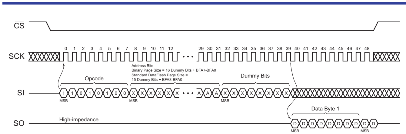
Figure 42. Buffer Read (Opcode D4h)
