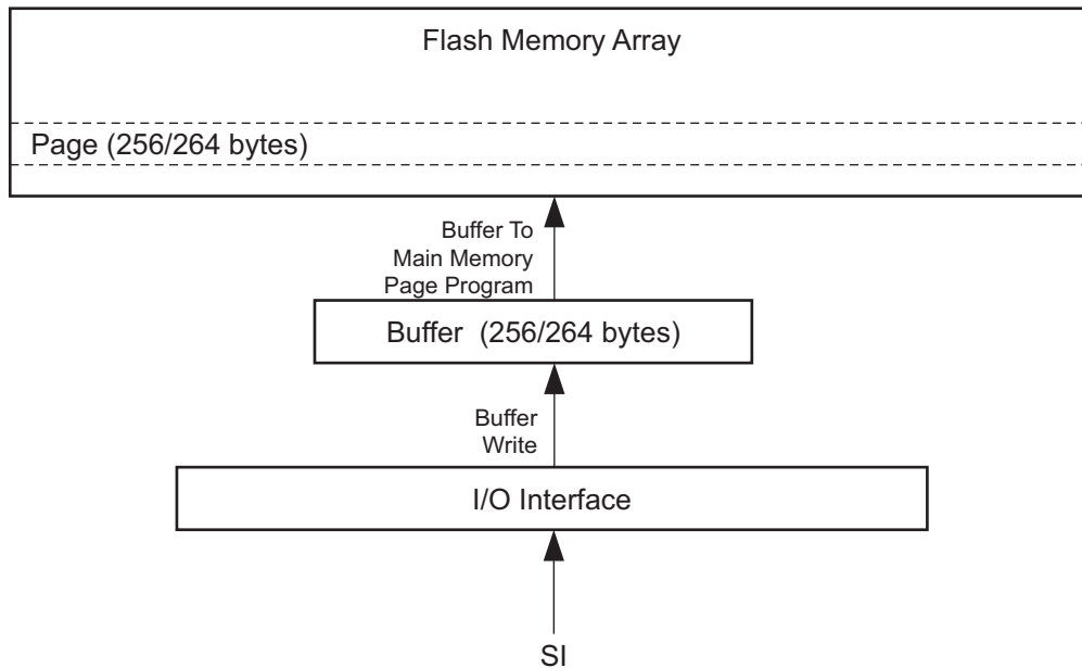
Figure 31. Block Diagram
