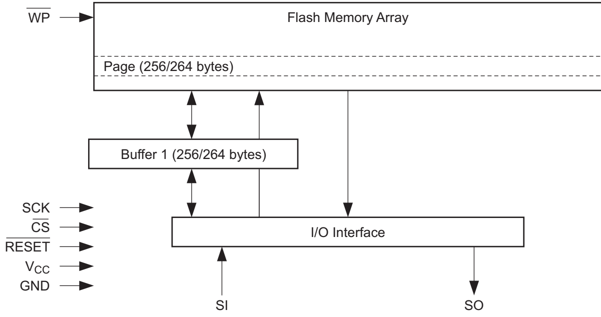
Figure 2. Block Diagram
