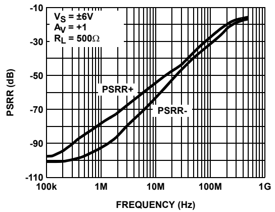
FIGURE 28. PSRR
