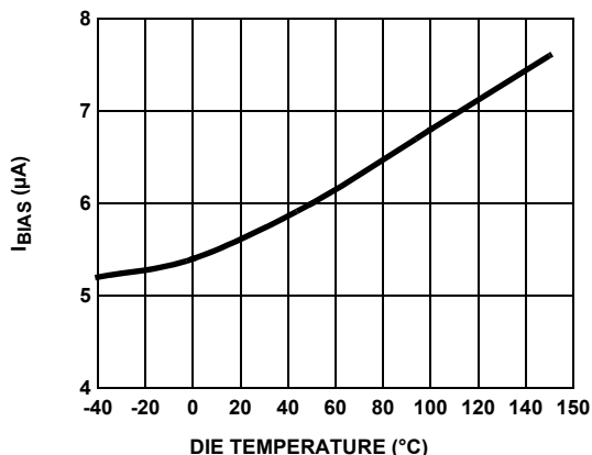
FIGURE 41. I_{BIAS} CURRENT vs TEMPERATURE
