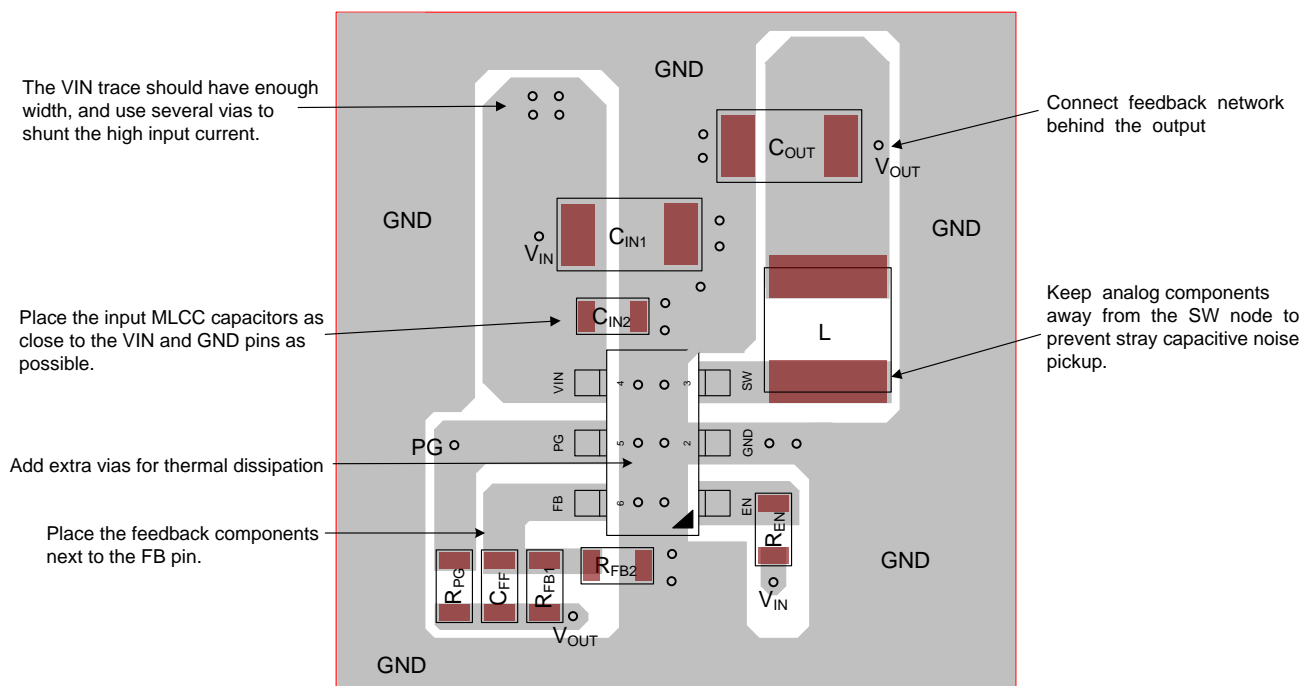
Figure 11. Layout Guide
