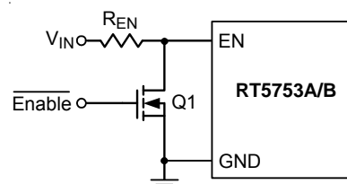
Figure 7. Logic Control for the EN Pin
