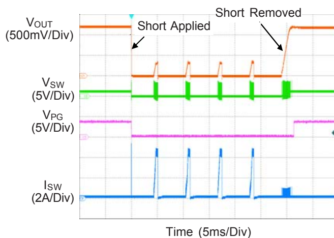
Figure 3. Short-Circuit Protection and Recovery
