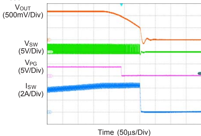
Figure 2. Over-Current Protection
