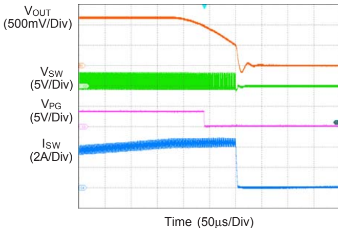
Figure 2. Over-Current Protection
