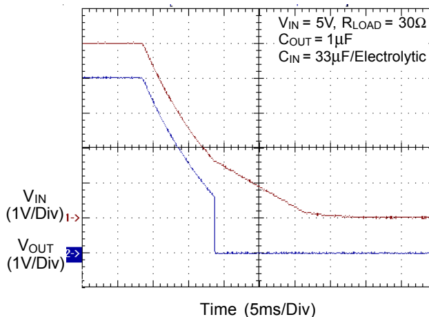
UVLO at Falling
