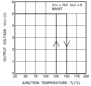
Fig. 8 Thermal cutoff circuit characteristics (BA05T)
