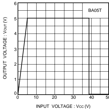
Fig. 10 Over voltage protection characteristics (BA05T)
