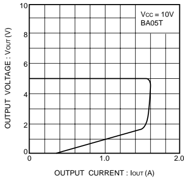
Fig. 9 Current limit characteristics (BA05T)
