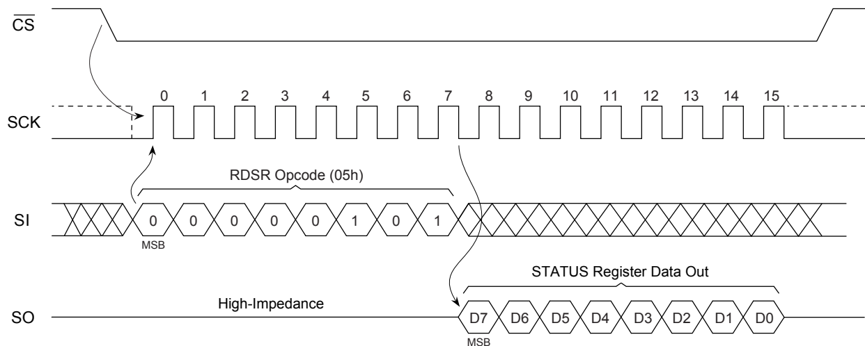
Figure 6-1. RDSR Waveform
