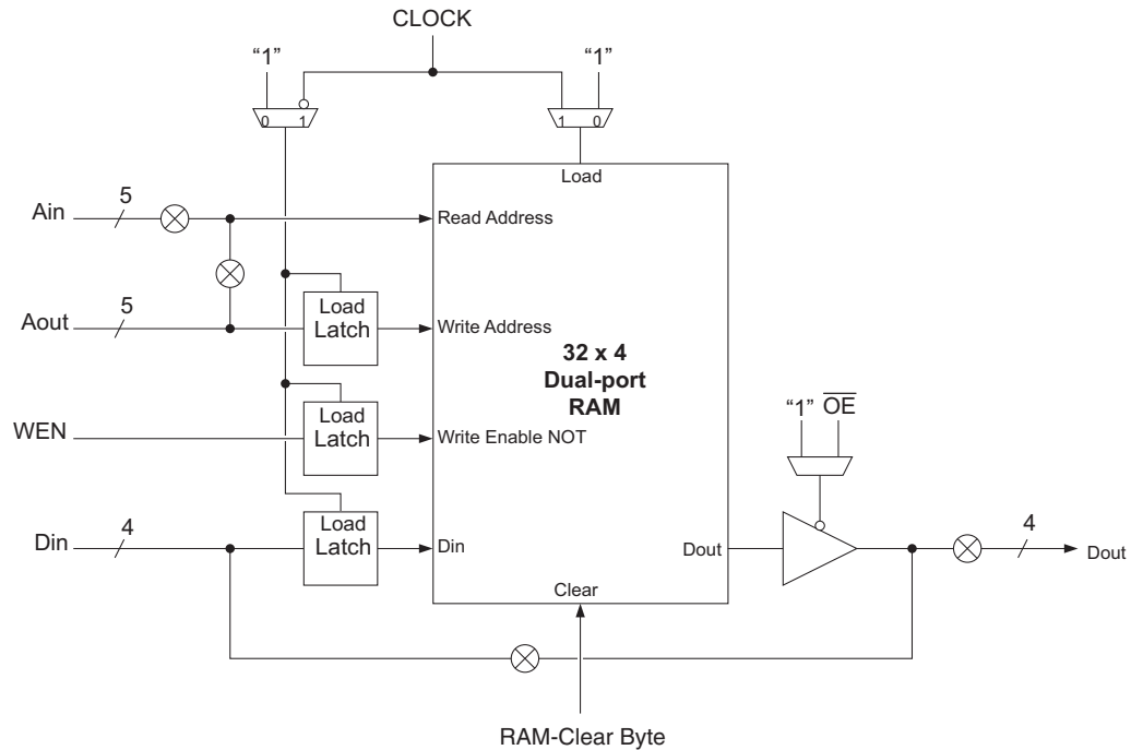
Figure 6-2. RAM Logic
