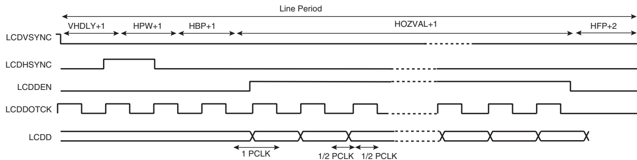
Figure 38-7. TFT Panel Timing (Line Expanded View), CLKMOD = 1
