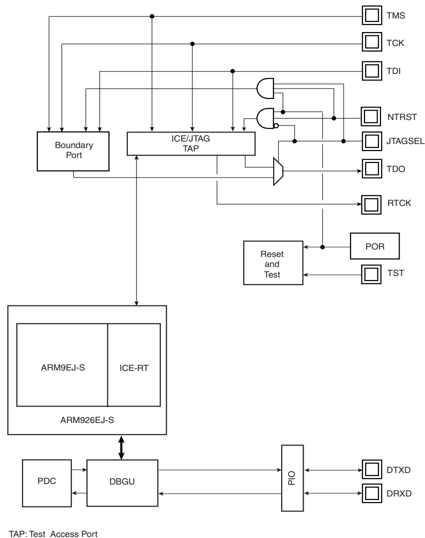
Figure 12-1. Debug and Test Block Diagram
