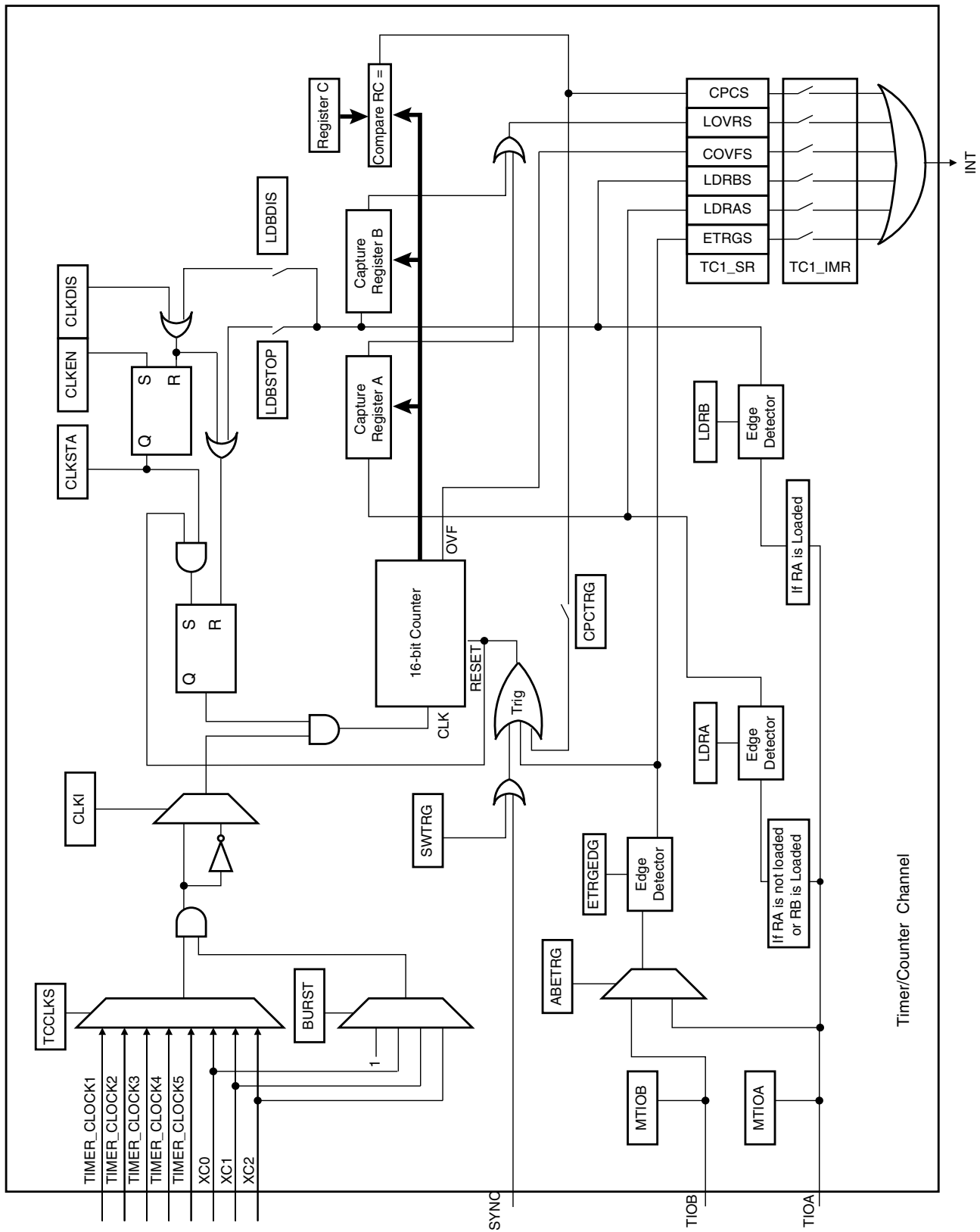
Figure 34-5. Capture Mode
