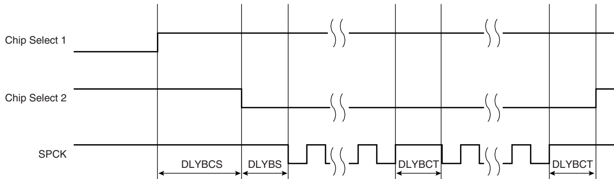
Figure 30-9. Programmable Delays
