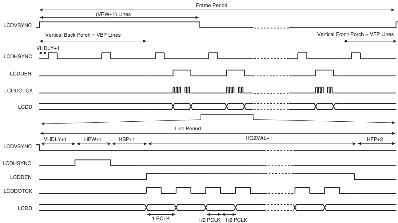
Figure 38-6. TFT Panel Timing, CLKMOD = 0, VPW = 2, VBP = 2, VFP = 1
