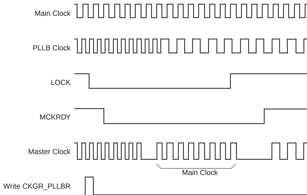
Figure 25-6: Change PLLB Programming
