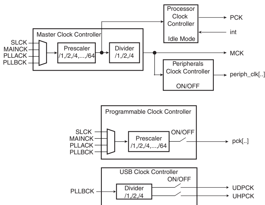
Figure 28-1. AT91SAM9XE128/256/512 Power Management Controller Block Diagram
