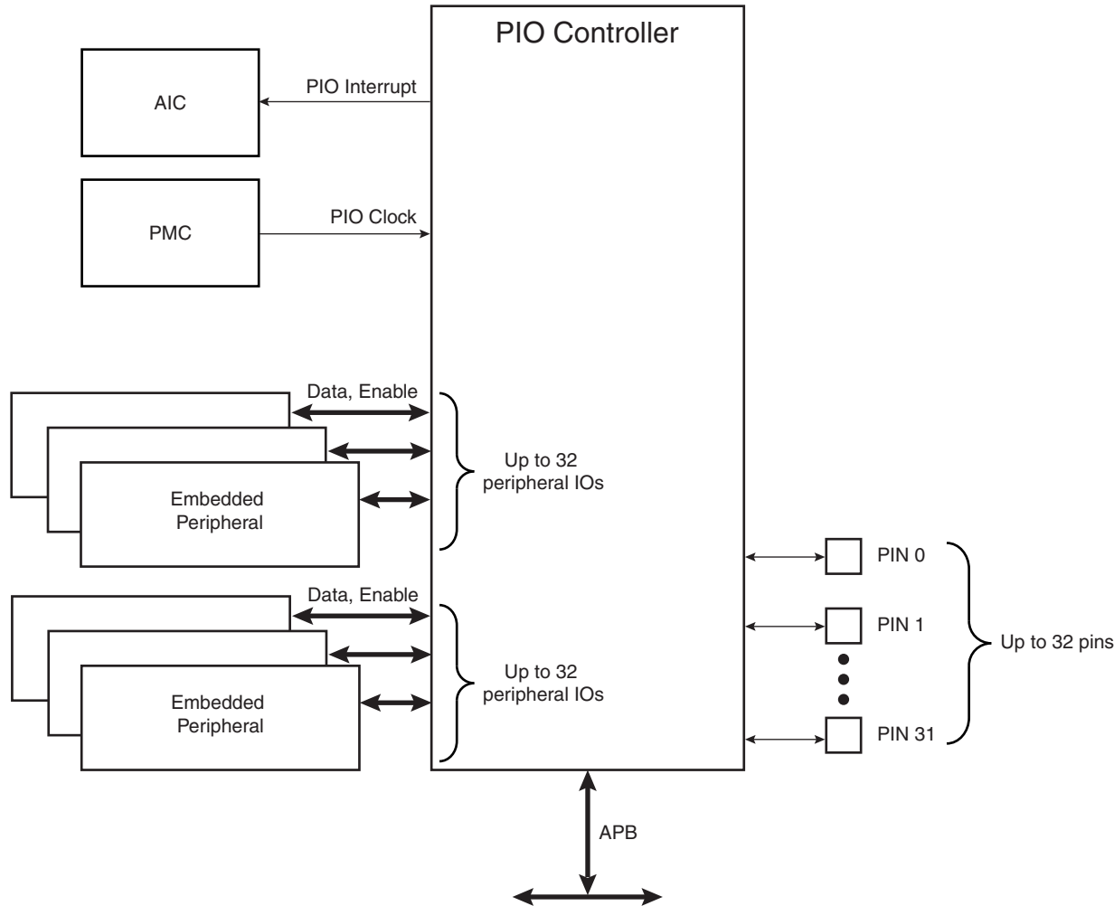
Figure 31-1. Block Diagram
