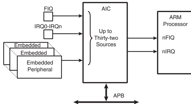
Figure 29-1. Block Diagram
