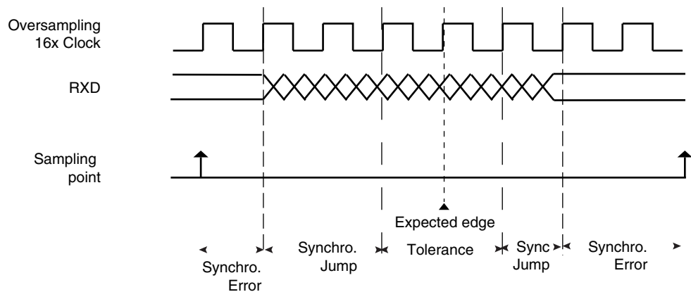
Figure 34-11. Bit Resynchronization
