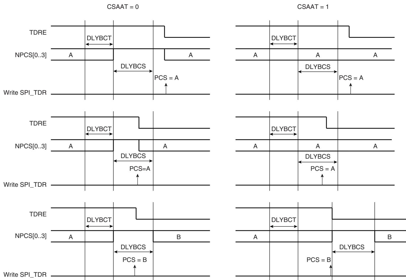
Figure 32-8. Peripheral Deselection
