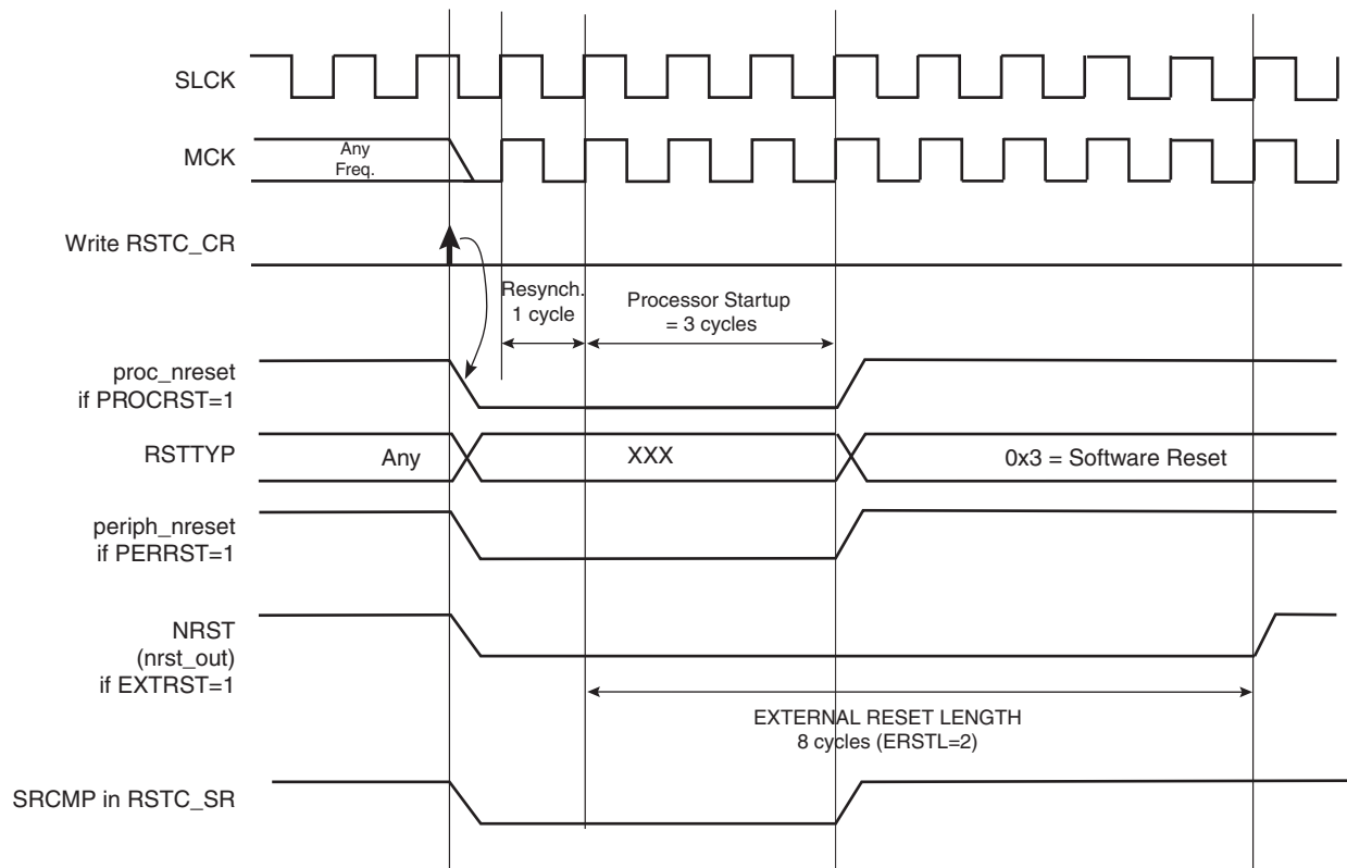
Figure 15-8. Software Reset
