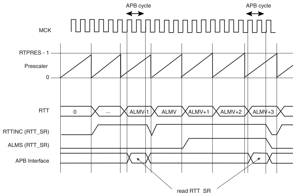
Figure 16-2. RTT Counting
