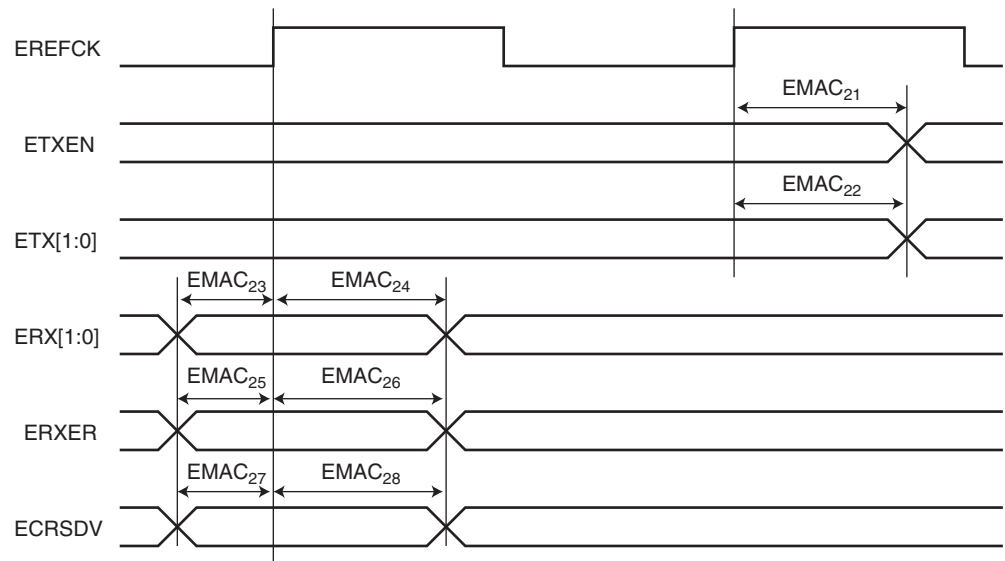
Figure 43-5. EMAC RMII Mode
