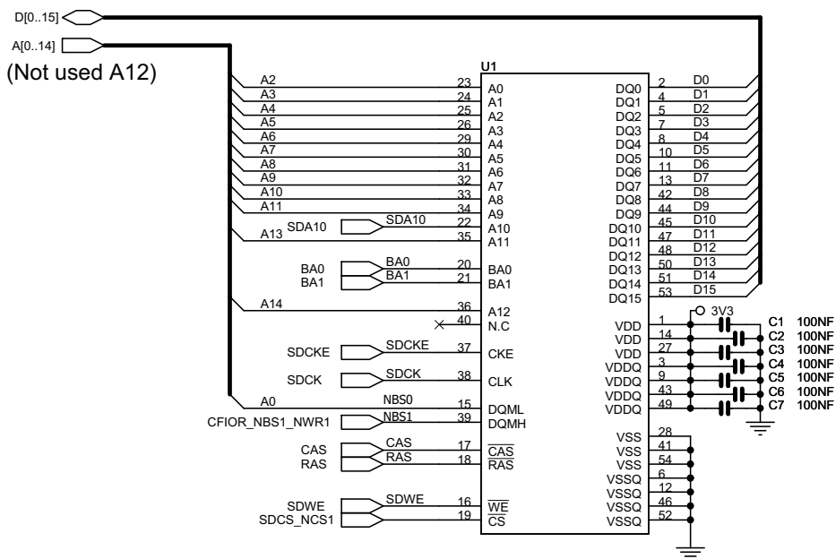
Figure 22-8. Hardware Configuration
