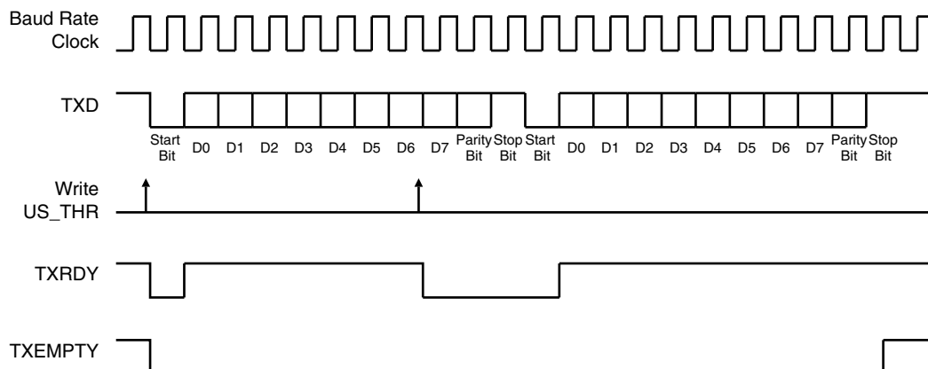
Figure 34-7. Transmitter Status
