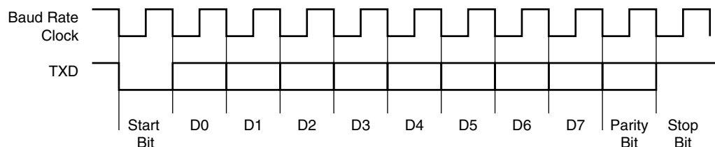
Figure 34-6. Character Transmit
