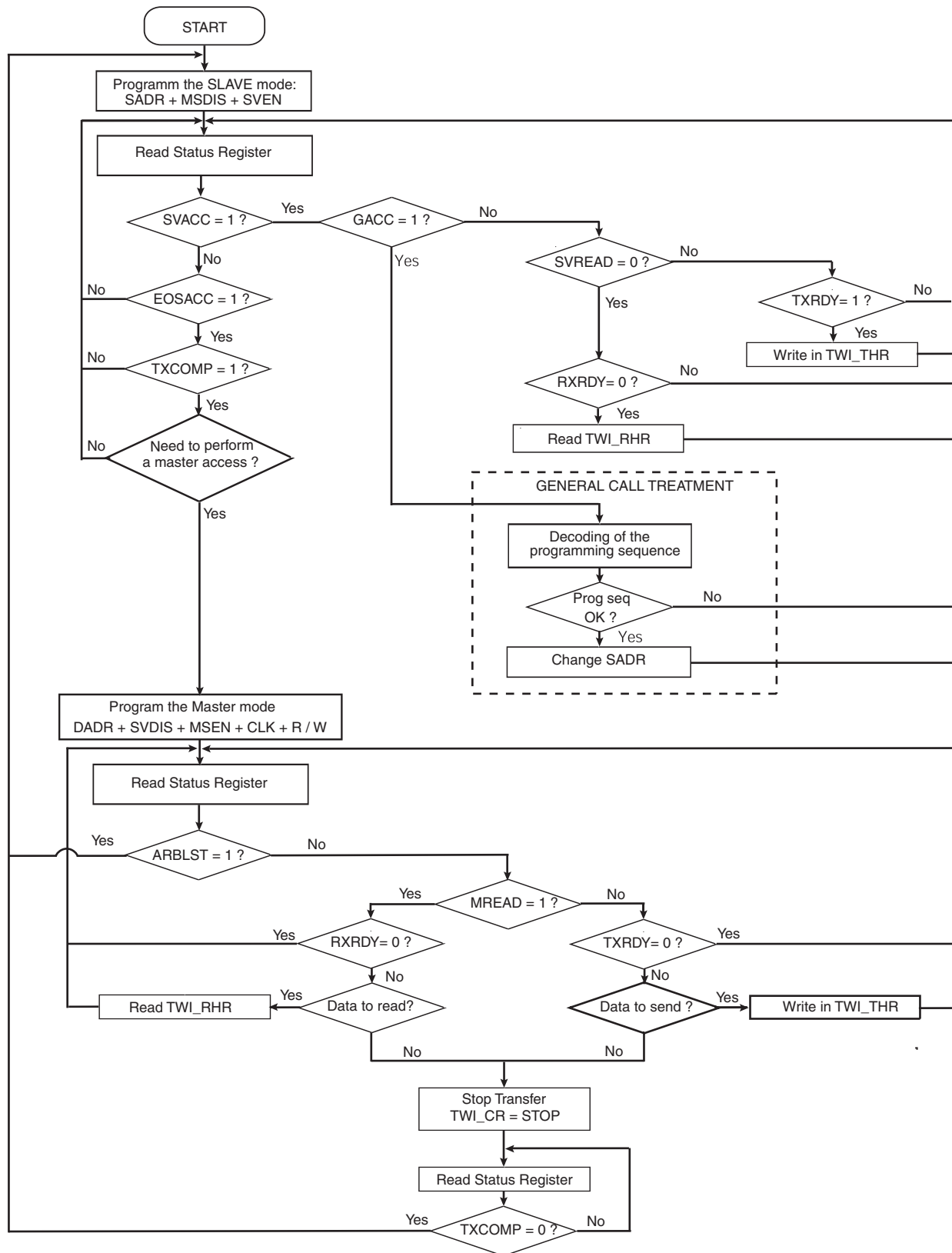
Figure 33-23. Multi-master Flowchart
