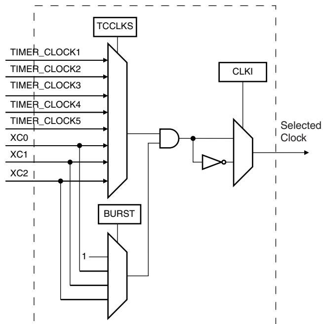
Figure 36-3. Clock Selection
