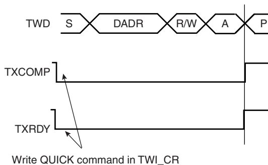
Figure 33-14. SMBUS Quick Command
