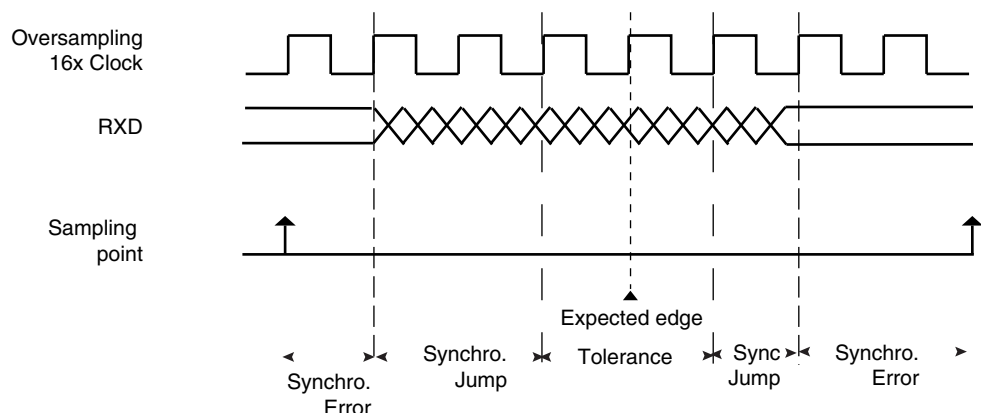
Figure 34-11. Bit Resynchronization
