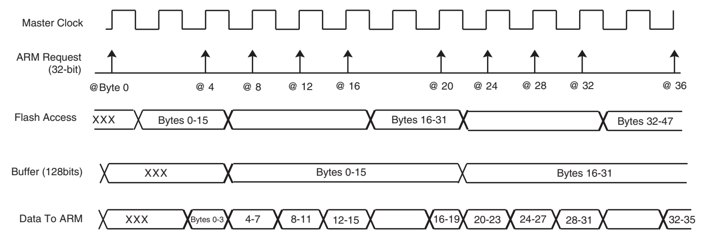
Figure 20-5. Data Read Optimization in ARM Mode for FWS = 1
