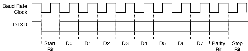
Figure 30-10. Character Transmission
