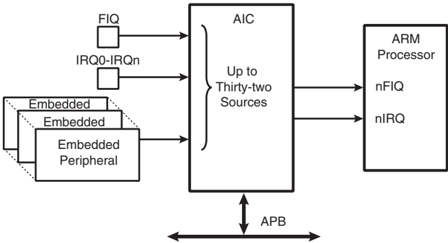
Figure 29-1. Block Diagram
