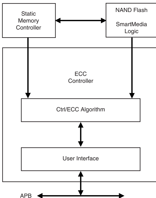
Figure 25-1. Block Diagram
