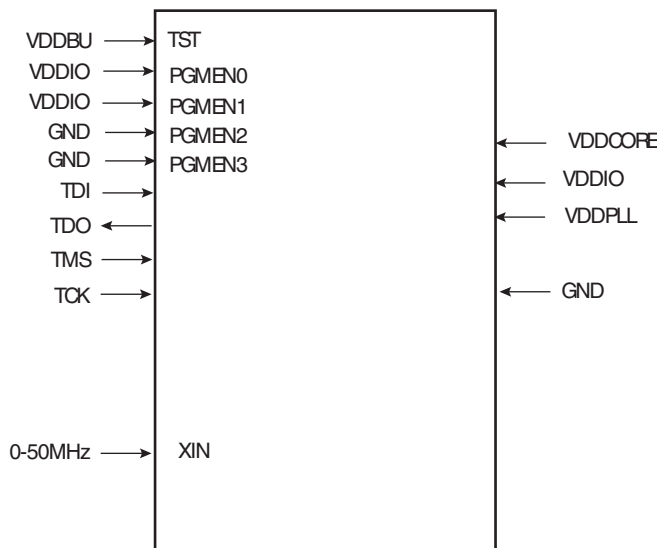
Figure 14-4. Serial Programming
