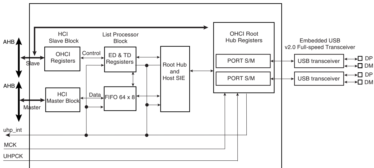
Figure 40-1. Block Diagram
