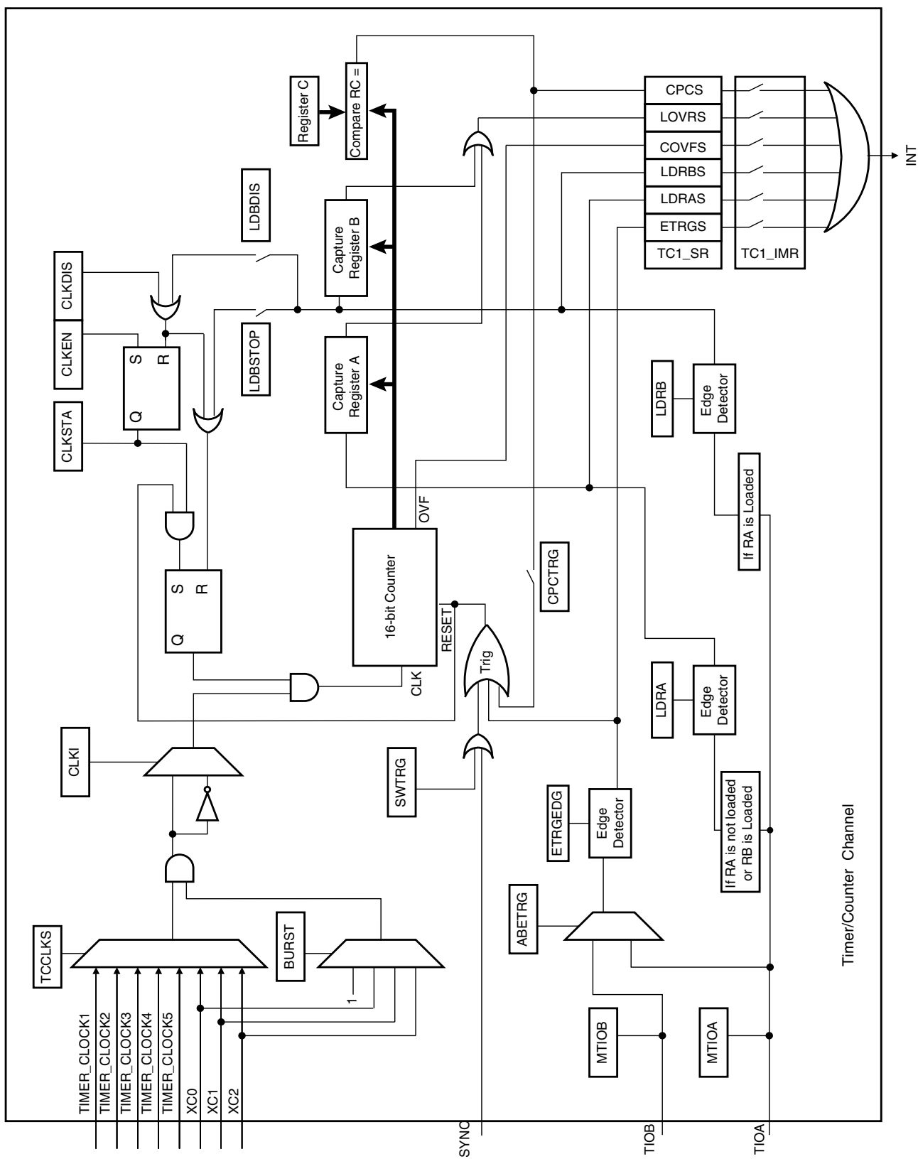
Figure 36-5. Capture Mode
