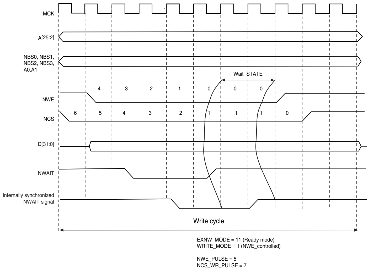
Figure 23-28. NWAIT Assertion in Write Access: Ready Mode ( \text{EXNW\_MODE} = 11 )
