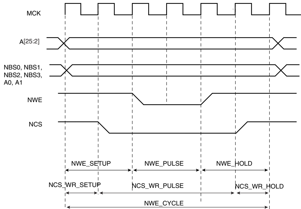
Figure 23-12. Write Cycle
