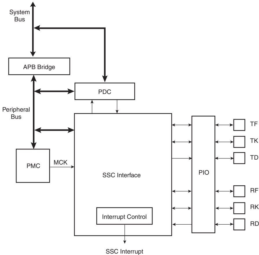
Figure 35-1. Block Diagram
