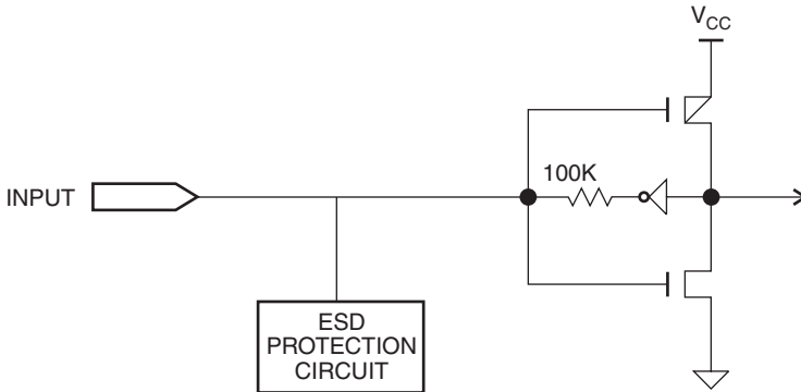
Figure 8-1. Input Diagram
