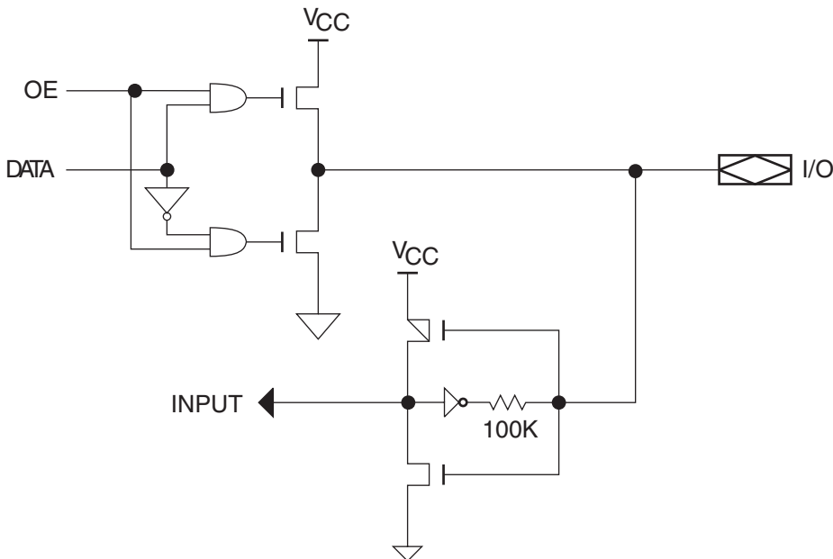
Figure 8-2. I/O Diagram
