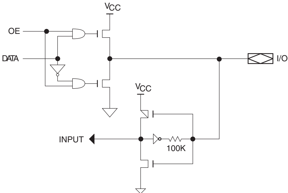
Figure 8-2. I/O Diagram
