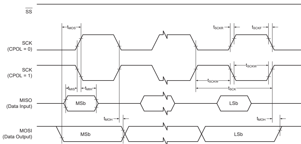
Figure 32-8. SPI - Timing Requirements in Client Mode
