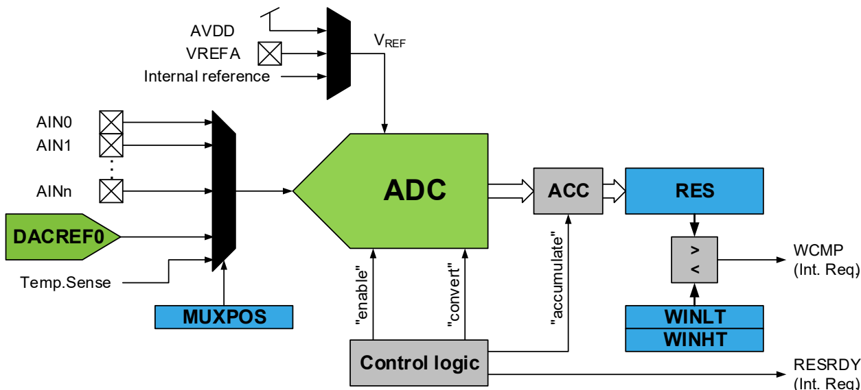
Figure 29-1. Block Diagram
