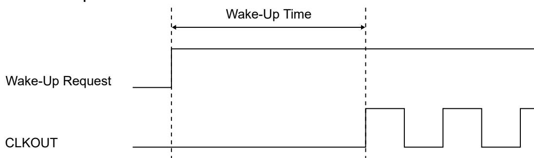
Figure 32-4. Wake-Up Time Definition
