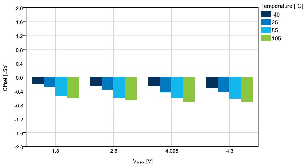
Figure 33-63. Offset vs. V_{REF} ( V_{DD} = 5.0V , f_{ADC} = 115 kps, REFSEL = External Reference)
