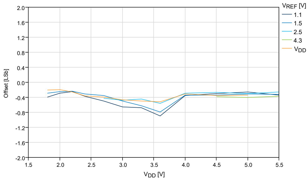
Figure 33-52. Offset Error vs. V_{DD} ( f_{ADC} = 115 kps) at T = 25^{\circ}C , REFSEL = Internal Reference
