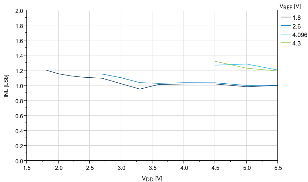
Figure 33-60. INL vs. V_{DD} ( f_{ADC} = 115 kps, T = 25^{\circ}C , REFSEL = External Reference)
