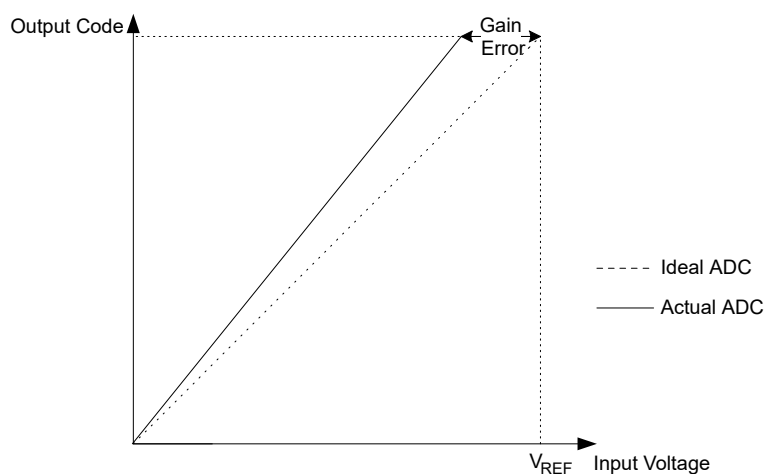
Figure 5-2. Gain Error
