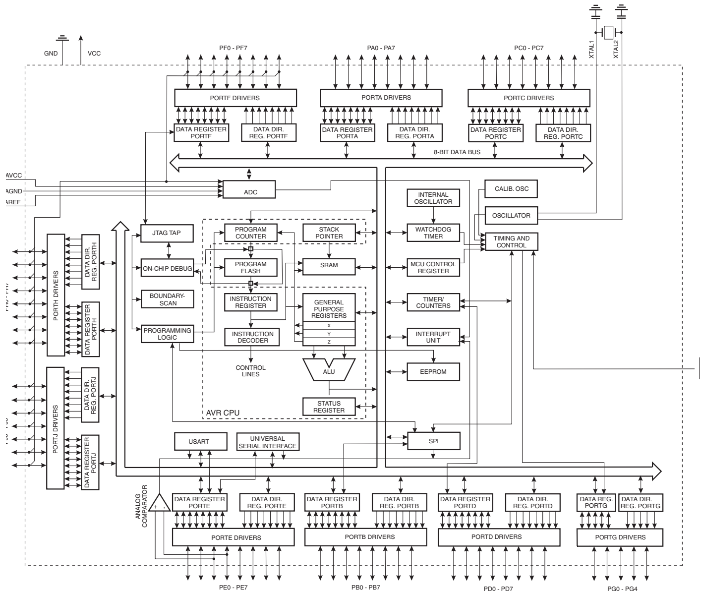
Figure 2-1. Block diagram.
