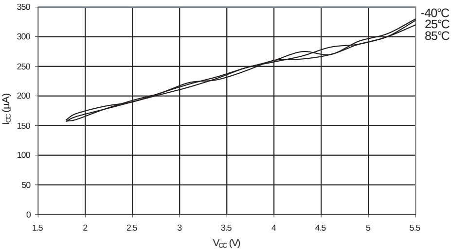
Figure 32-41. ADC Current vs. V_{CC} ( A_{REF} = A_{V_{CC}} )
