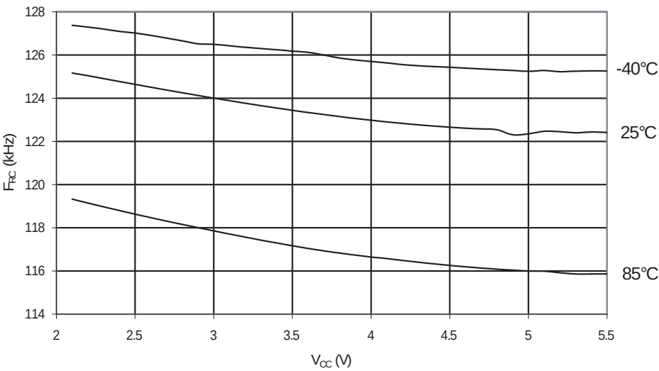
Figure 32-35. Watchdog Oscillator Frequency vs. V_{CC}
