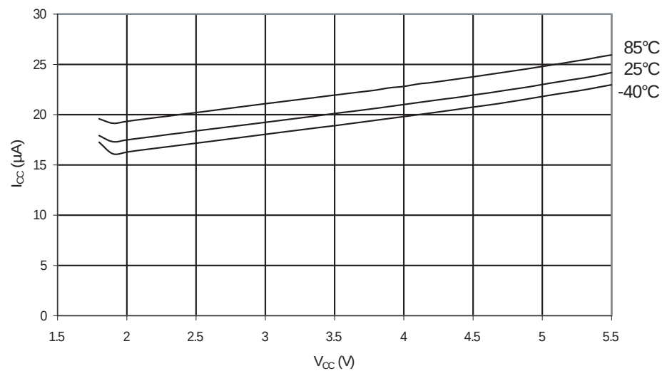
Figure 32-40. Brownout Detector Current vs. V_{CC}
