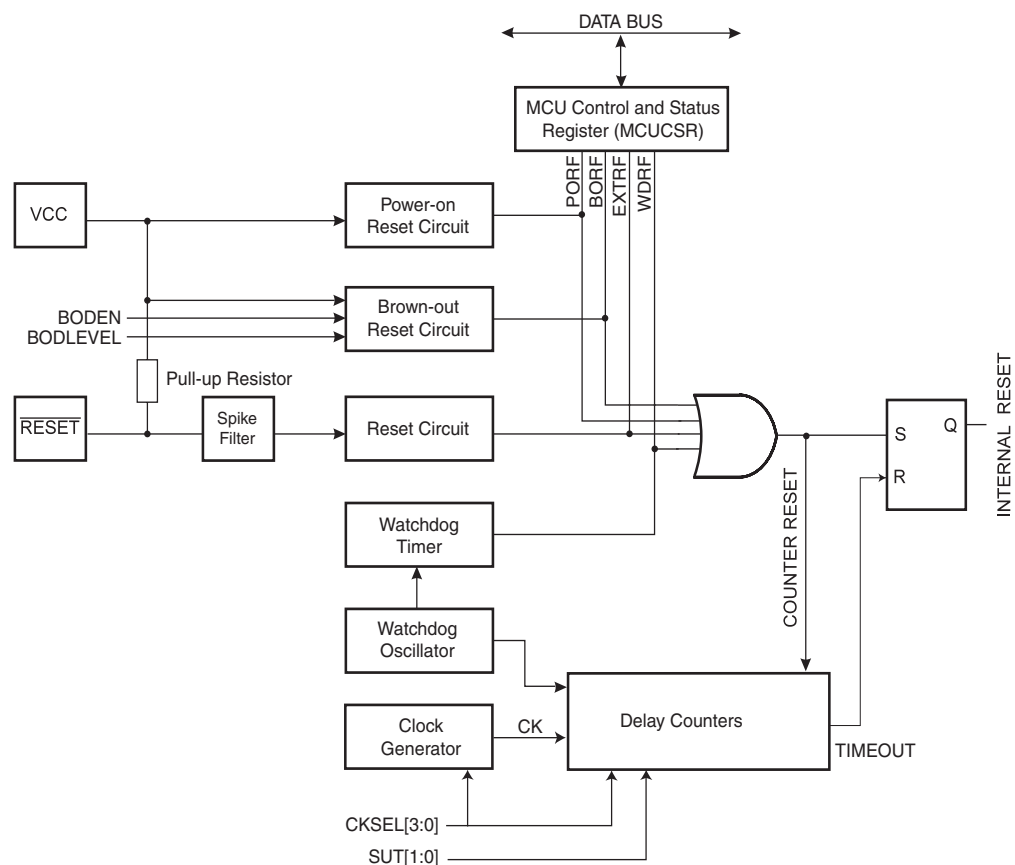
Figure 15. Reset Logic
