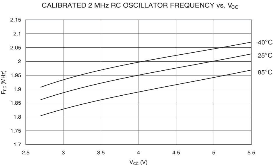
Figure 182. Calibrated 2 MHz RC Oscillator Frequency vs. V_{CC}
