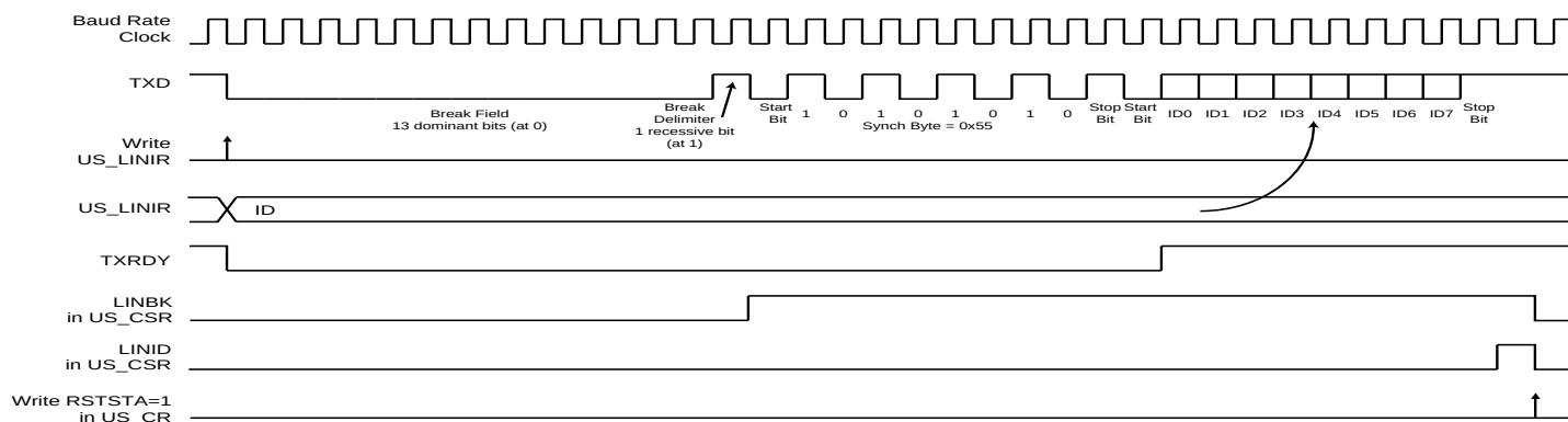
Figure 35-40. Header Transmission
