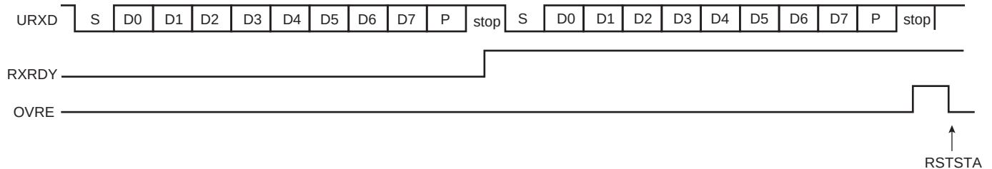
Figure 34-6. Receiver Overrun
