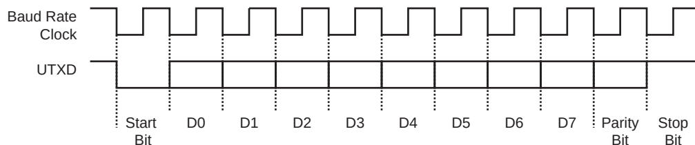
Figure 34-9. Character Transmission
