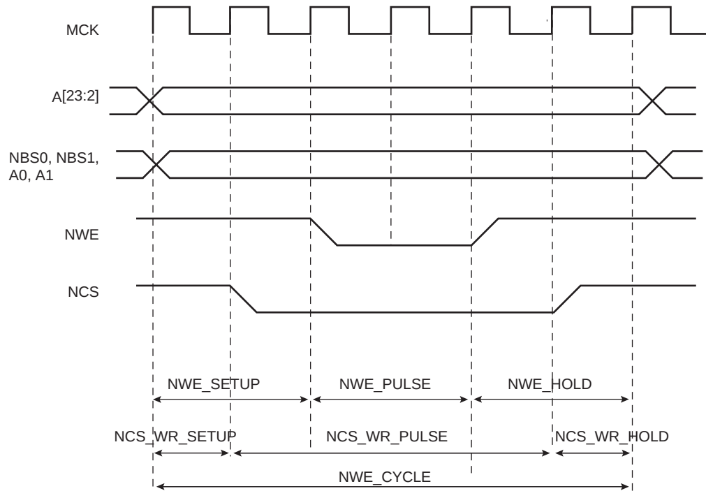
Figure 25-10. Write Cycle
