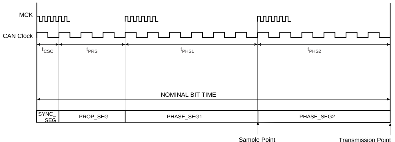
Figure 40-5. CAN Bit Timing
