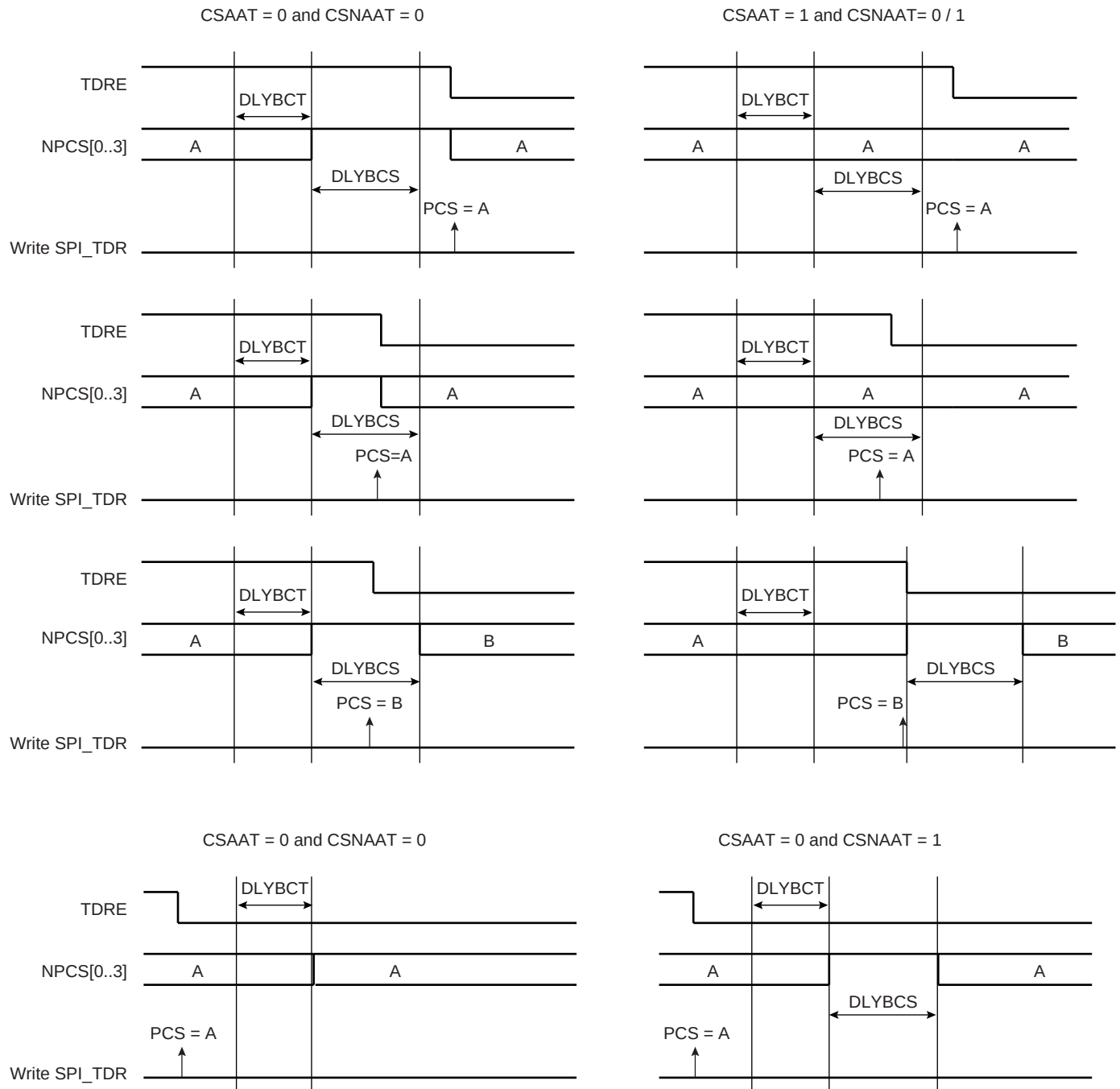
Figure 32-10. Peripheral Deselection
