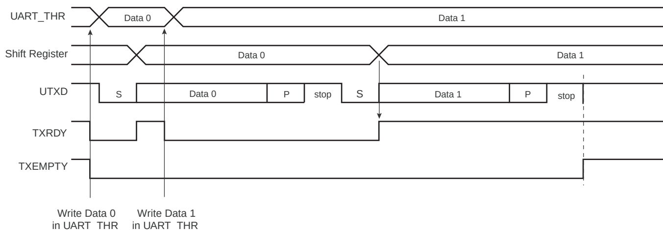
Figure 34-10. Transmitter Control
