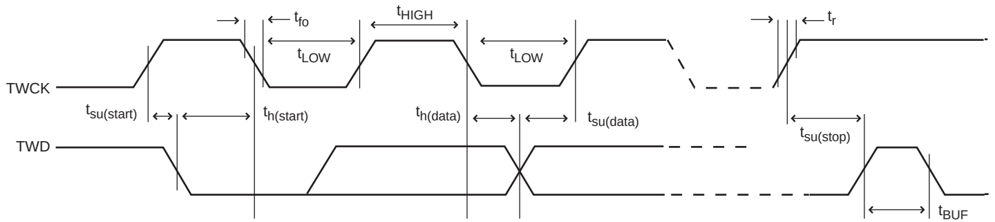
Figure 45-40. Two-wire Serial Bus Timing
