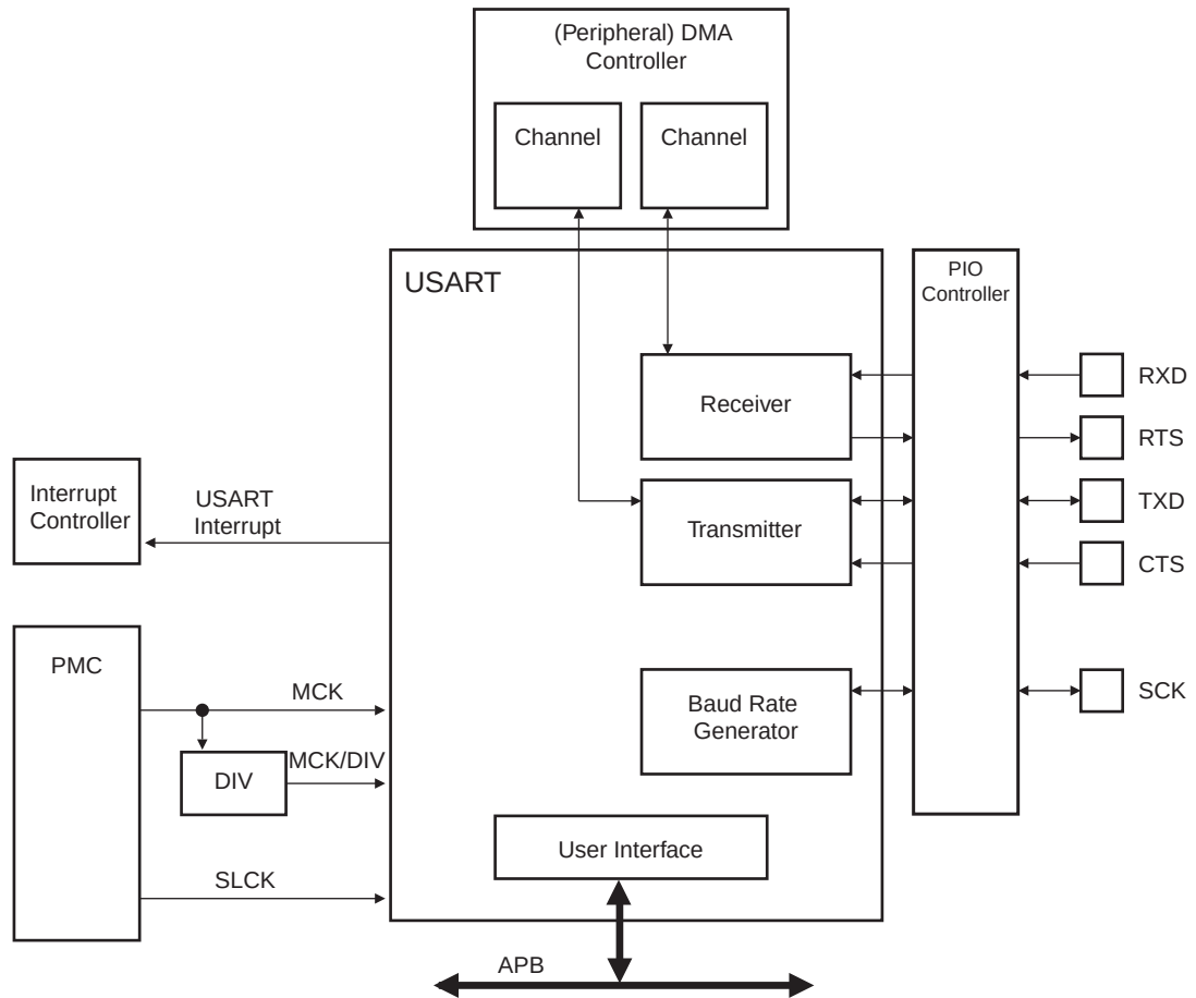
Figure 35-1. USART Block Diagram
