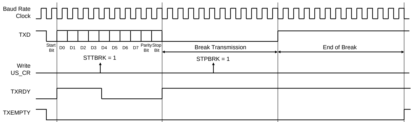
Figure 35-26. Break Transmission
