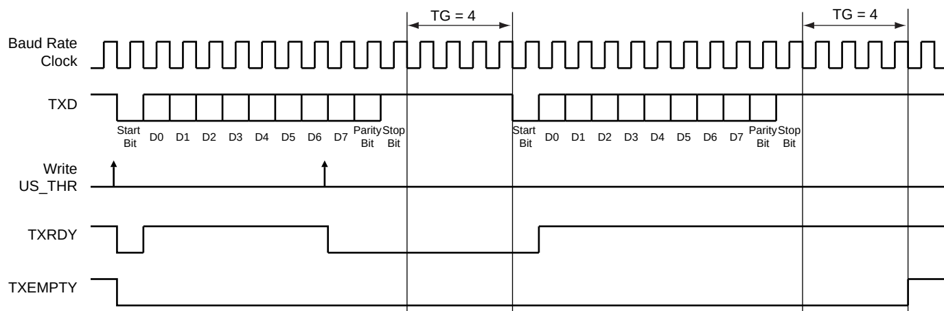
Figure 35-23. Timeguard Operations
