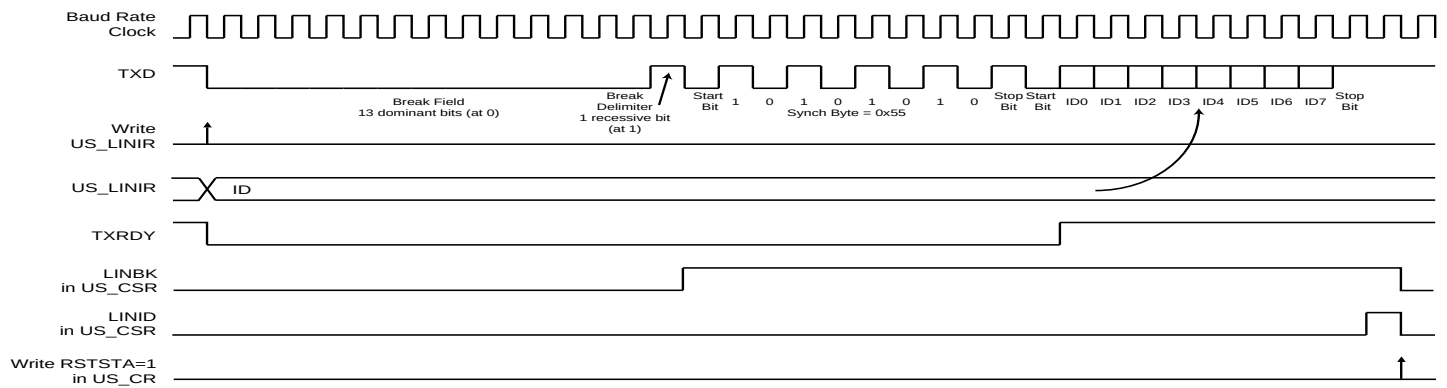
Figure 35-40. Header Transmission
