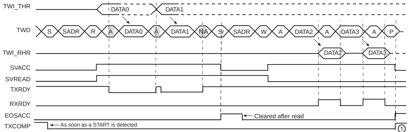
Figure 33-30. Repeated Start + Reversal from Read to Write Mode
