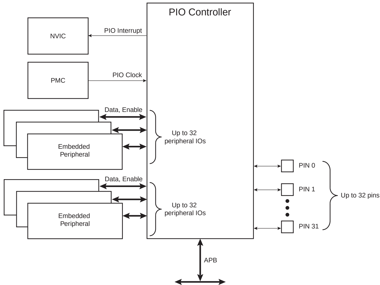
Figure 31-1. Block Diagram
