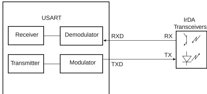
Figure 35-33. Connection to IrDA Transceivers
