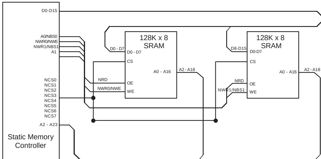
Figure 25-2. SMC Connections to Static Memory Devices
