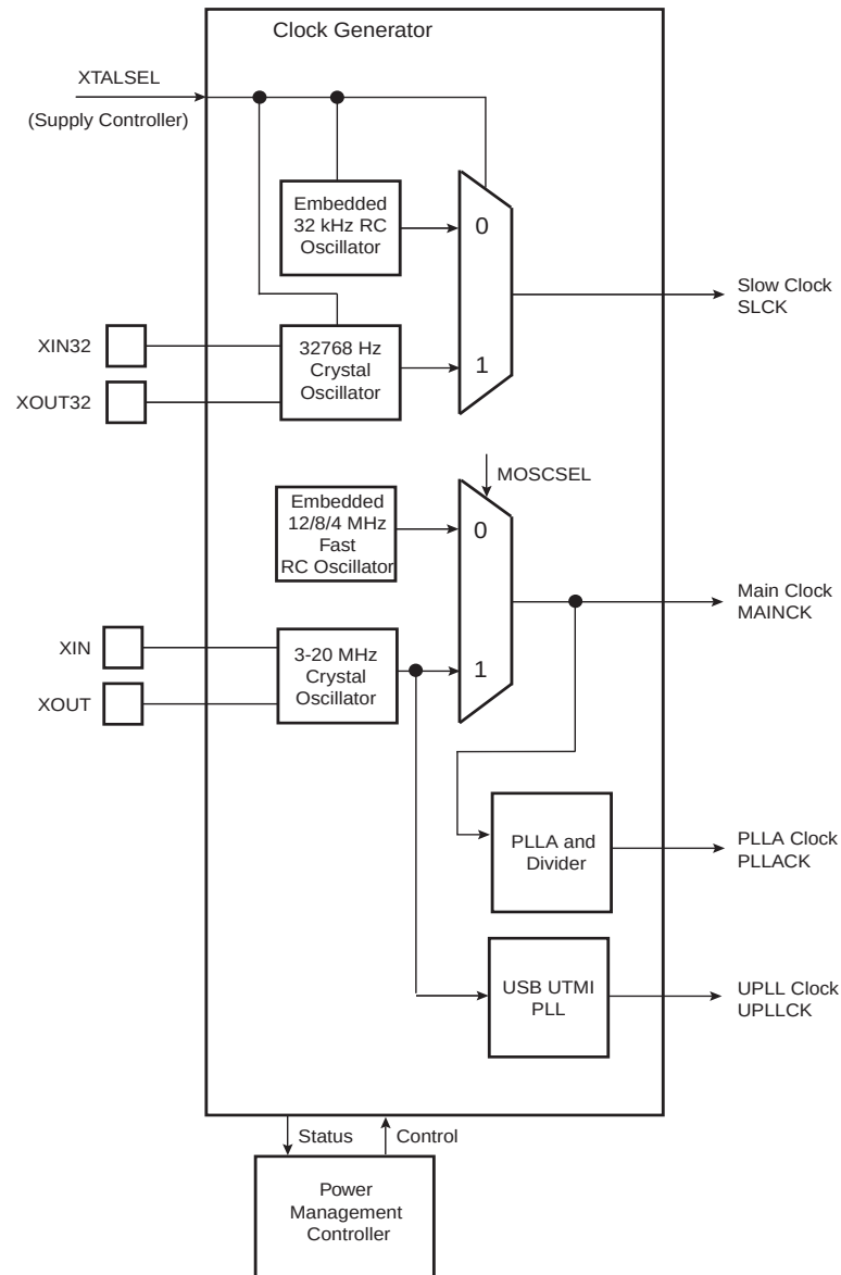
Figure 27-1. Clock Generator Block Diagram
