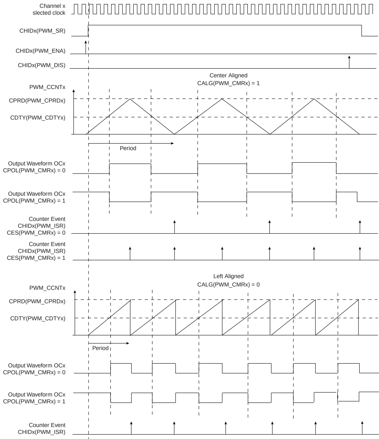
Figure 38-5. Waveform Properties
