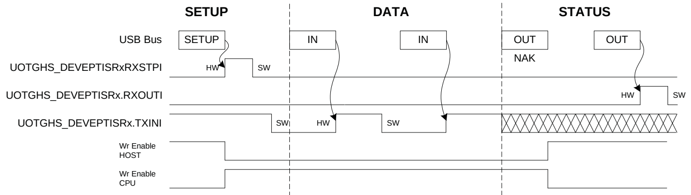
Figure 39-15. Control Read
