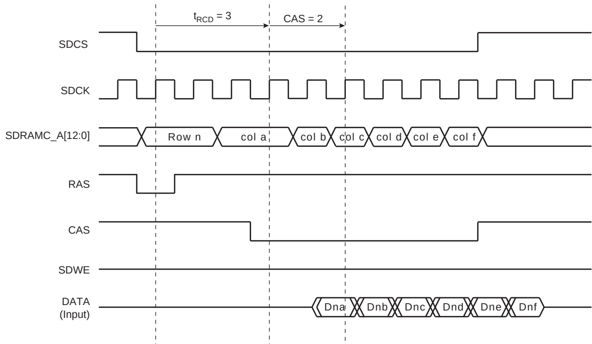
Figure 24-3. Read Burst SDRAM Access
