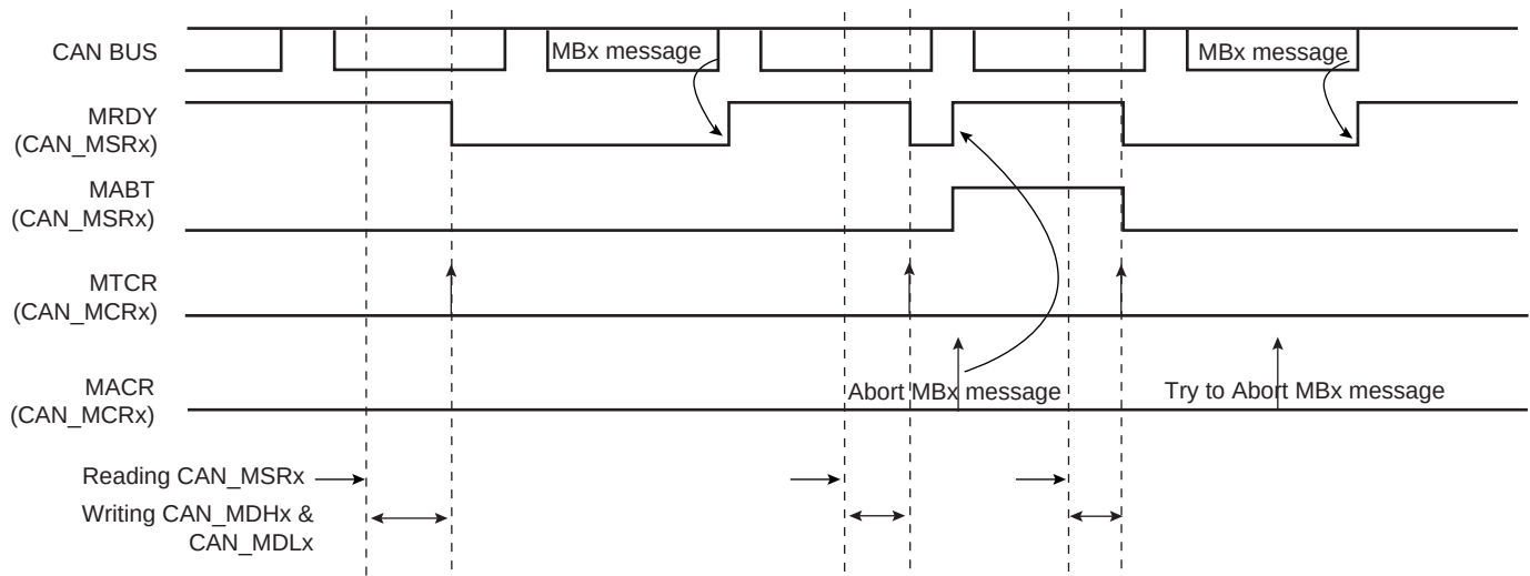
Figure 40-15. Transmitting Messages
