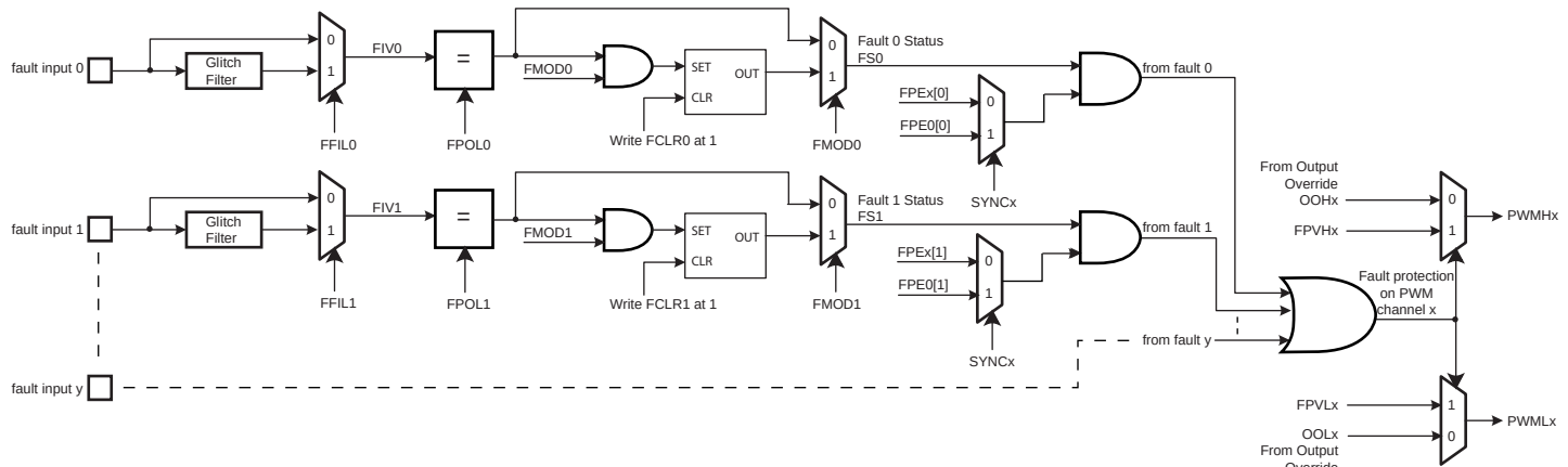
Figure 38-9. Fault Protection
