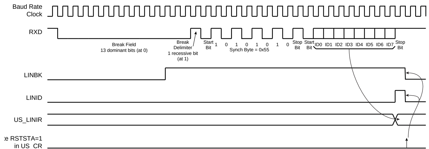
Figure 35-41. Header Reception
