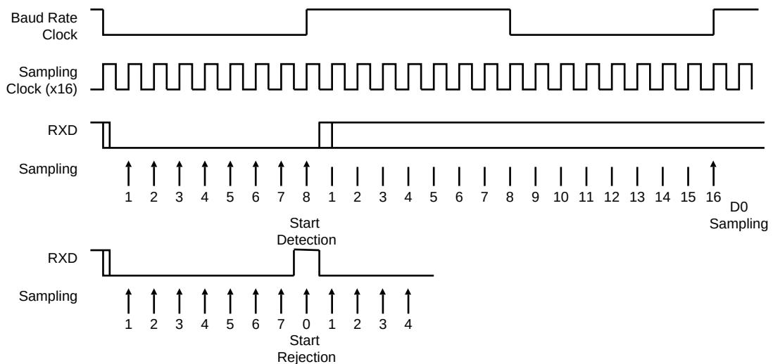
Figure 35-12. Asynchronous Start Detection
