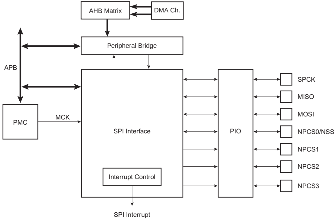
Figure 32-1. Block Diagram
