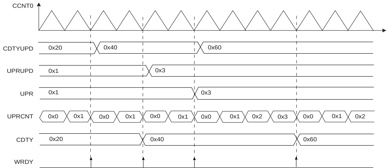
Figure 38-11. Method 2 (UPDM=1)
