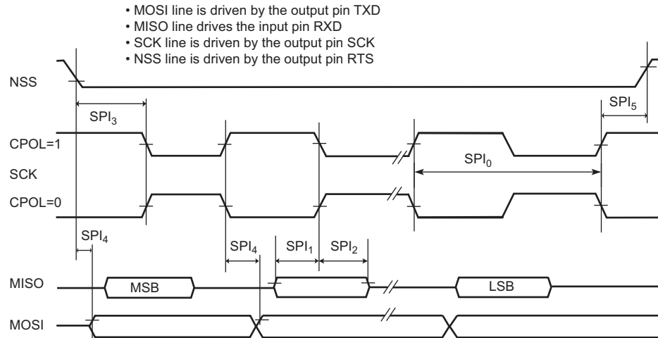
Figure 45-34. USART SPI Master Mode
