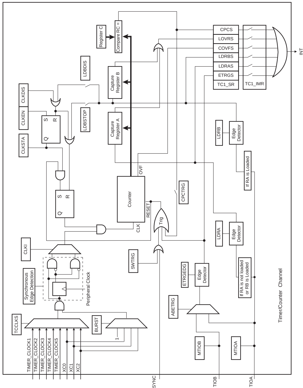
Figure 36-5. Capture Mode
