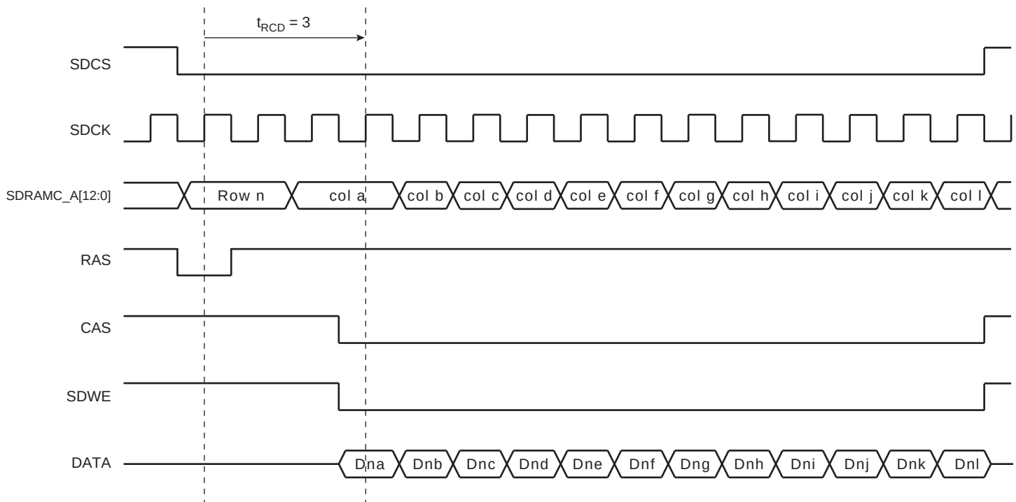
Figure 24-2. Write Burst SDRAM Access
