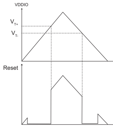
Figure 45-3. Zero-Power-on Reset Characteristics
