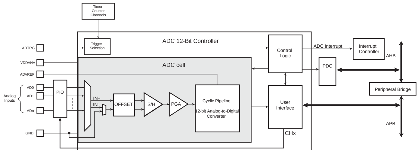
Figure 43-1. Analog-to-Digital Converter Block Diagram
