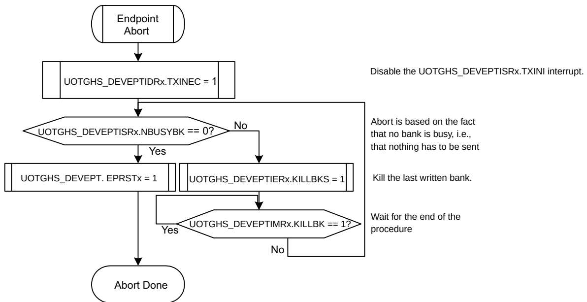
Figure 39-18. Abort Algorithm
