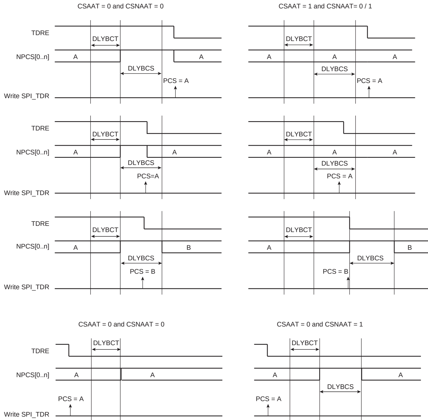
Figure 33-12. Peripheral Deselection
