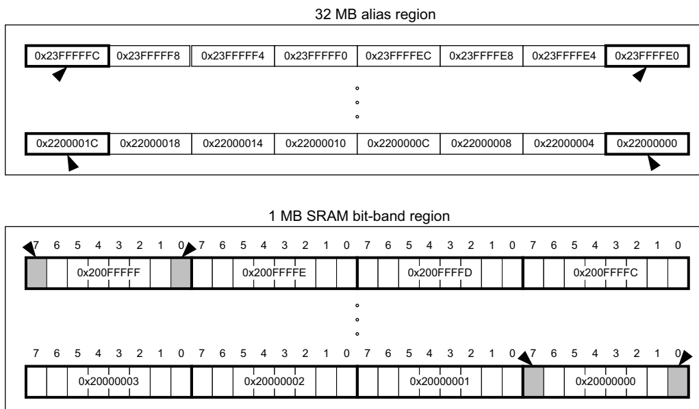
Figure 12-4. Bit-band Mapping
