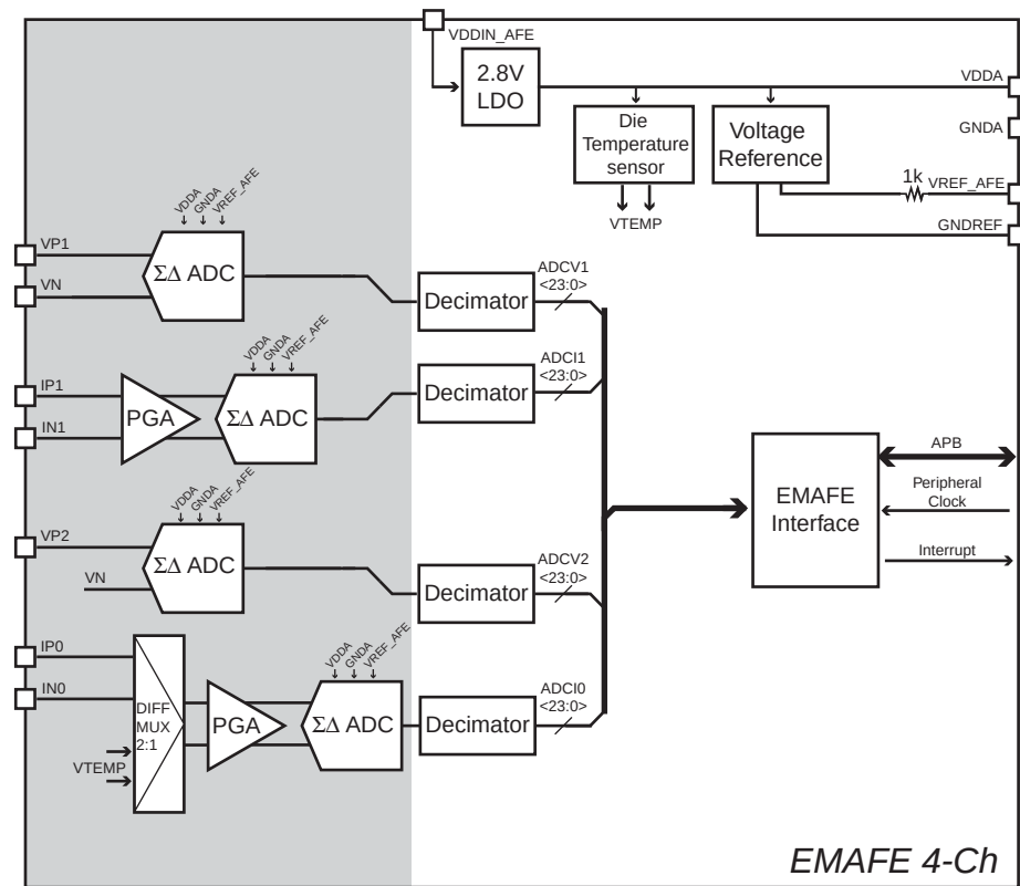
Figure 41-2. Functional Block Diagram for Two-Phase EMAFE
