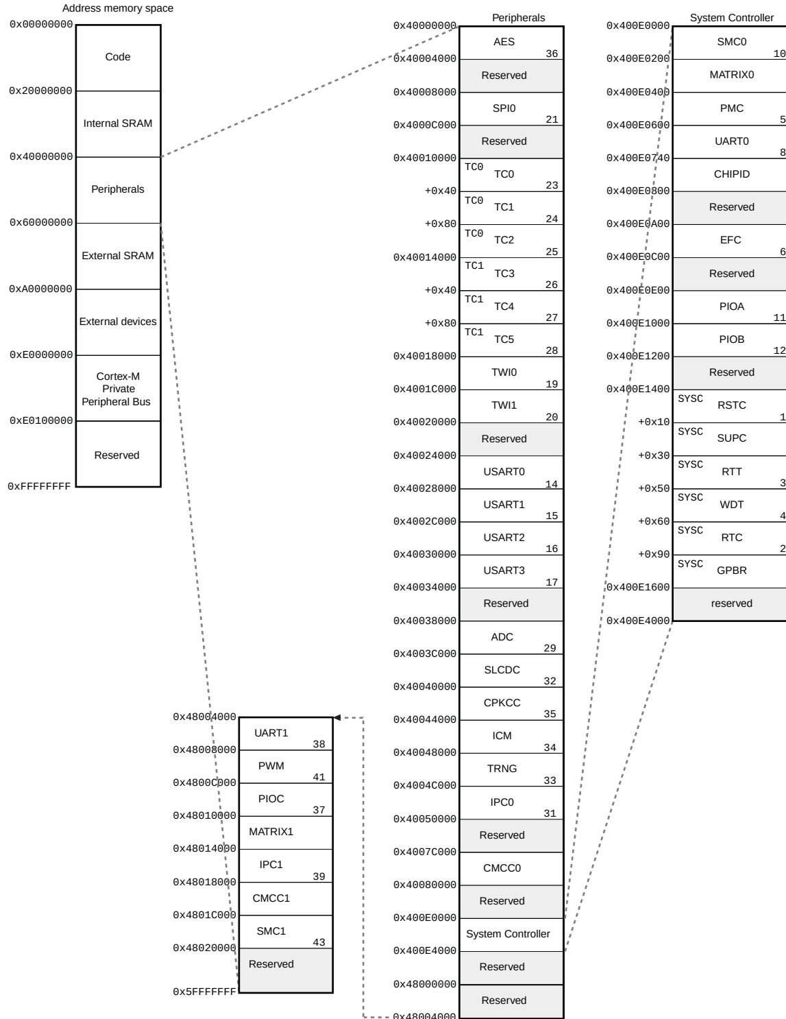
Figure 7-4. SAM4CM16/8/4 Memory Mapping of the Peripherals Area
