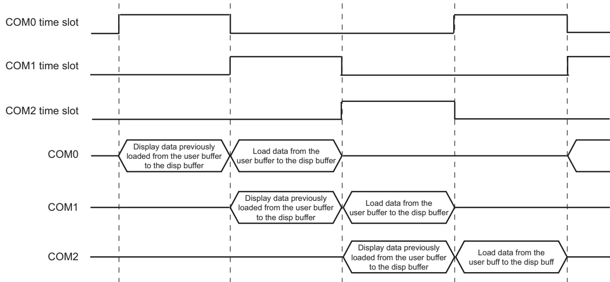
Figure 39-9. Memory Management
