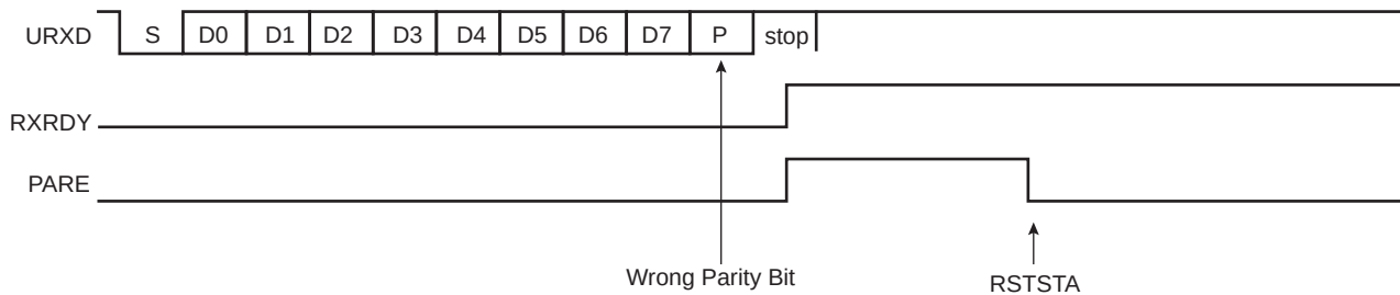
Figure 35-7. Parity Error
