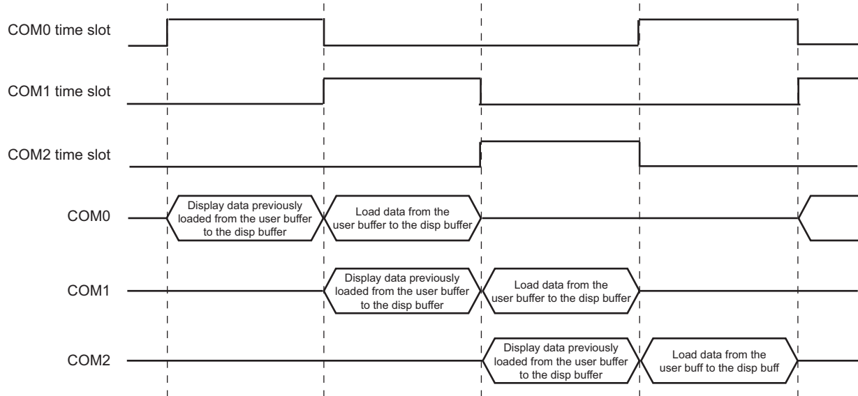
Figure 39-9. Memory Management
