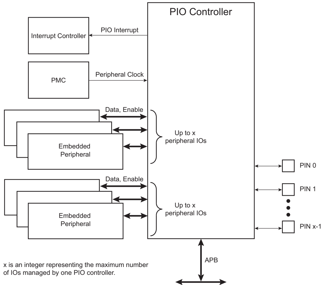
Figure 32-1. Block Diagram
