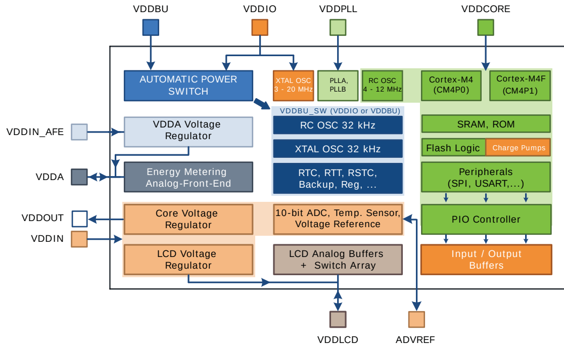
Figure 5-1. Power Domains
