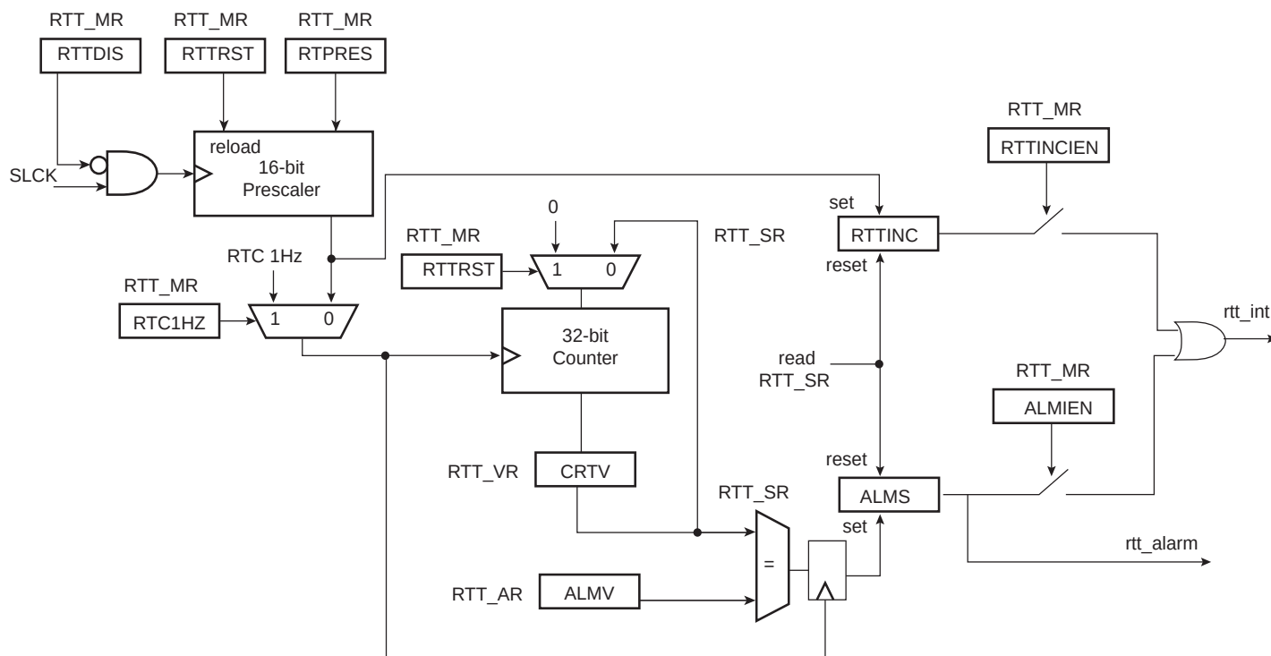
Figure 16-1. Real-time Timer
