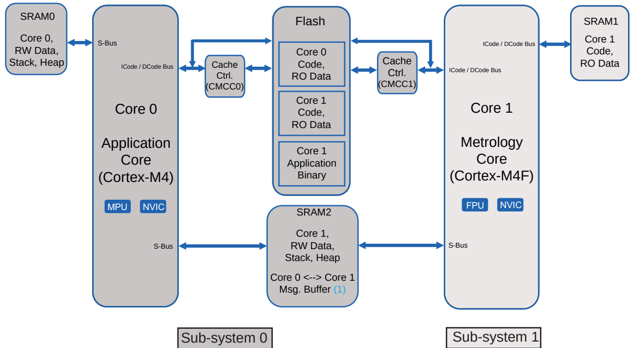
Figure 8-6. Execution View
