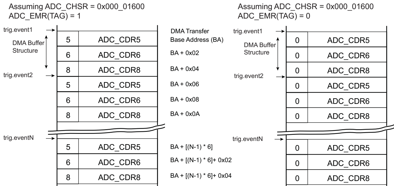
Figure 40-12. Buffer Structure
