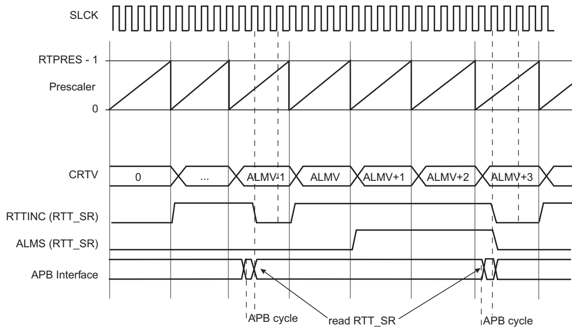
Figure 16-2. RTT Counting
