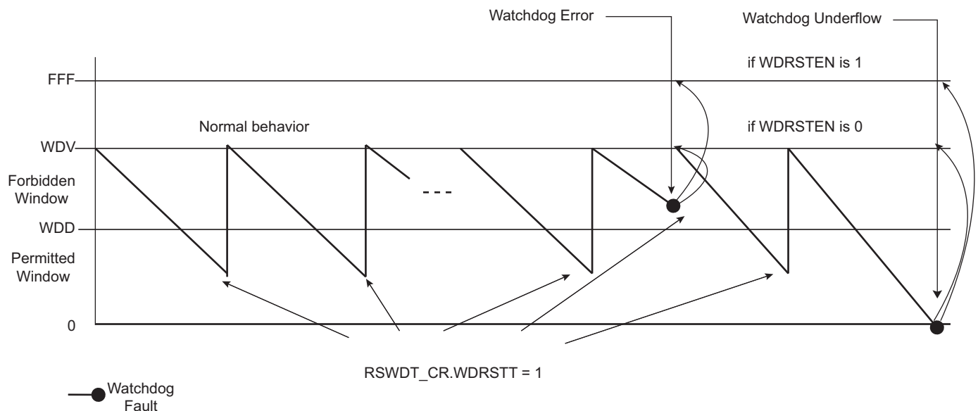
Figure 19-2. Watchdog Behavior
