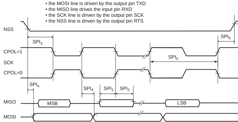
Figure 46-10. USART SPI Master Mode
