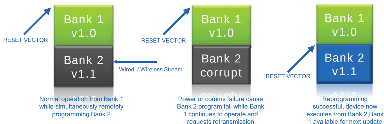
Figure 8-1. Dual Bank and Dual Boot Firmware Upgrade
