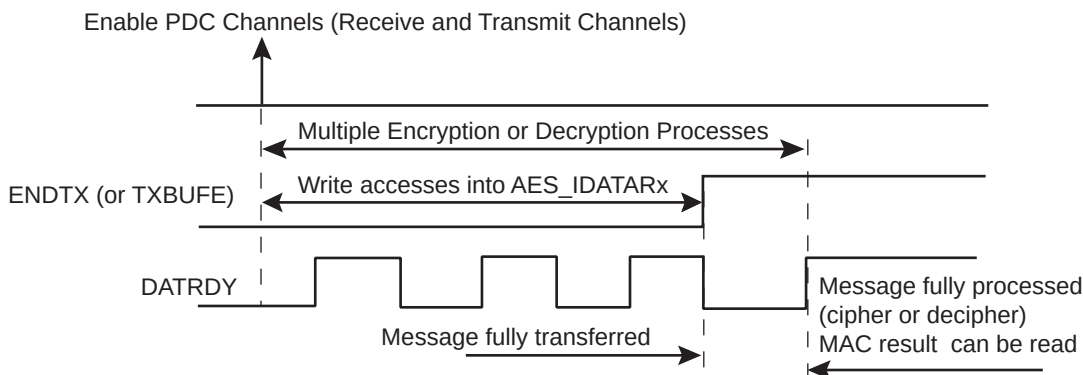
Figure 42-4. PDC Transfer with AES_MR.LOD = 1
