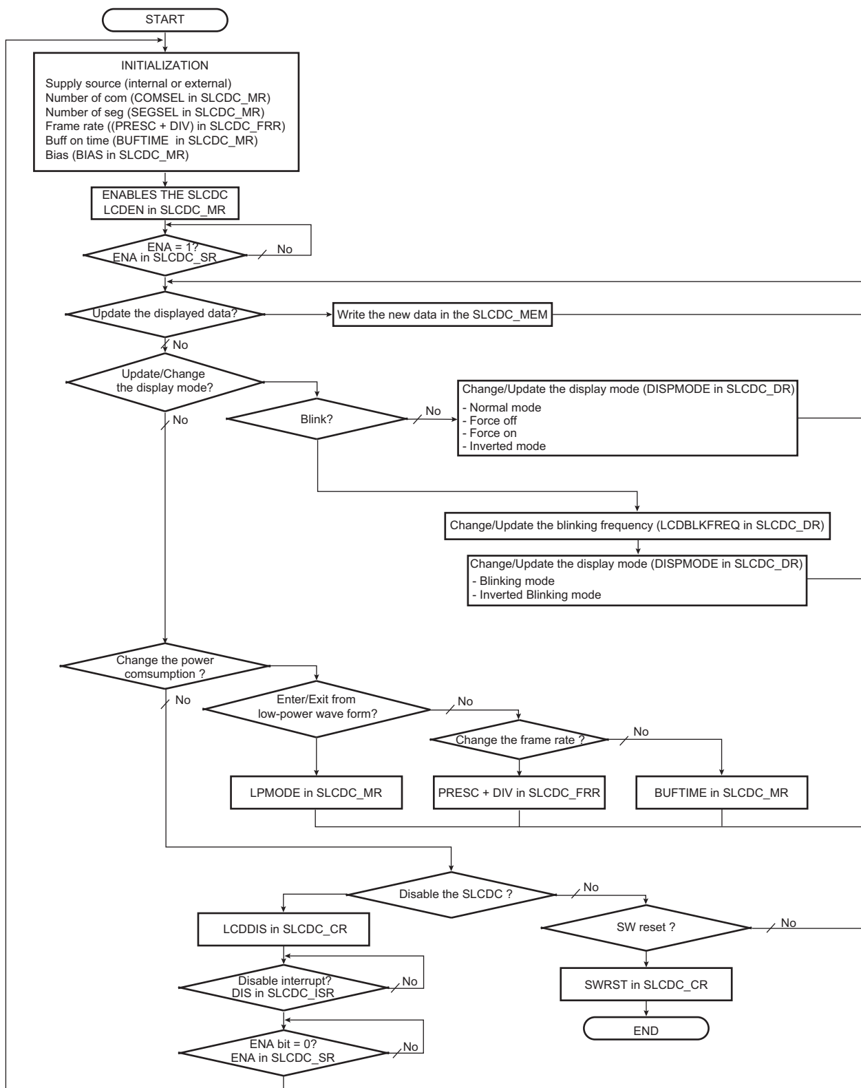
Figure 39-12. SLCD Flow Chart
