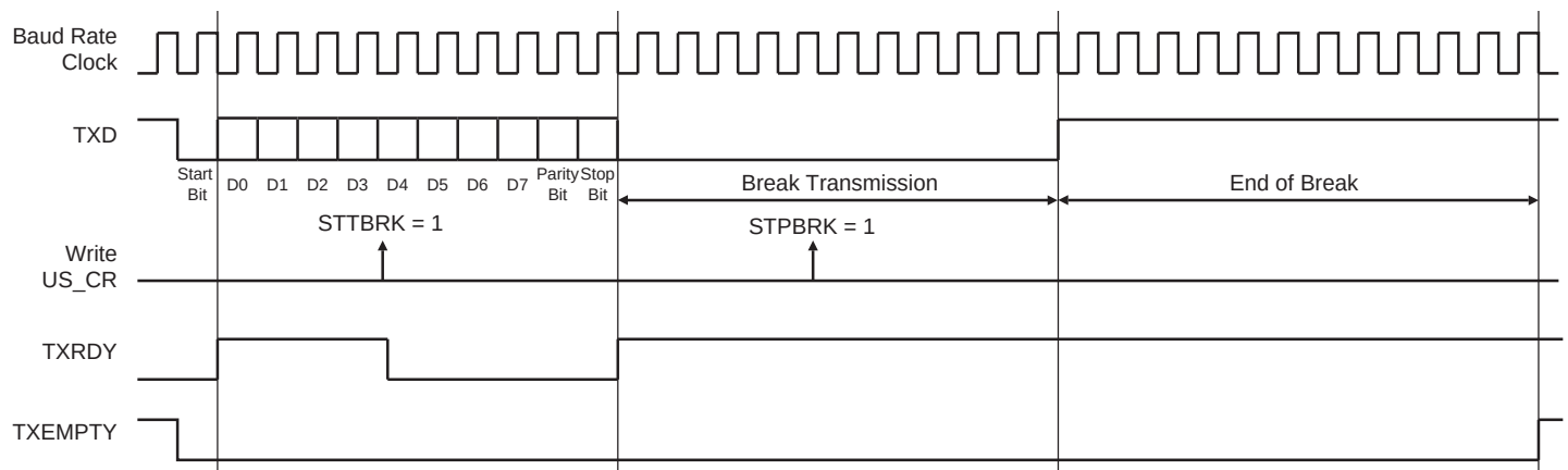
Figure 37-25. Break Transmission
