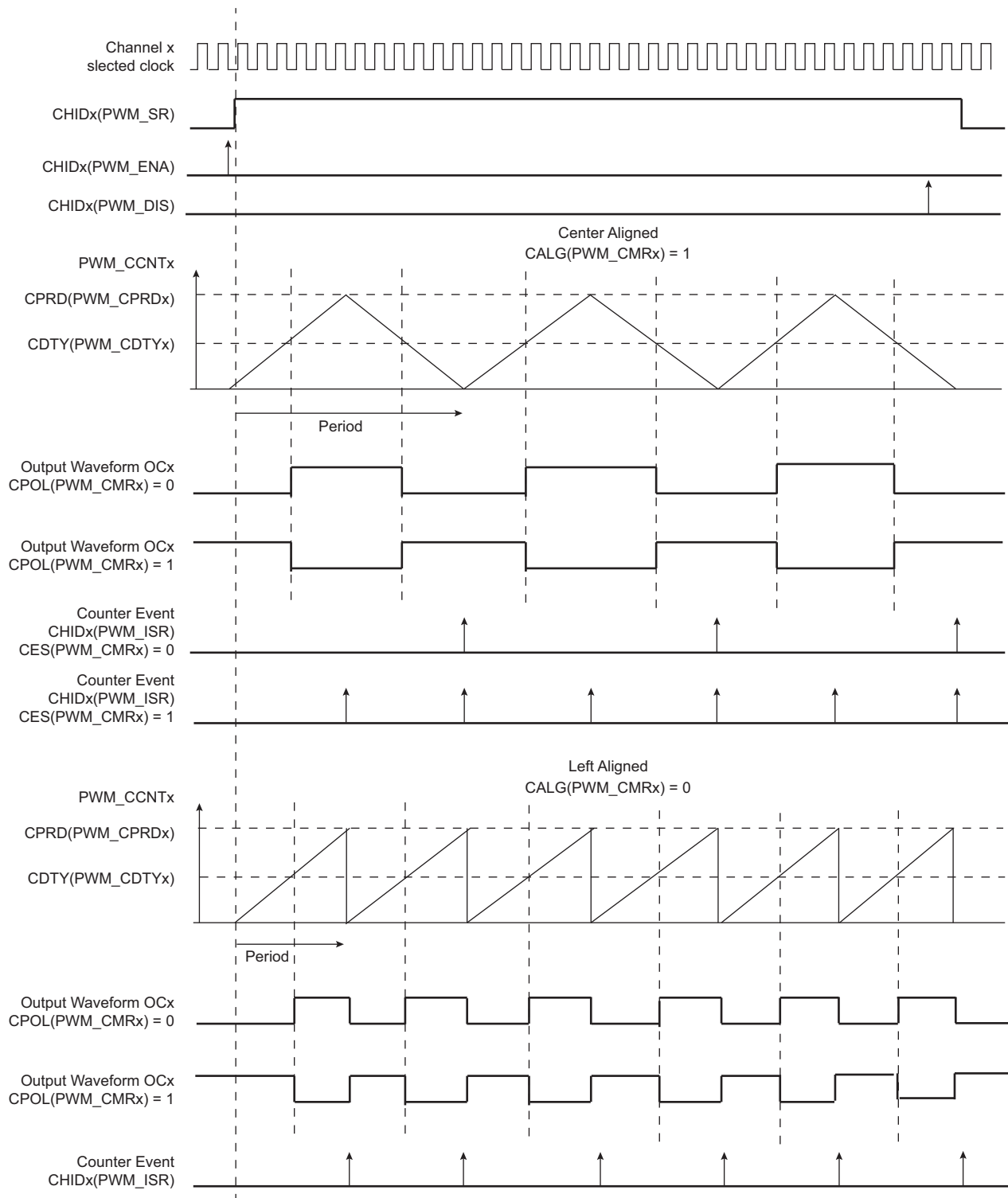
Figure 39-5. Waveform Properties
