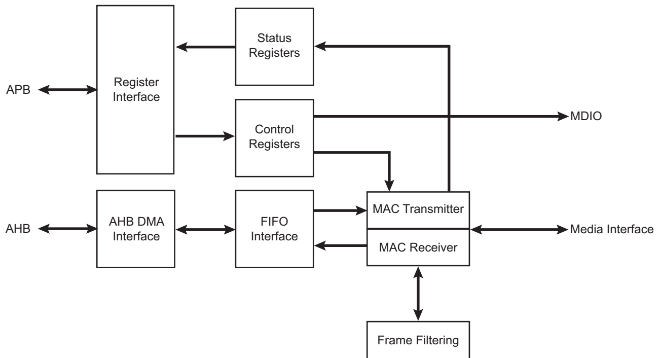
Figure 42-1. Block Diagram
