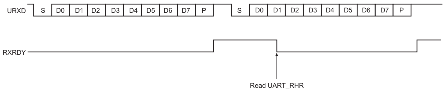
Figure 36-5. Receiver Ready
