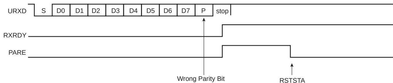
Figure 36-7. Parity Error
