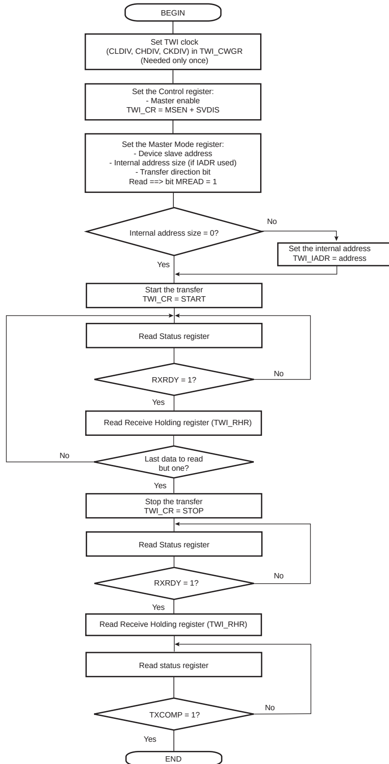
Figure 35-19. TWI Read Operation with Multiple Data Bytes with or without Internal Address
