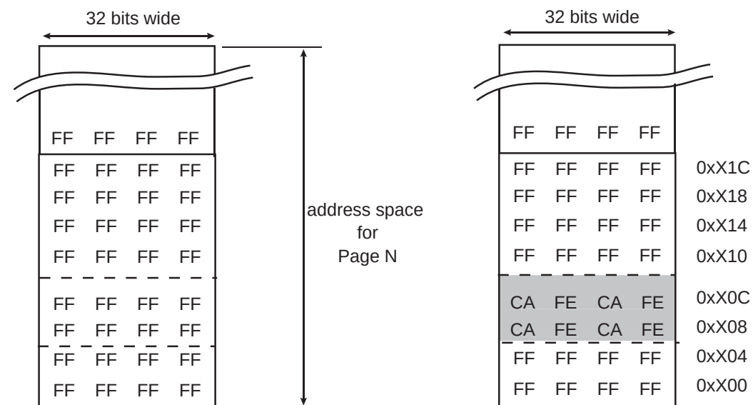
Figure 20-9. Partial Page Programming
