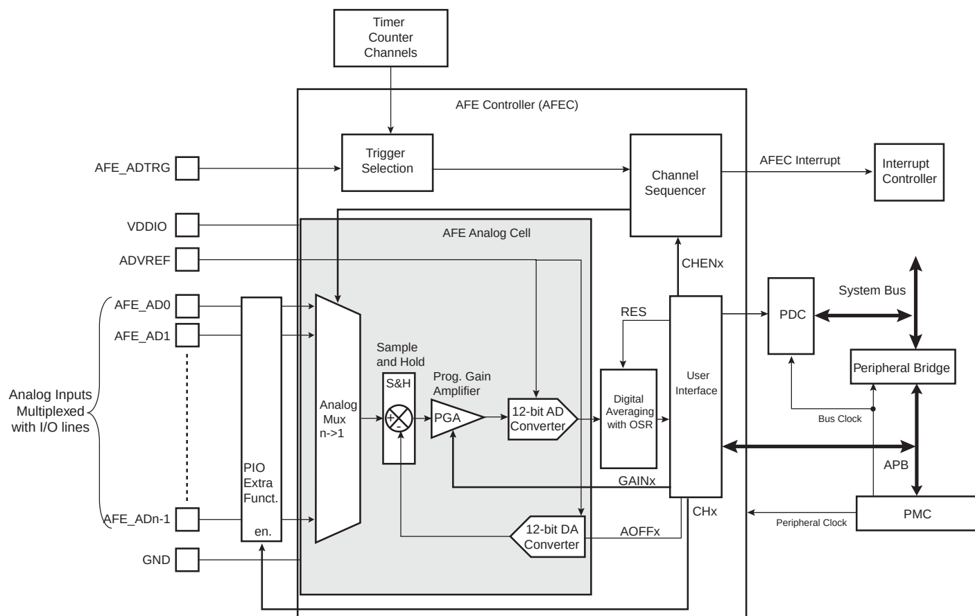
Figure 43-1. Analog Front-End Controller Block Diagram
