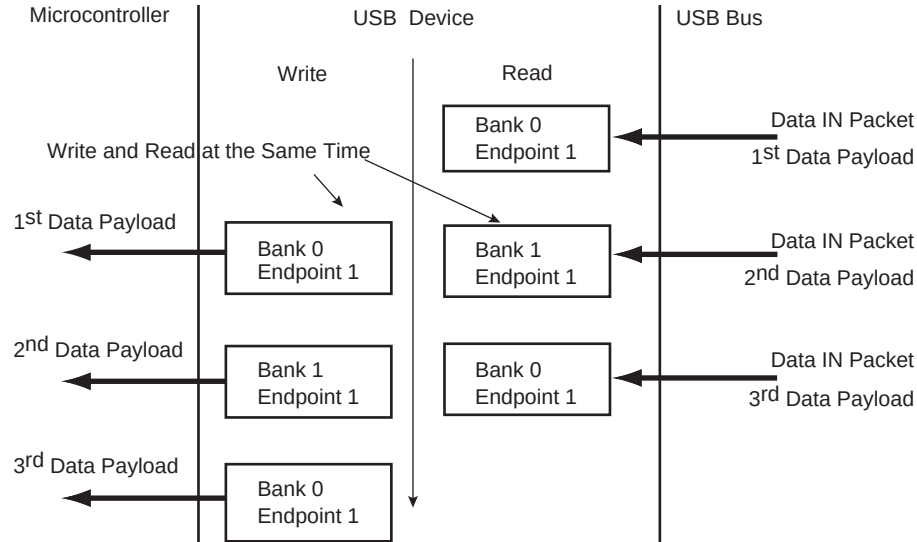
Figure 41-10. Bank Swapping in Data OUT Transfers for Ping-pong Endpoints
