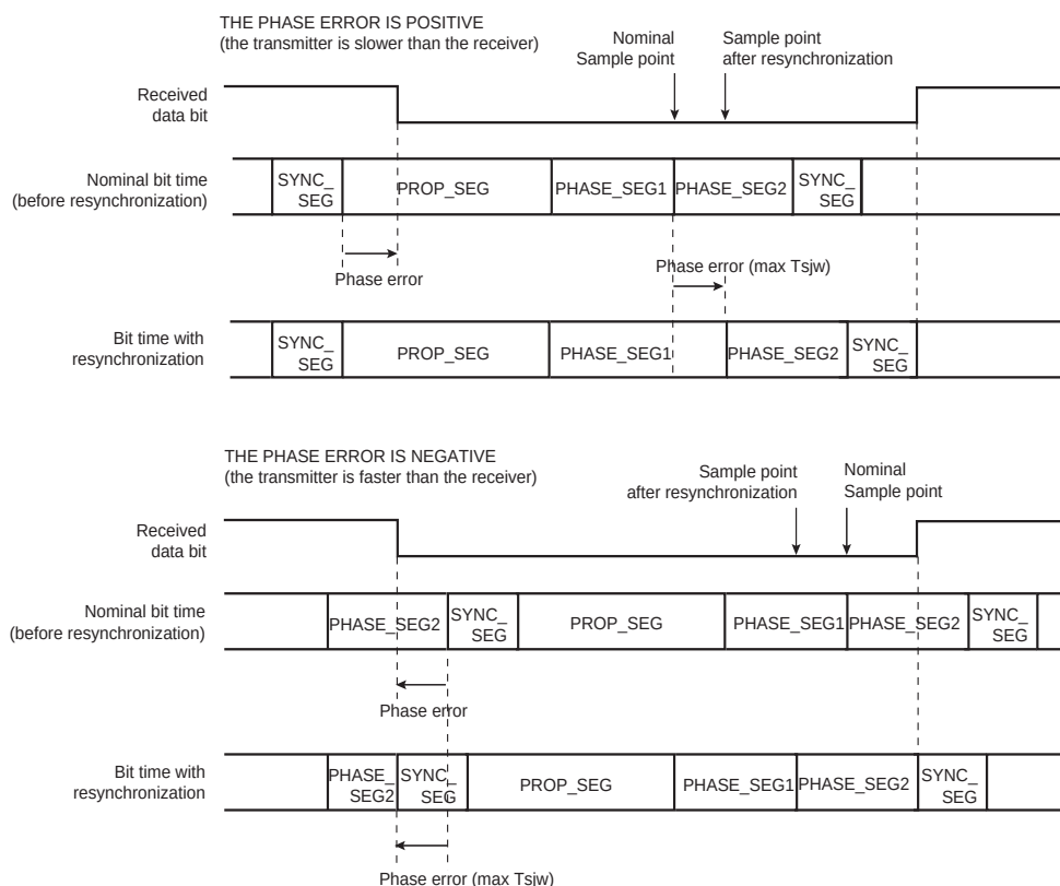
Figure 31-6. CAN Resynchronization
