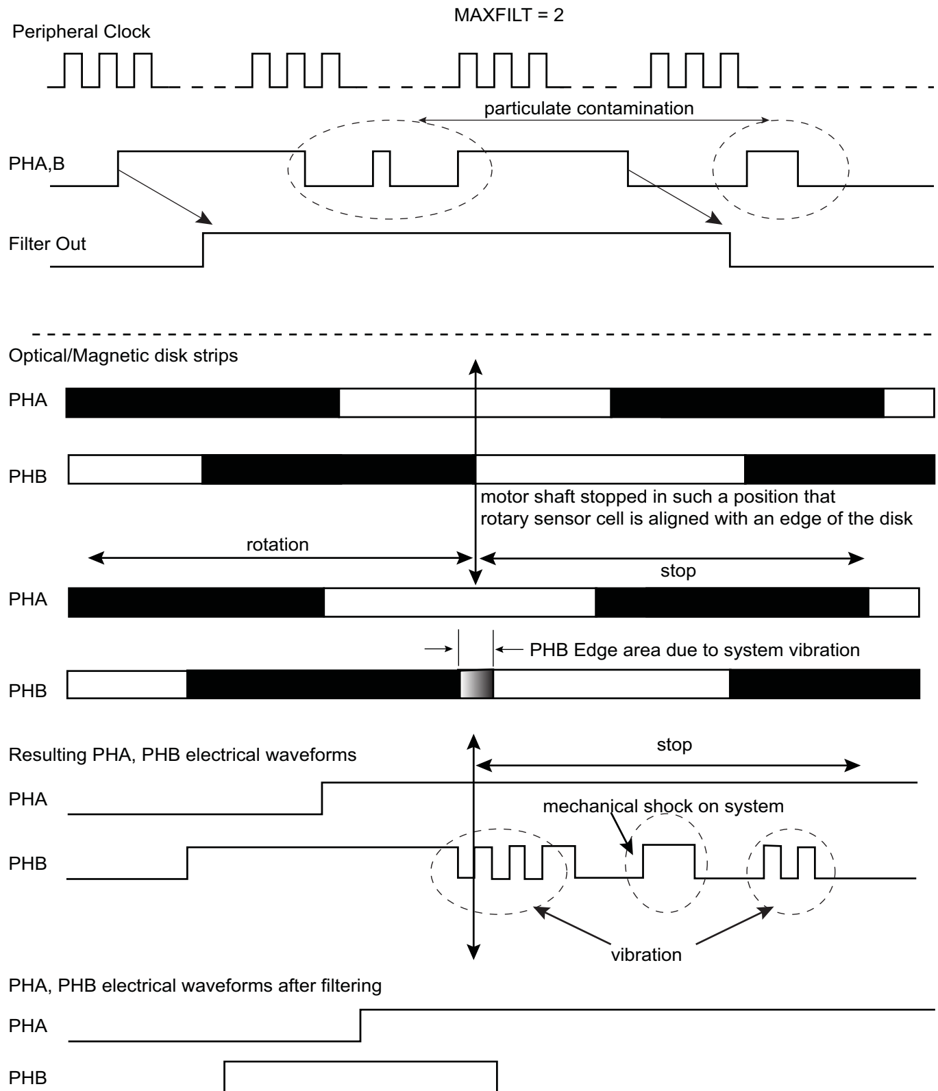
Figure 38-19. Filtering Examples
