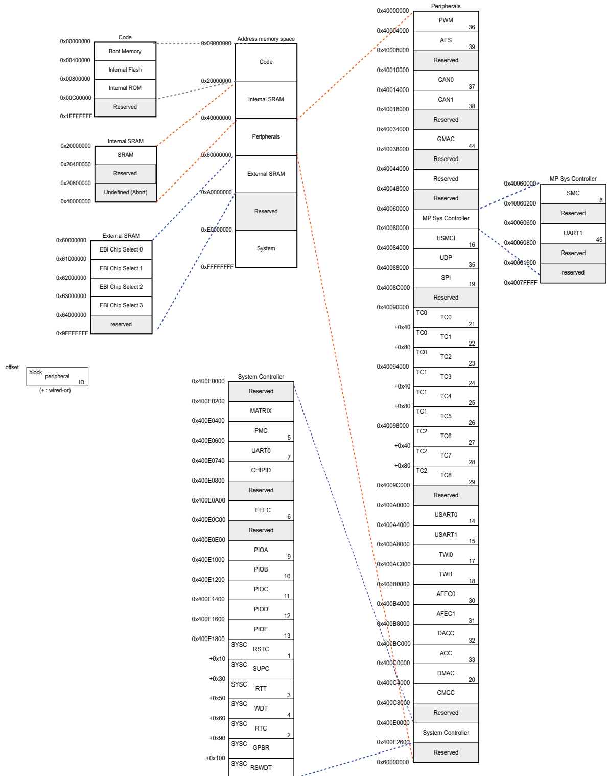
Figure 7-1. SAM4E Product Mapping
