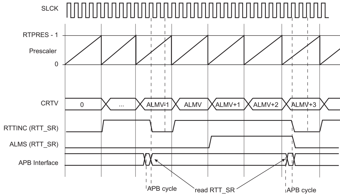
Figure 14-2. RTT Counting
