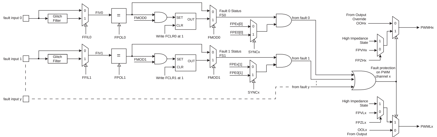
Figure 39-11. Fault Protection
