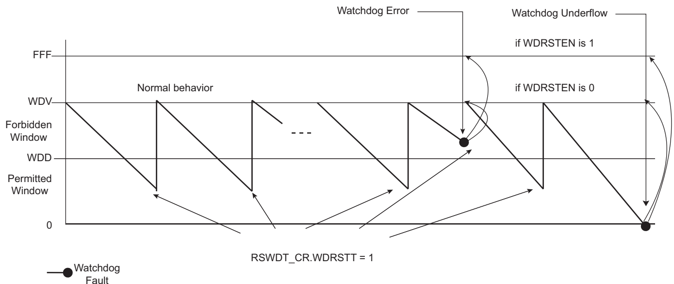
Figure 17-2. Watchdog Behavior
