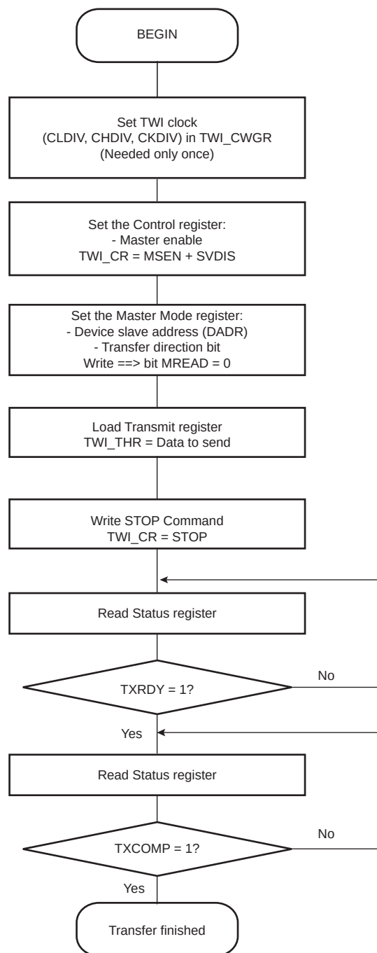
Figure 35-14. TWI Write Operation with Single Data Byte without Internal Address
