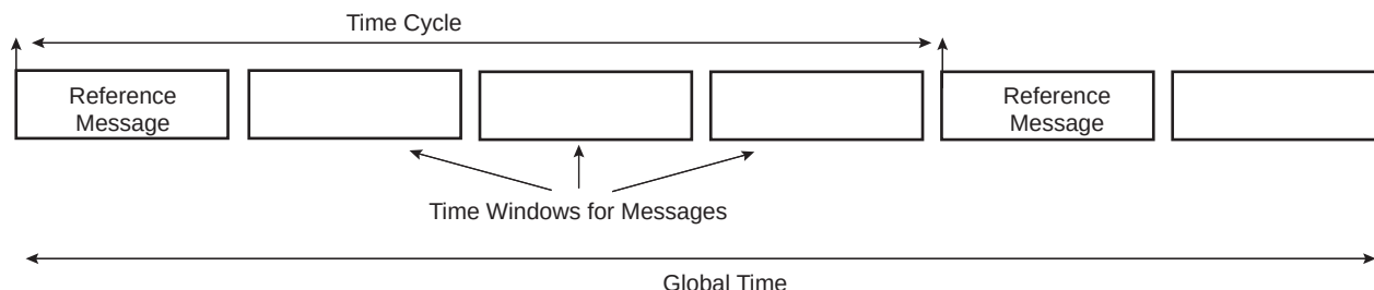
Figure 31-20. Time Triggered Principle
