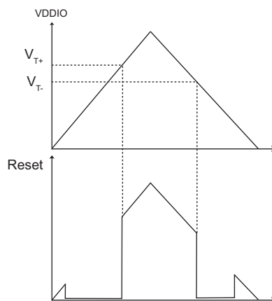
Figure 46-3. Zero-Power-On Reset Characteristics
