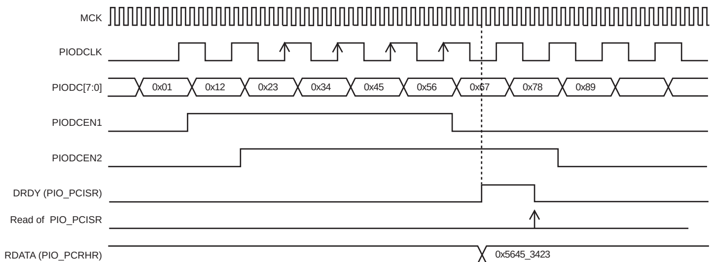
Figure 33-10. Parallel Capture Mode Waveforms (DSIZE = 2, ALWYS = 0, HALFS = 0)
