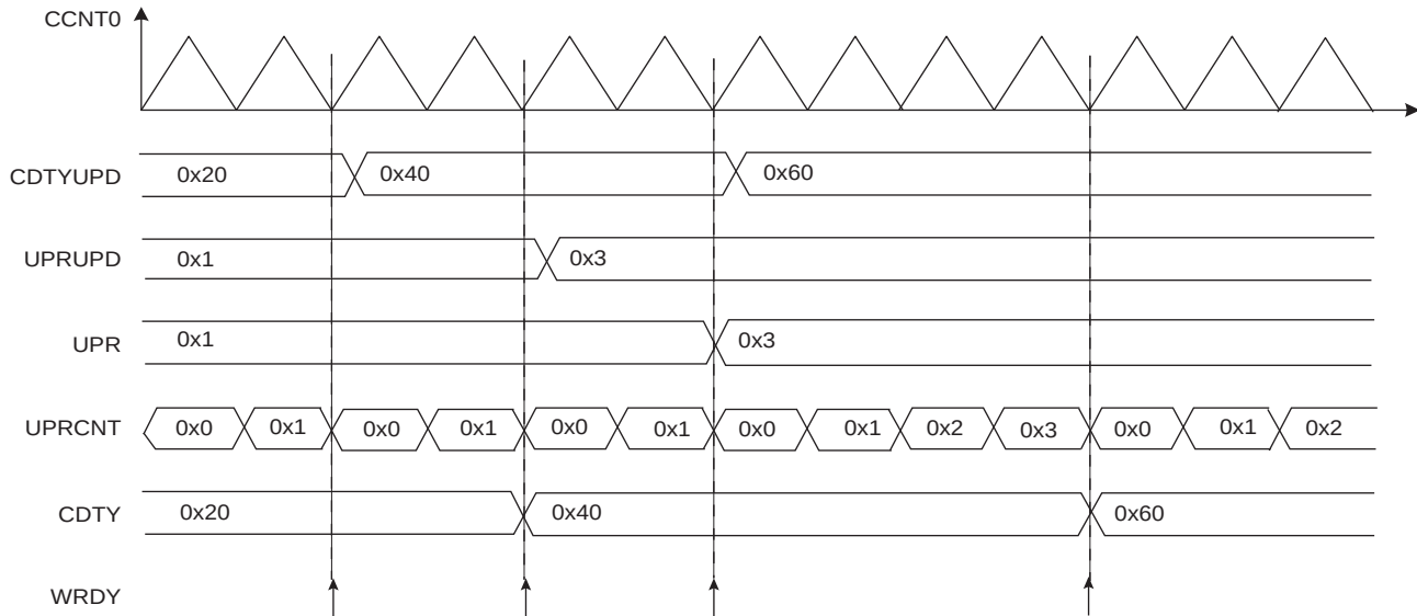
Figure 39-14. Method 2 (UPDM = 1)
