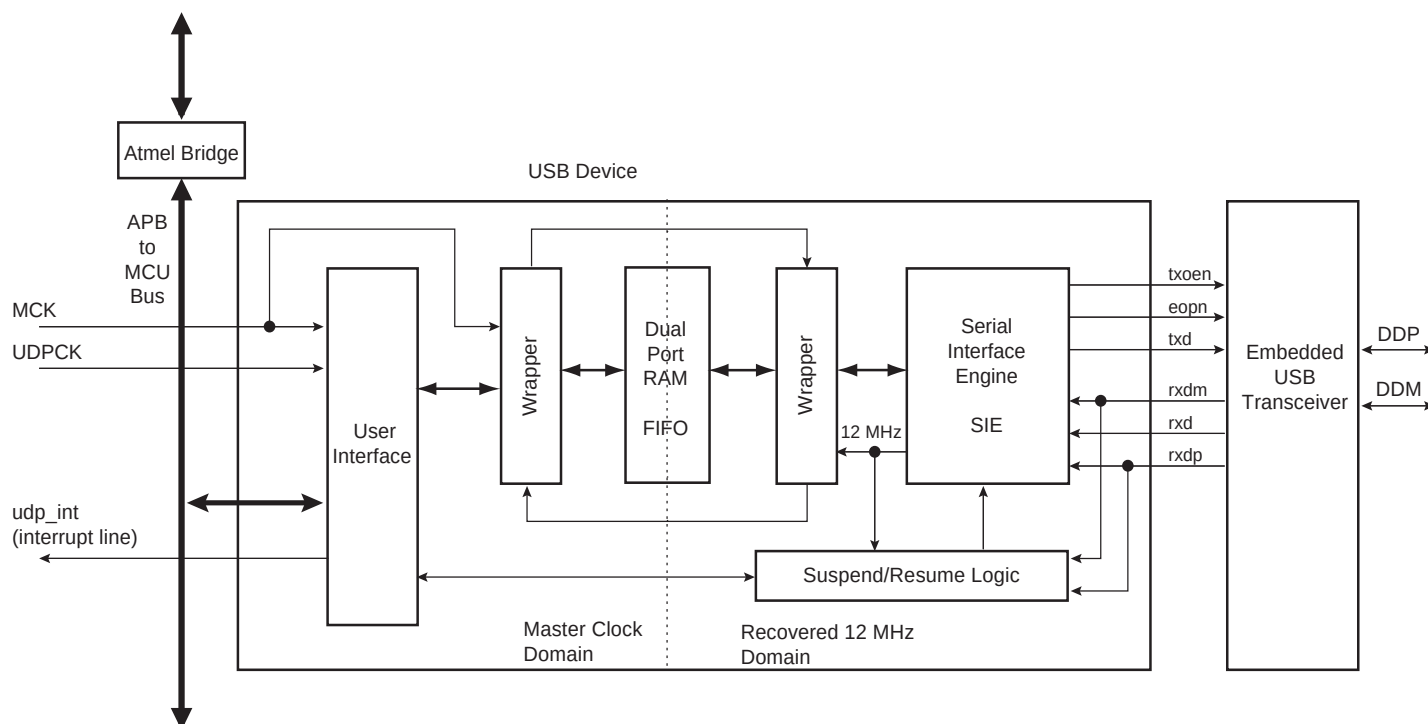
Figure 41-1. Block Diagram
