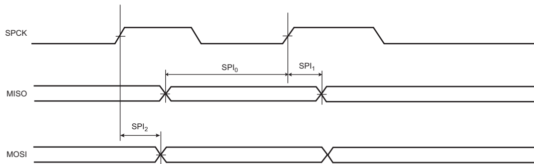
Figure 46-21. SPI Master Mode with (CPOL = NCPHA = 0) or (CPOL = NCPHA = 1)
