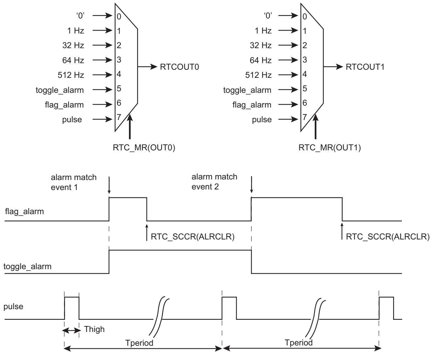
Figure 15-6. Waveform Generation
