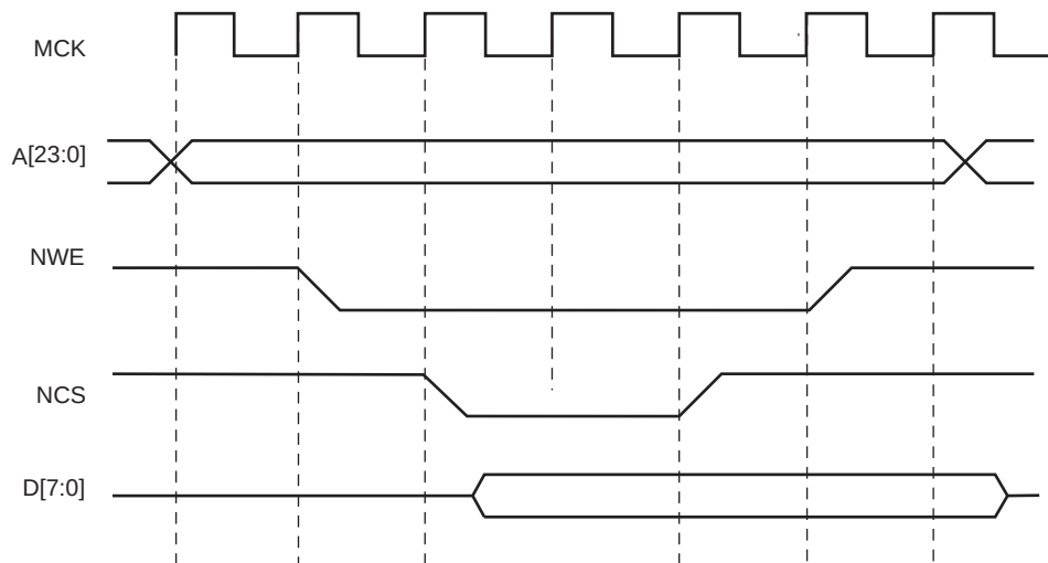
Figure 27-12. WRITE_MODE = 0. Write Operation is Controlled by NCS
