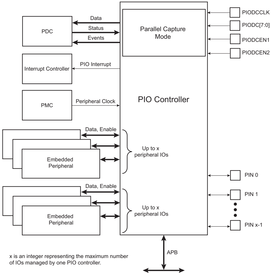
Figure 33-1. Block Diagram
