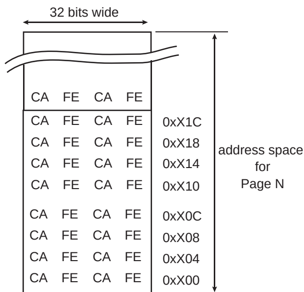
Figure 20-8. Full Page Programming
