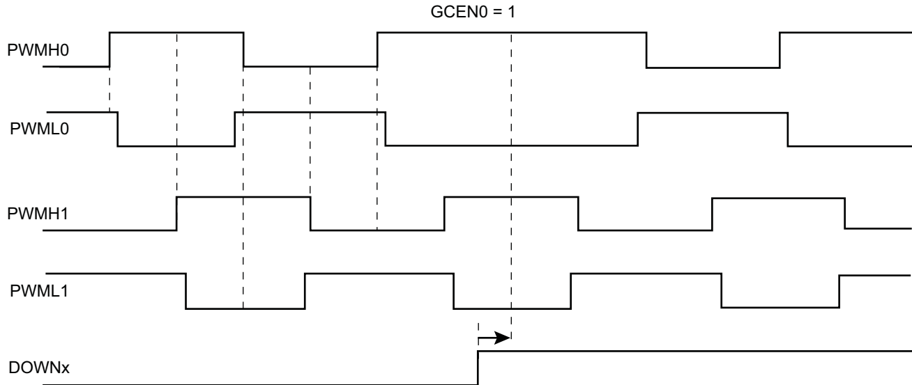
Figure 39-8. 2-bit Gray Up/Down Counter
