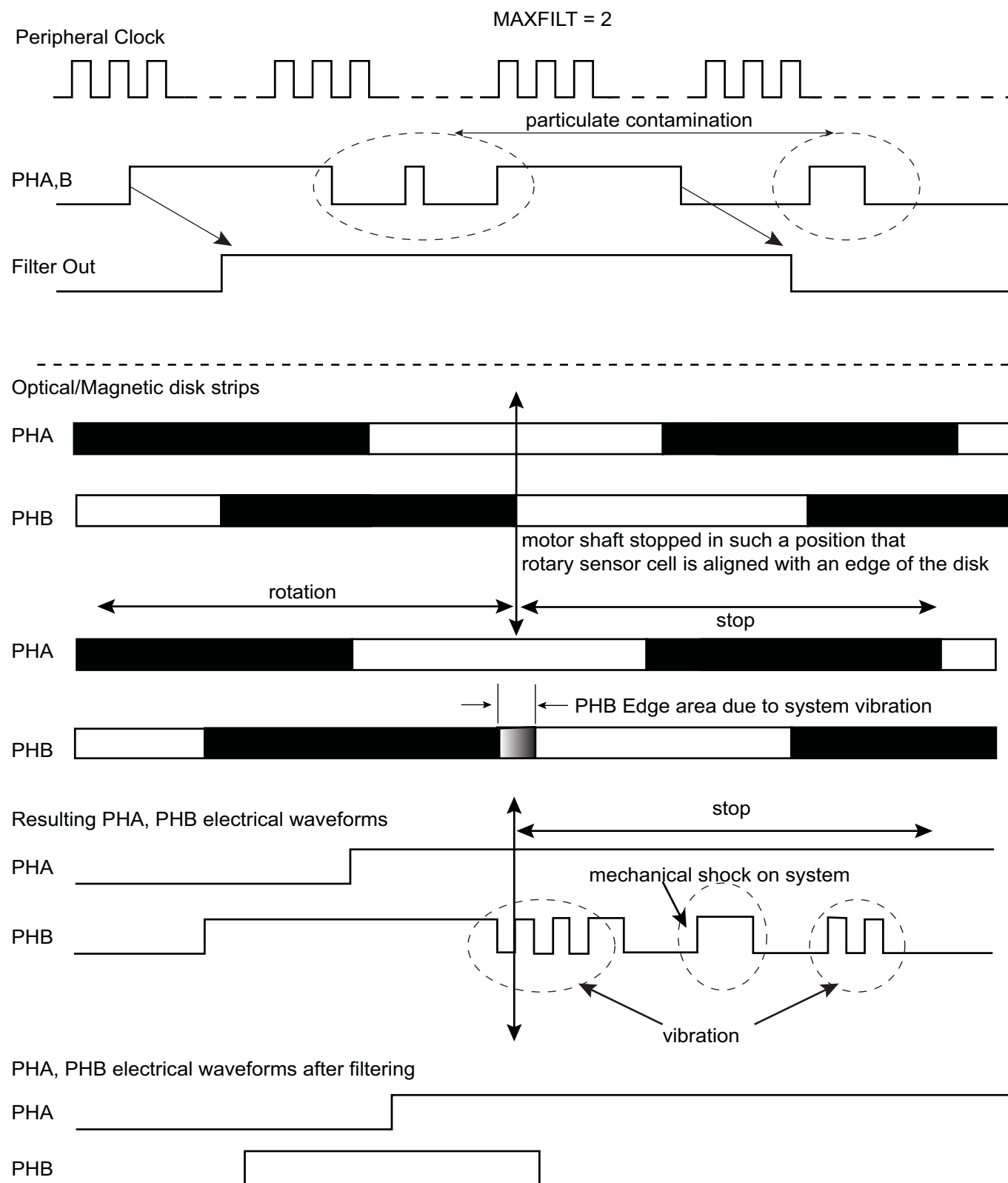
Figure 38-19. Filtering Examples
