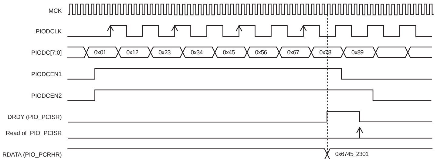
Figure 33-12. Parallel Capture Mode Waveforms (DSIZE = 2, ALWYS = 0, HALFS = 1, FRSTS = 0)
