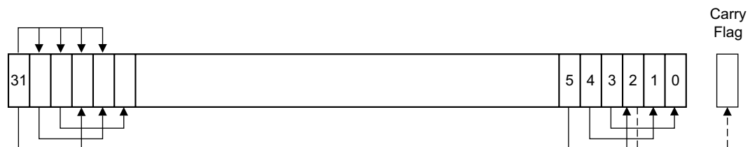
Figure 11-8. ASR #3
