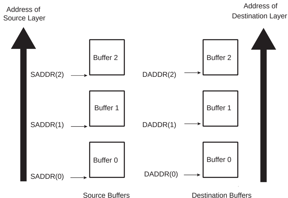
Figure 25-5. Multi-buffer with Linked List Address for Source and Destination
