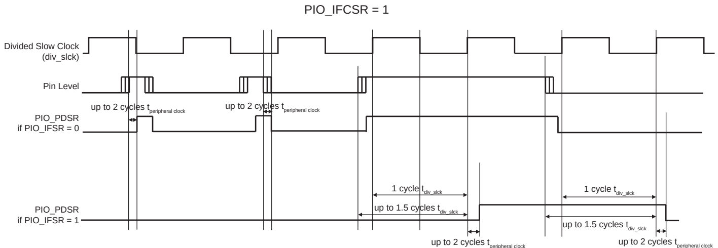
Figure 33-5. Input Debouncing Filter Timing
