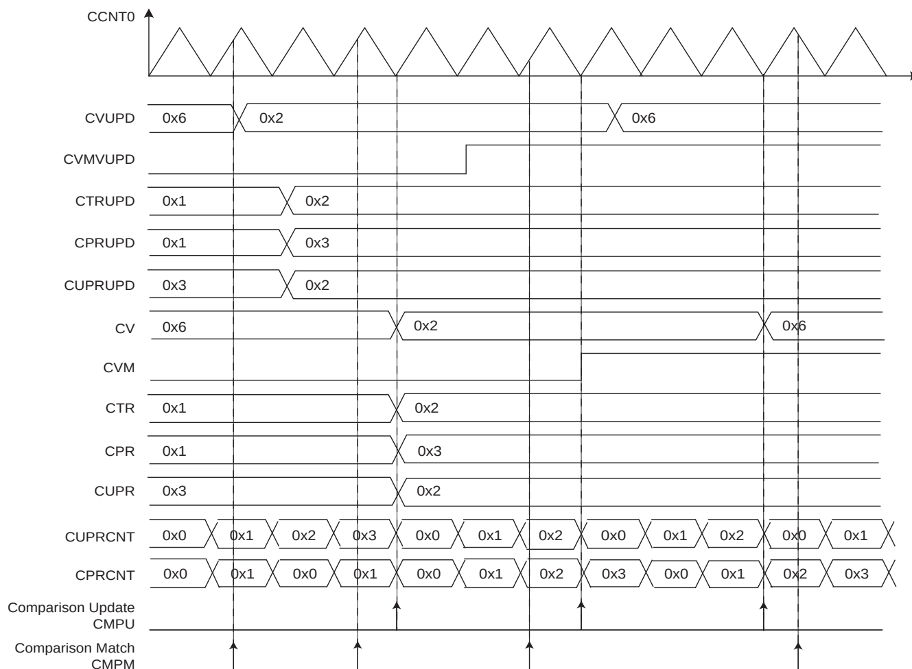
Figure 39-18. Comparison Waveform
