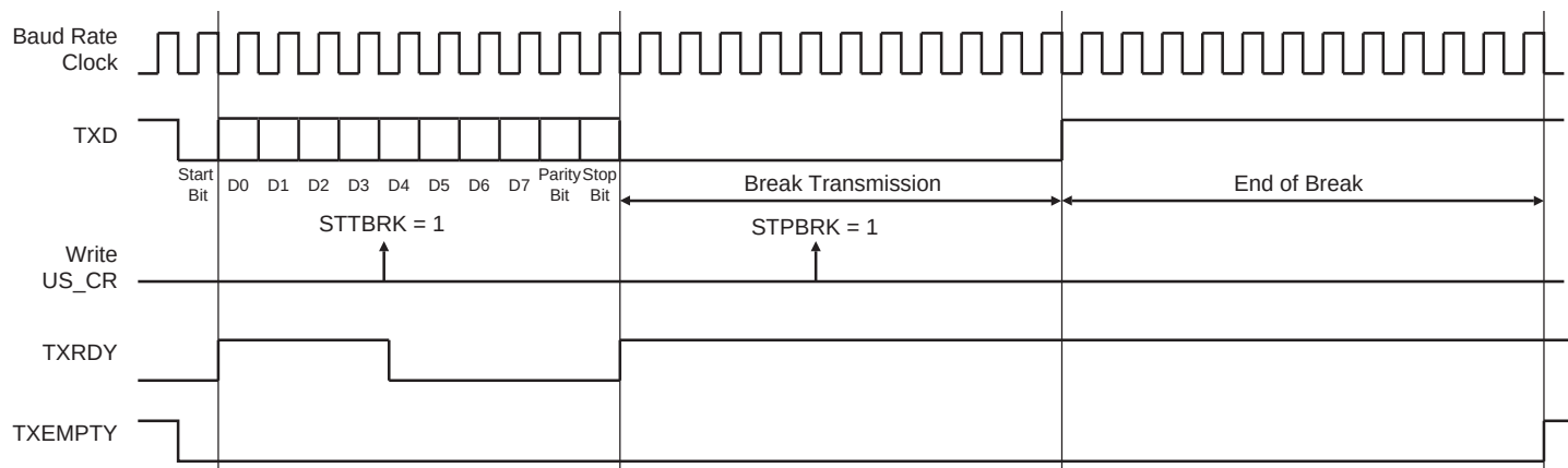
Figure 37-25. Break Transmission
