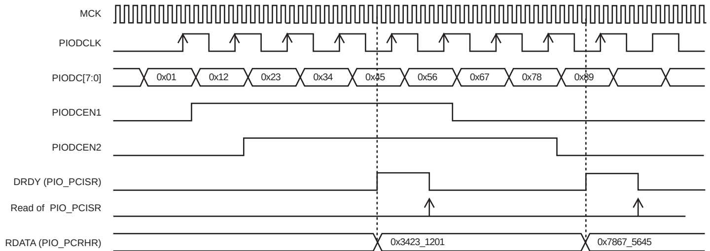
Figure 33-11. Parallel Capture Mode Waveforms (DSIZE = 2, ALWYS = 1, HALFS = 0)
