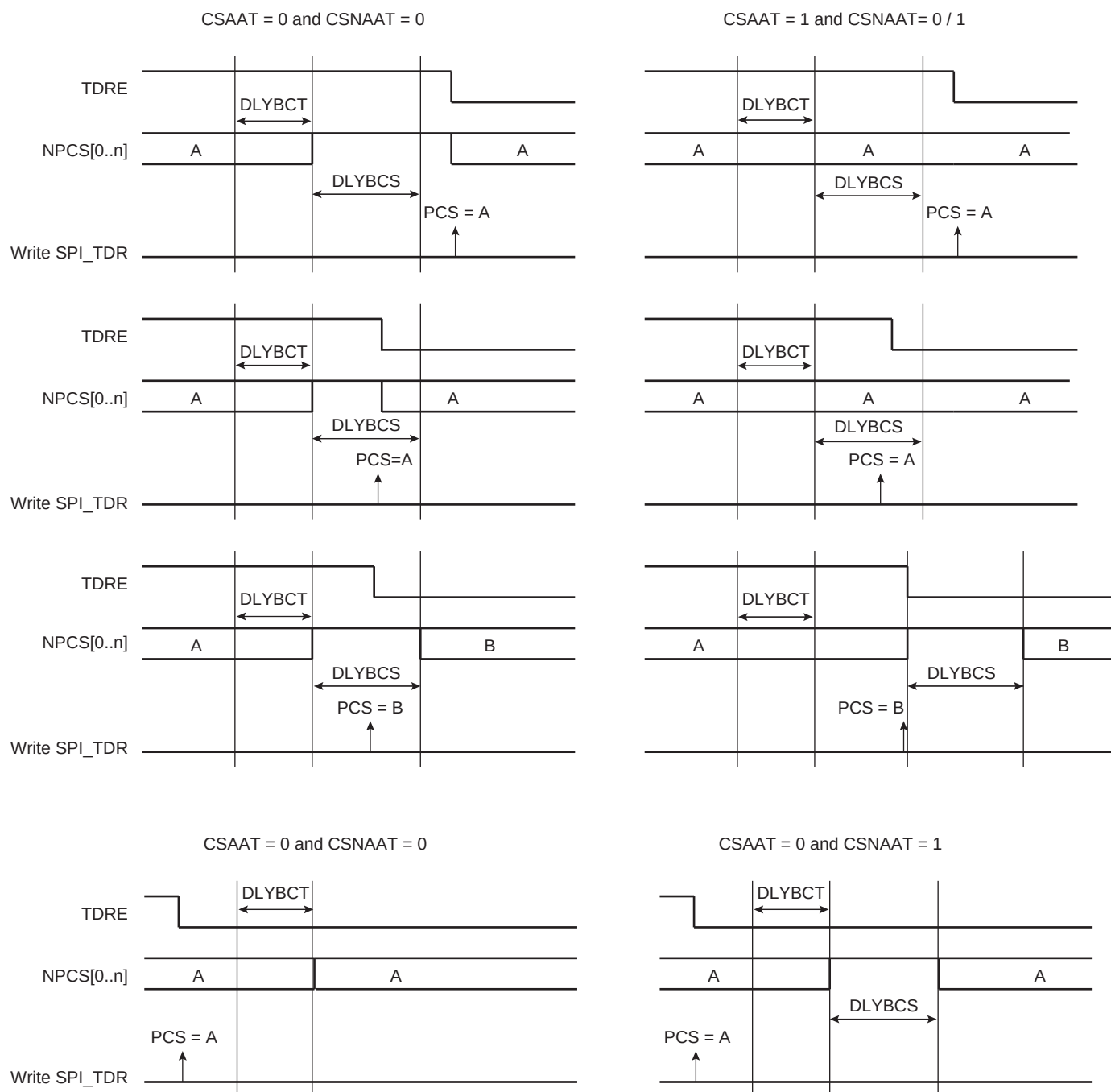
Figure 34-12. Peripheral Deselection
