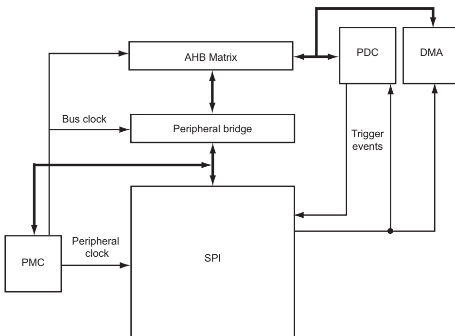
Figure 34-1. Block Diagram
