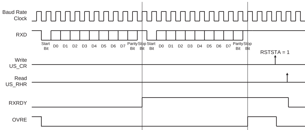
Figure 37-20. Receiver Status
