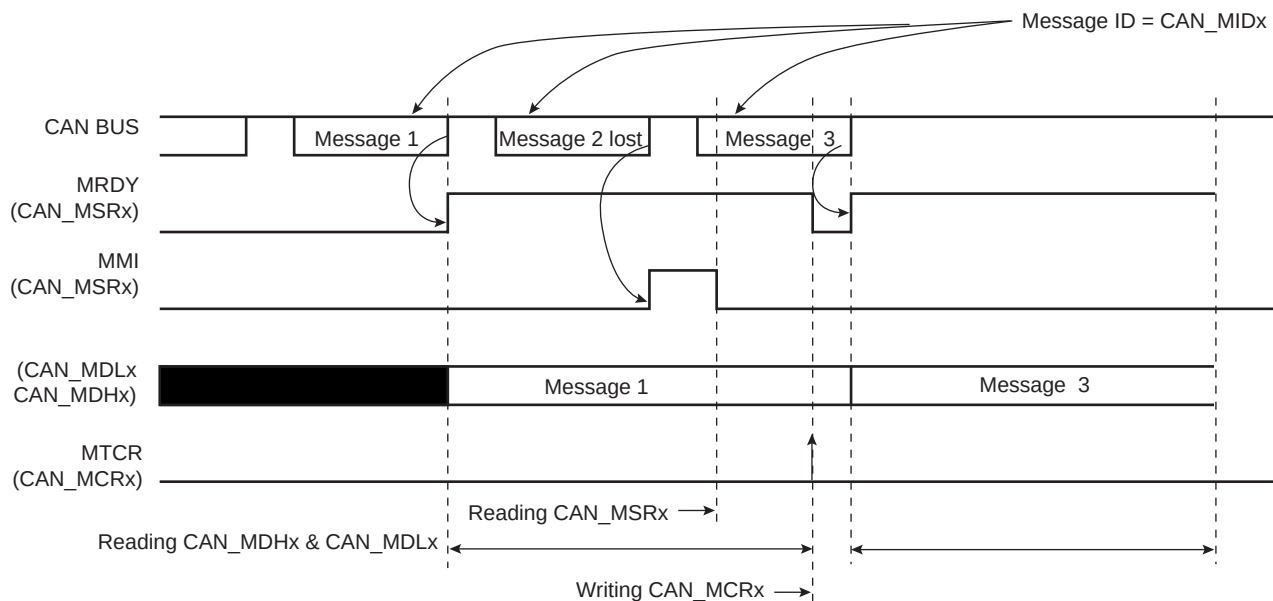
Figure 31-11. Receive Mailbox
