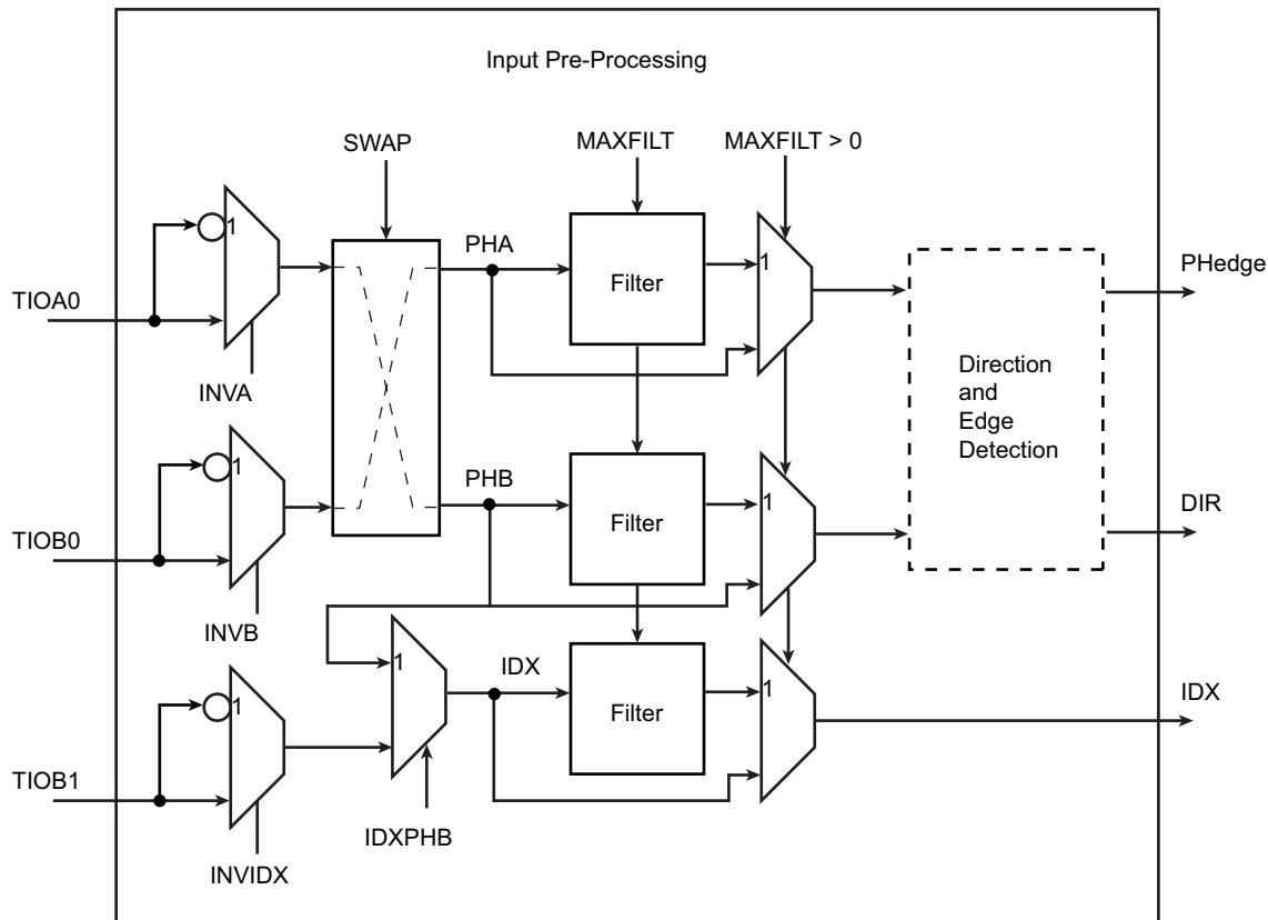
Figure 38-18. Input Stage
