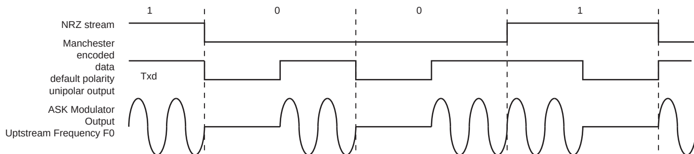
Figure 37-17. ASK Modulator Output
