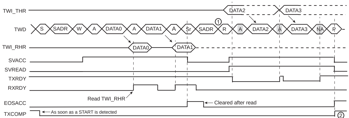
Figure 35-29. Repeated Start + Reversal from Write to Read Mode
