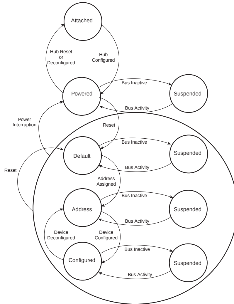
Figure 41-14. USB Device State Diagram
