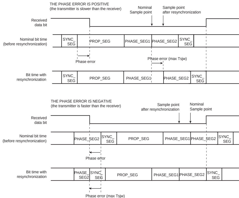
Figure 31-6. CAN Resynchronization
