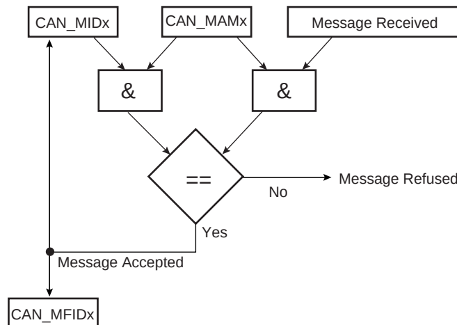
Figure 31-3. Message Acceptance Procedure
