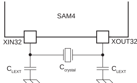
Figure 46-11. 32.768 kHz Crystal Oscillator Schematics
