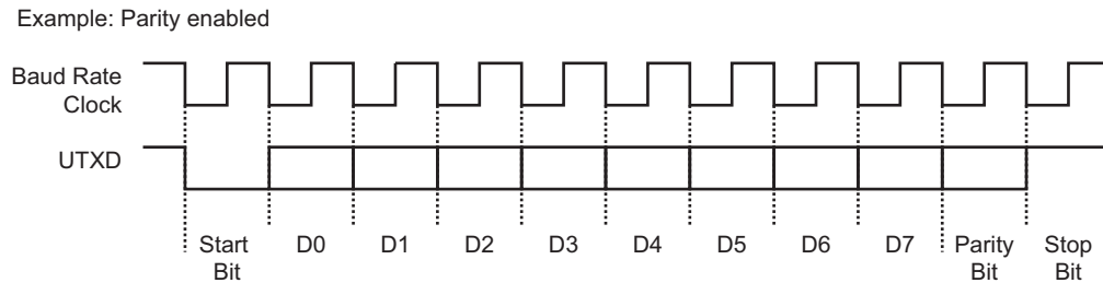
Figure 36-9. Character Transmission
