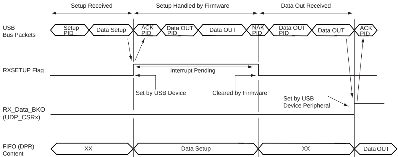
Figure 41-5. Setup Transaction Followed by a Data OUT Transaction
