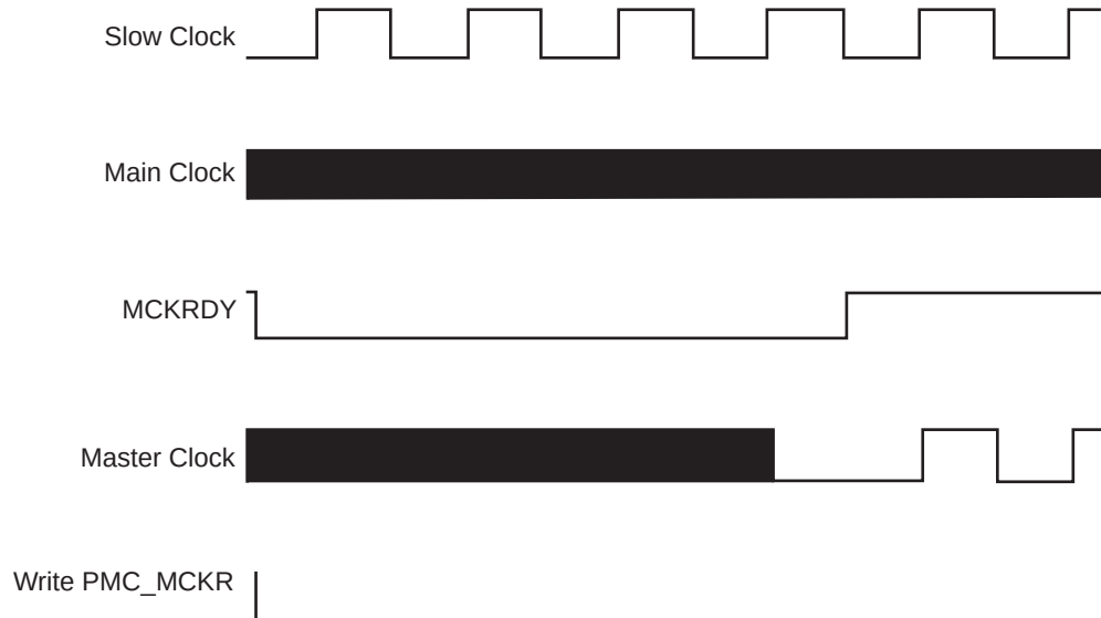
Figure 29-7. Switch Master Clock from Main Clock to Slow Clock
