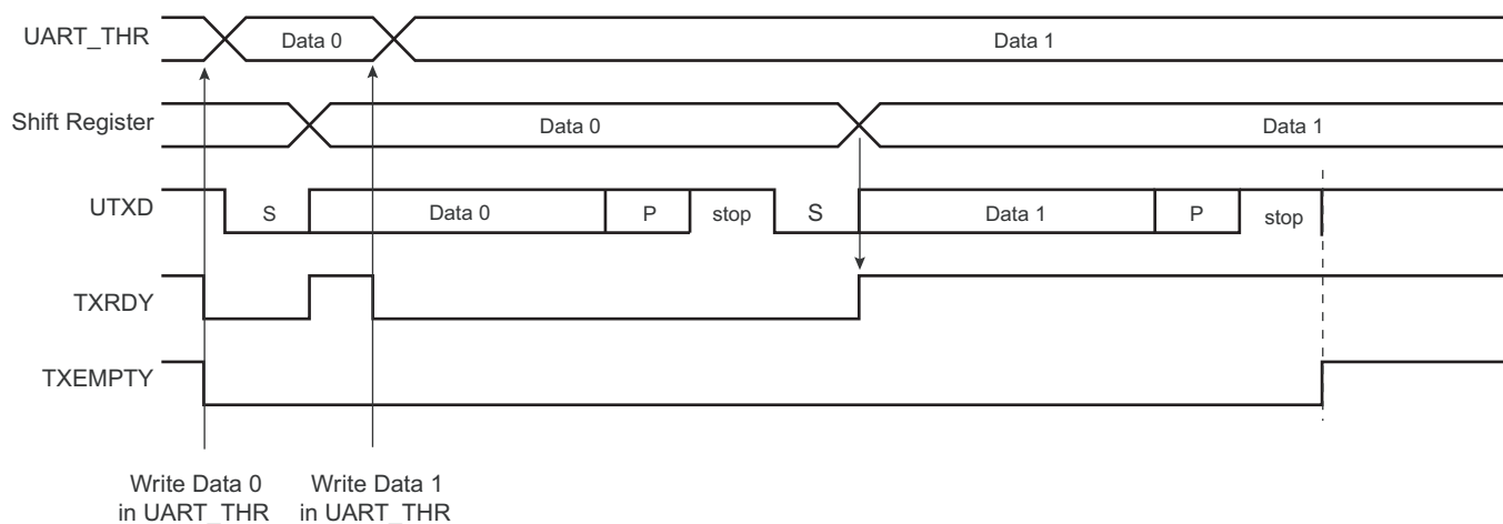
Figure 36-10. Transmitter Control
