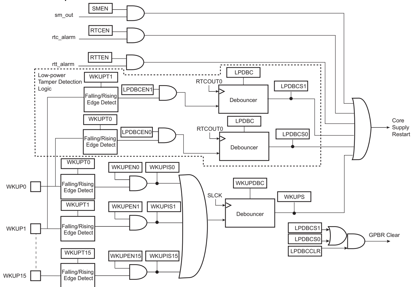
Figure 18-4. Wake-up Sources
