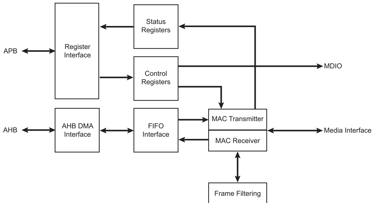
Figure 42-1. Block Diagram
