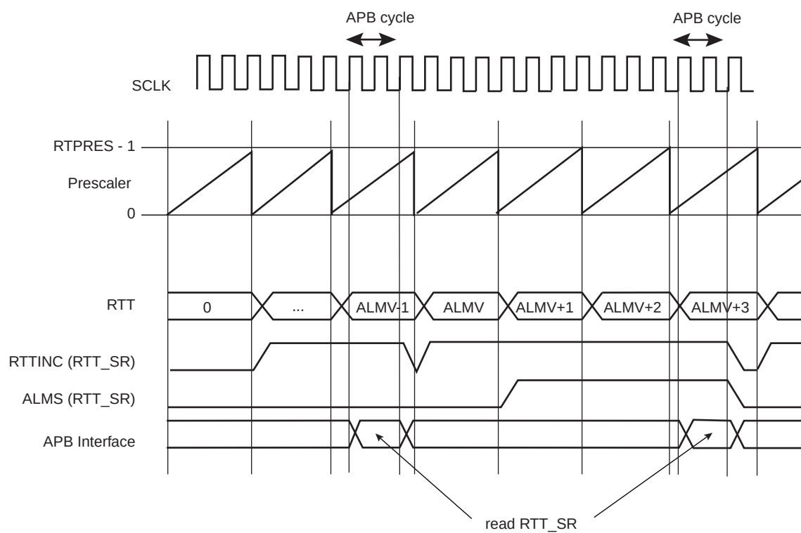
Figure 14-2. RTT Counting
