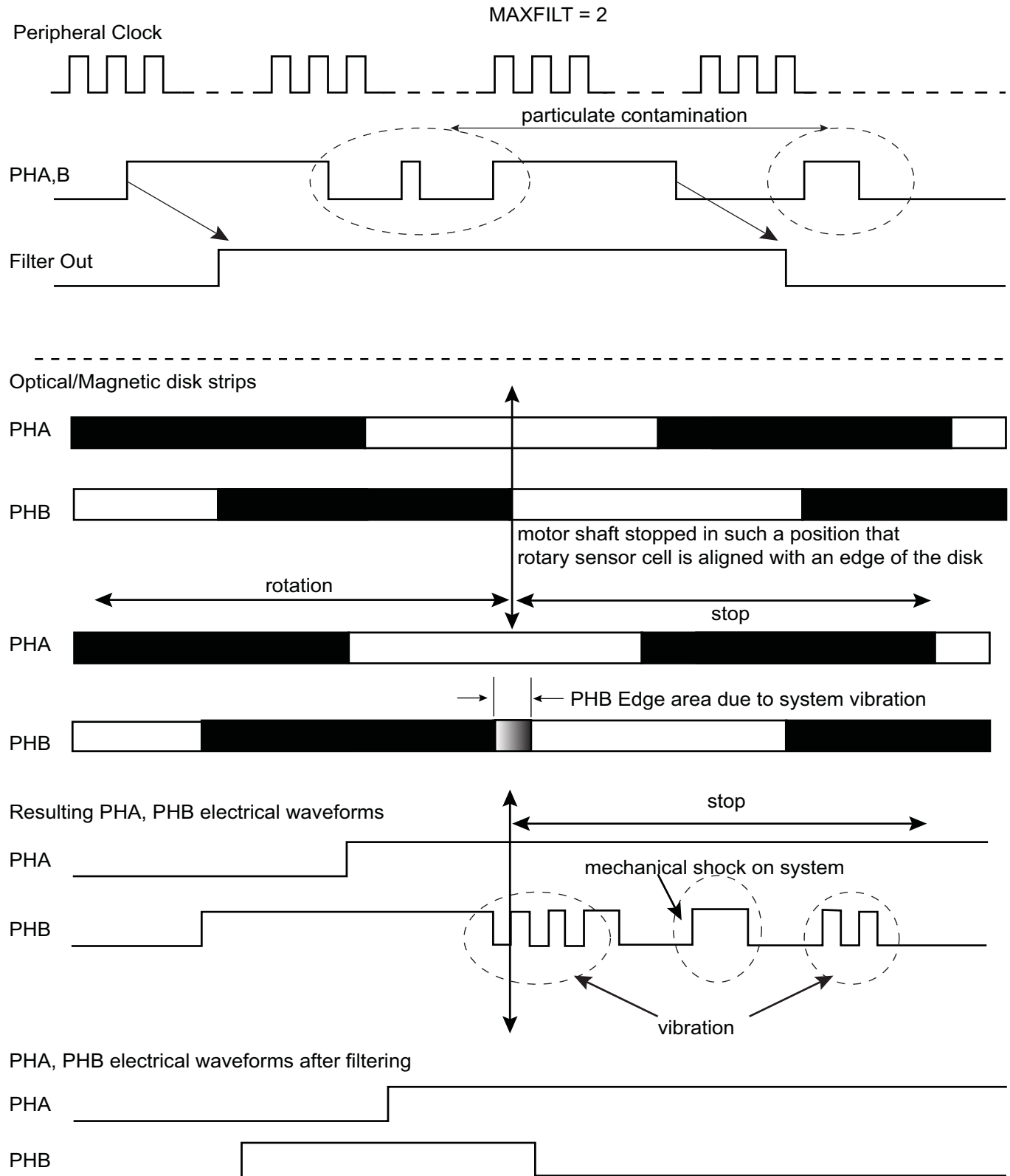
Figure 32-18. Filtering Examples
