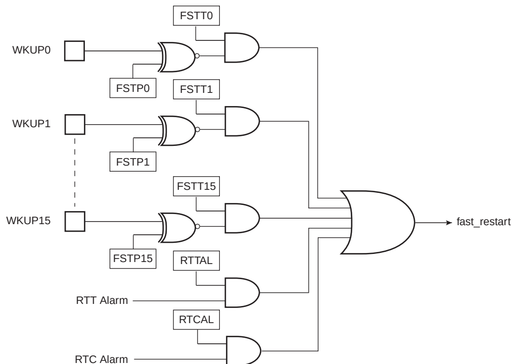
Figure 25-3. Fast Start-up Circuitry
