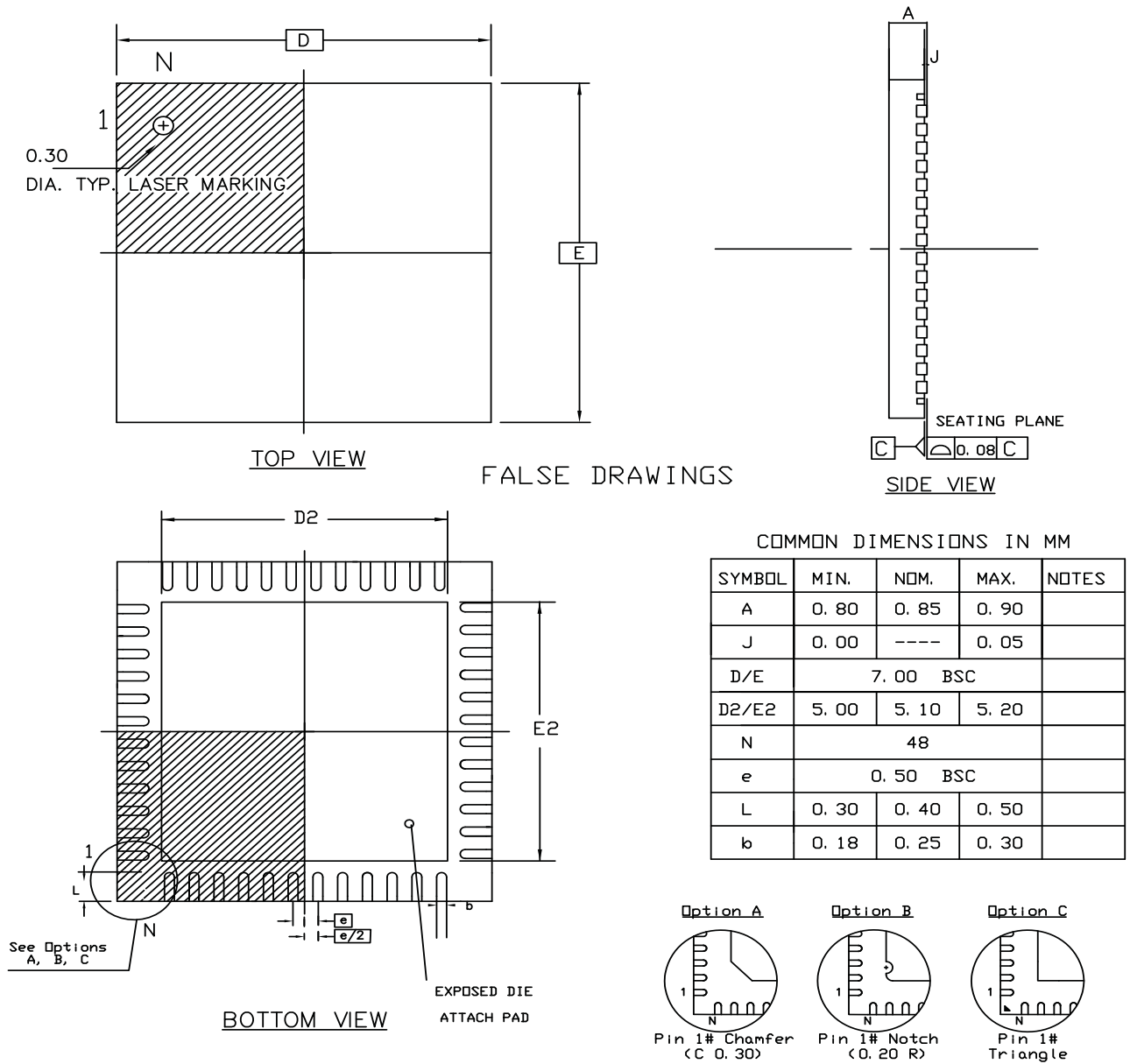
Figure 37-7. 48-pad QFN Package Drawing
