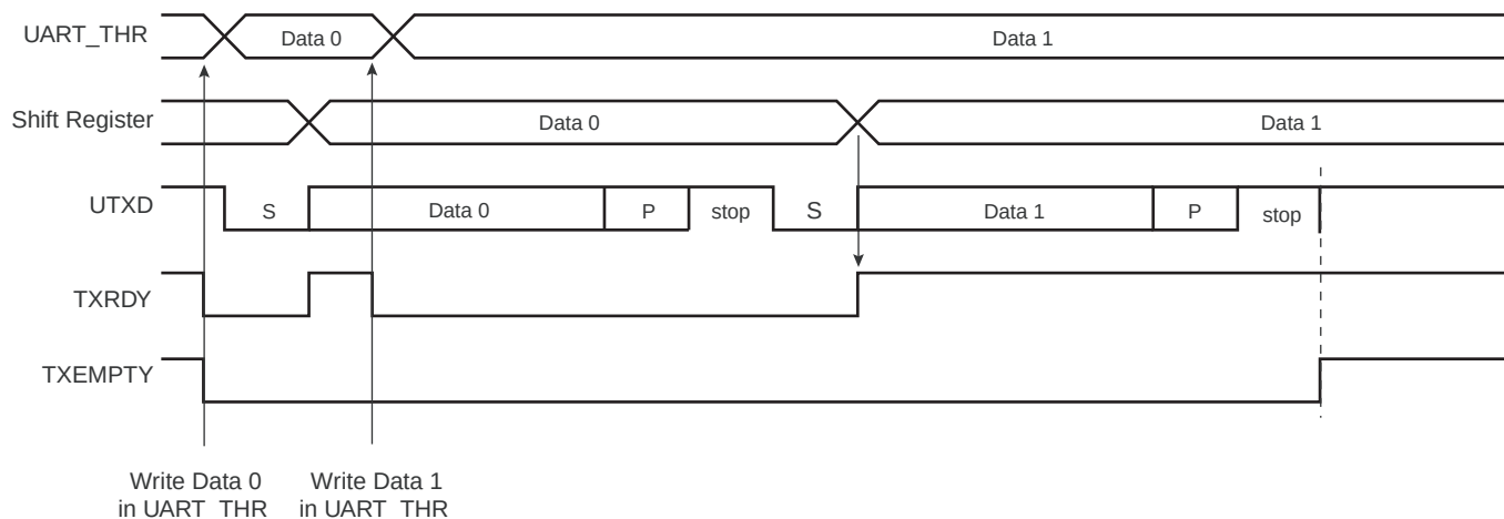
Figure 30-10. Transmitter Control
