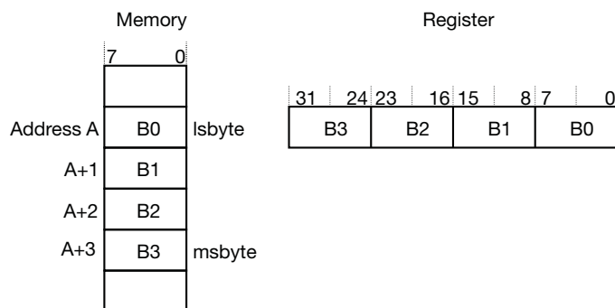
Figure 11-6. Little-endian Format
