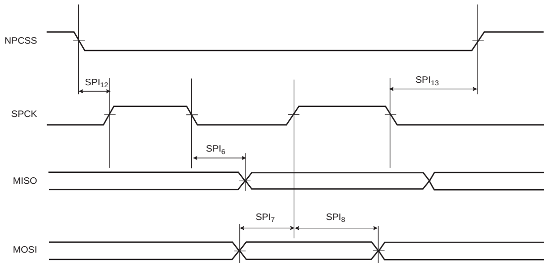
Figure 36-16. SPI Slave Mode with (CPOL = 0 and NCPHA = 1) or (CPOL = 1 and NCPHA = 0)
