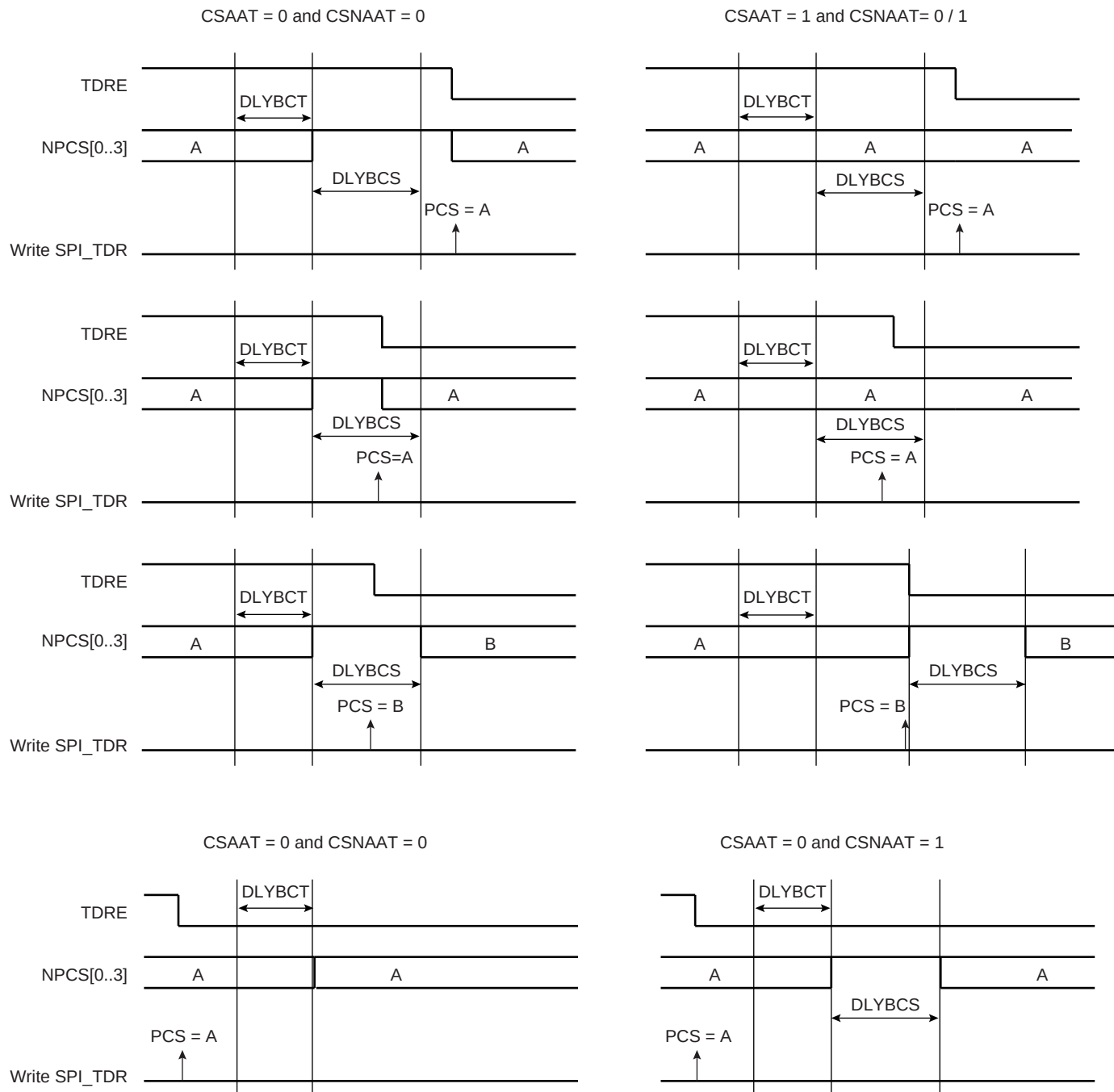
Figure 28-11. Peripheral Deselection
