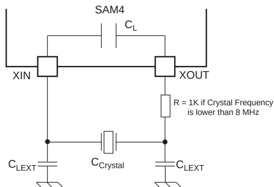
Figure 36-11. 3 to 20 MHz Crystal Oscillator Schematics
