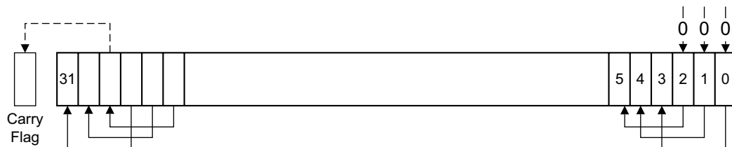
Figure 11-11. LSL #3
