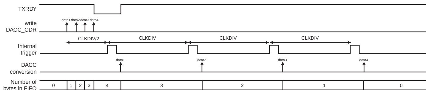
Figure 35-2. Internal trigger
