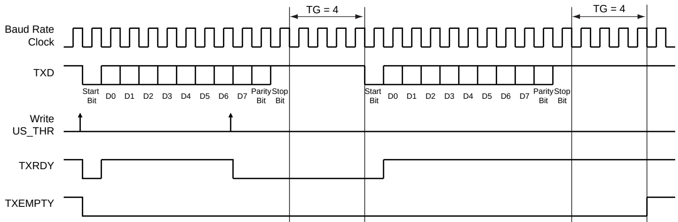
Figure 31-13. Timeguard Operations
