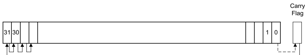
Figure 11-13. RRX
