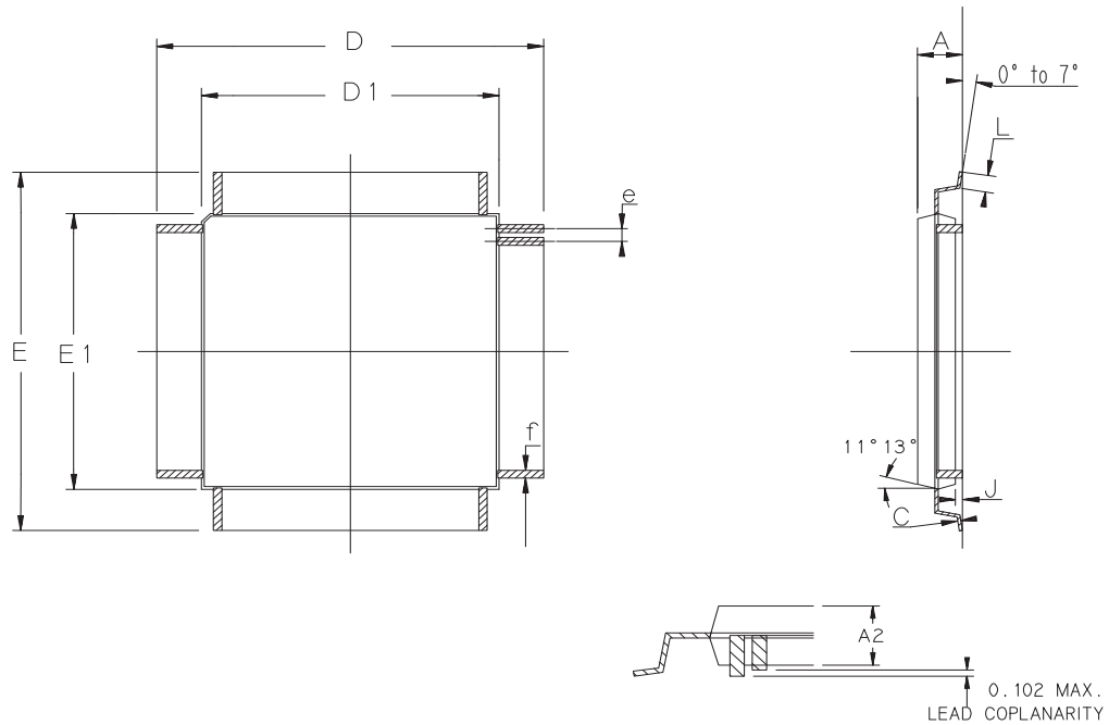
Figure 37-6. 48-lead LQFP Package Drawing
