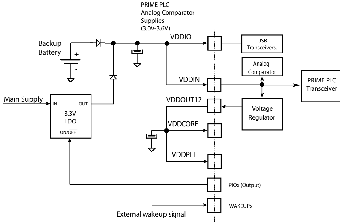
Figure 5-3. Backup Battery
