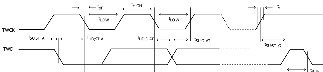
Figure 13-24. Two-wire Serial Bus Timing
