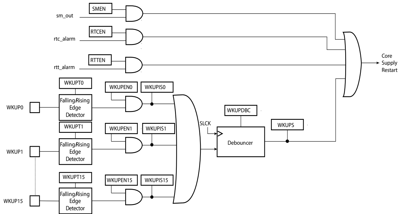
Figure 5-4. Wake-up Sources
