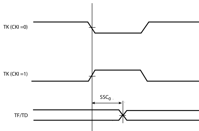
Figure 13-10. SSC Transmitter, TK and TF as output
