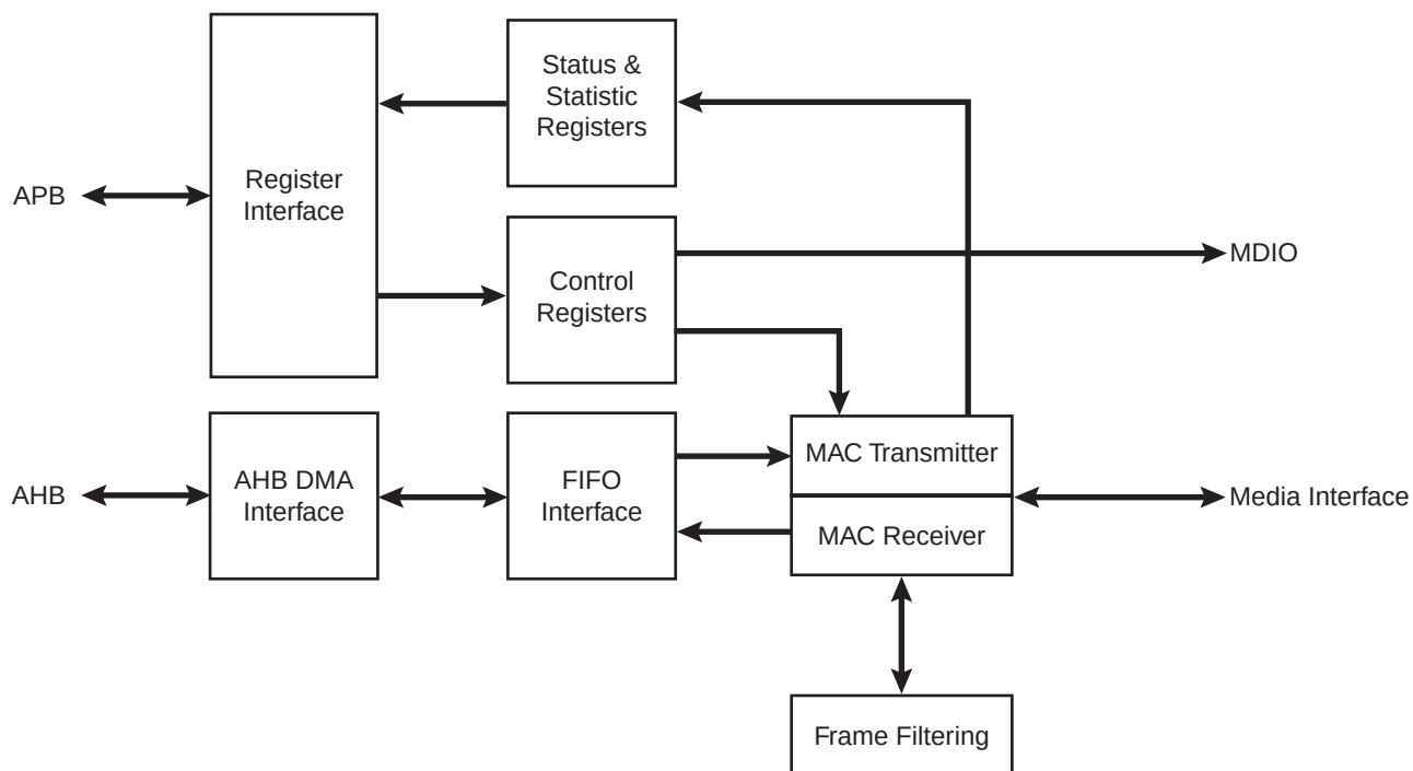
Figure 36-1. Block Diagram
