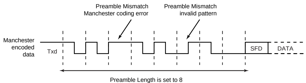
Figure 44-15. Preamble Pattern Mismatch
