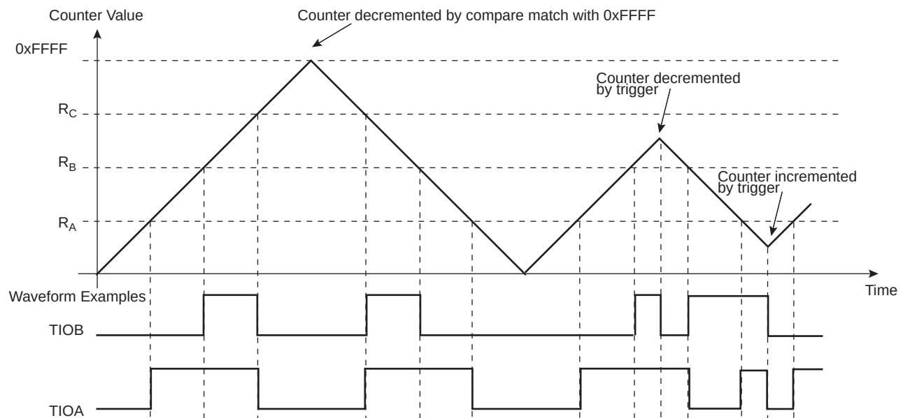
Figure 47-13.WAVSEL = 01 with Trigger
