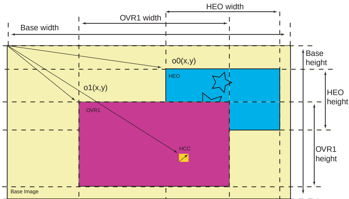
Video Prioritization Algorithm 1 : HCC &gt; OVR1 &gt; HEO &gt; BASE
