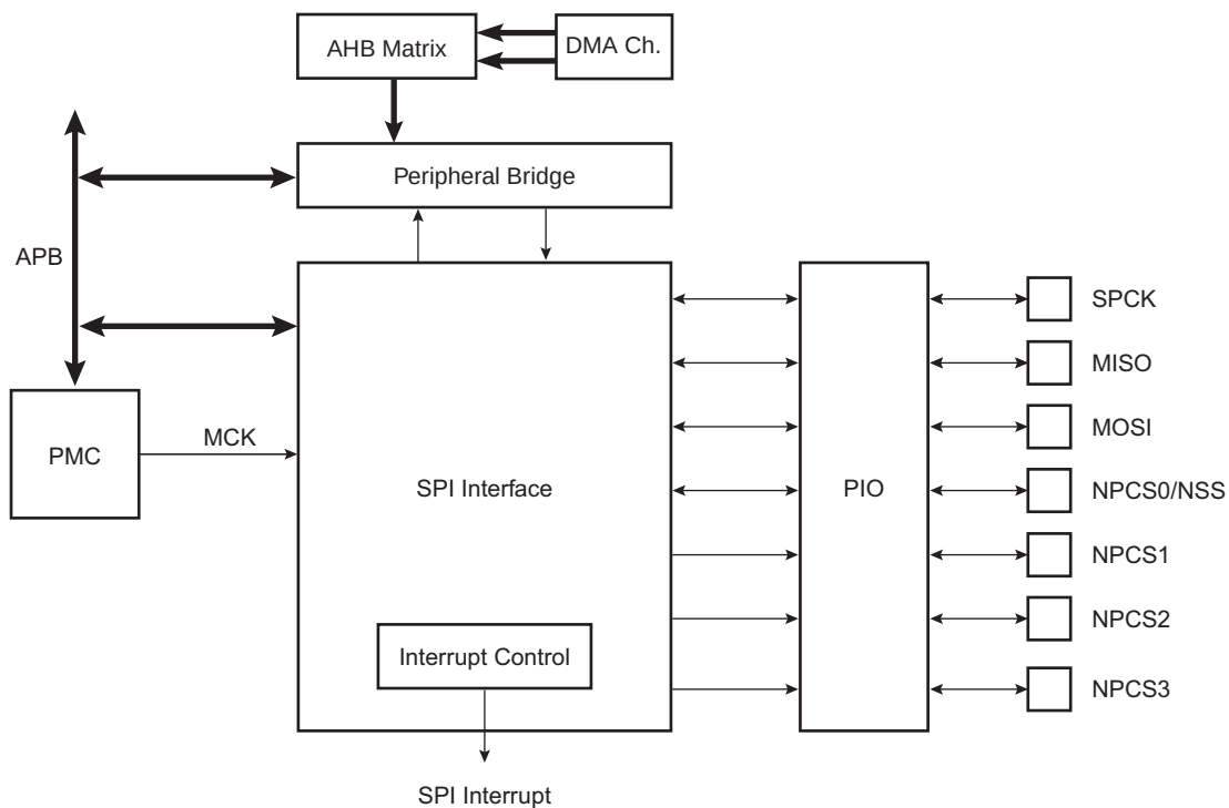
Figure 39-1. Block Diagram
