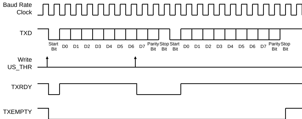
Figure 44-7. Transmitter Status
