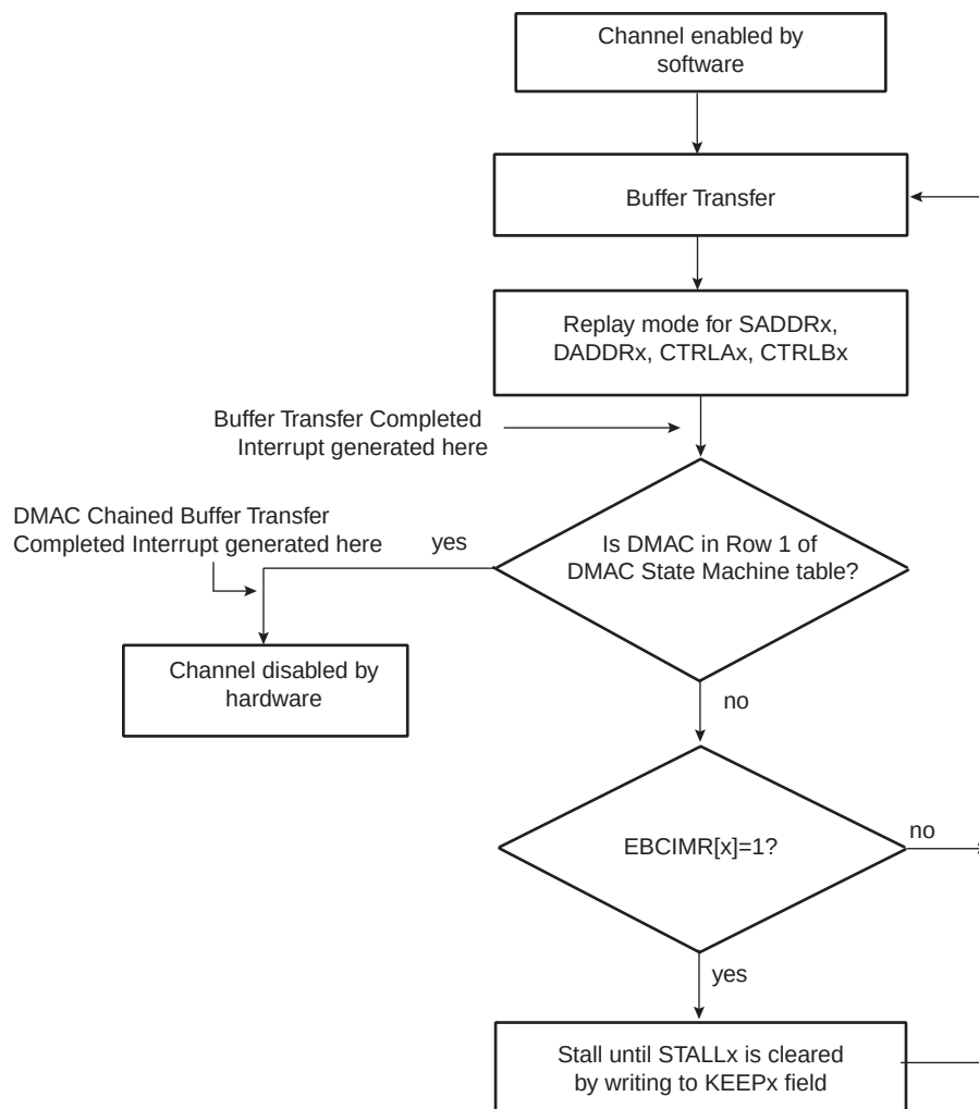
Figure 31-11.DMAC Transfer Flow for Source and Destination Address Auto-reloaded
