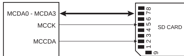
Figure 38-7. SD Card Bus Connections with One Slot
