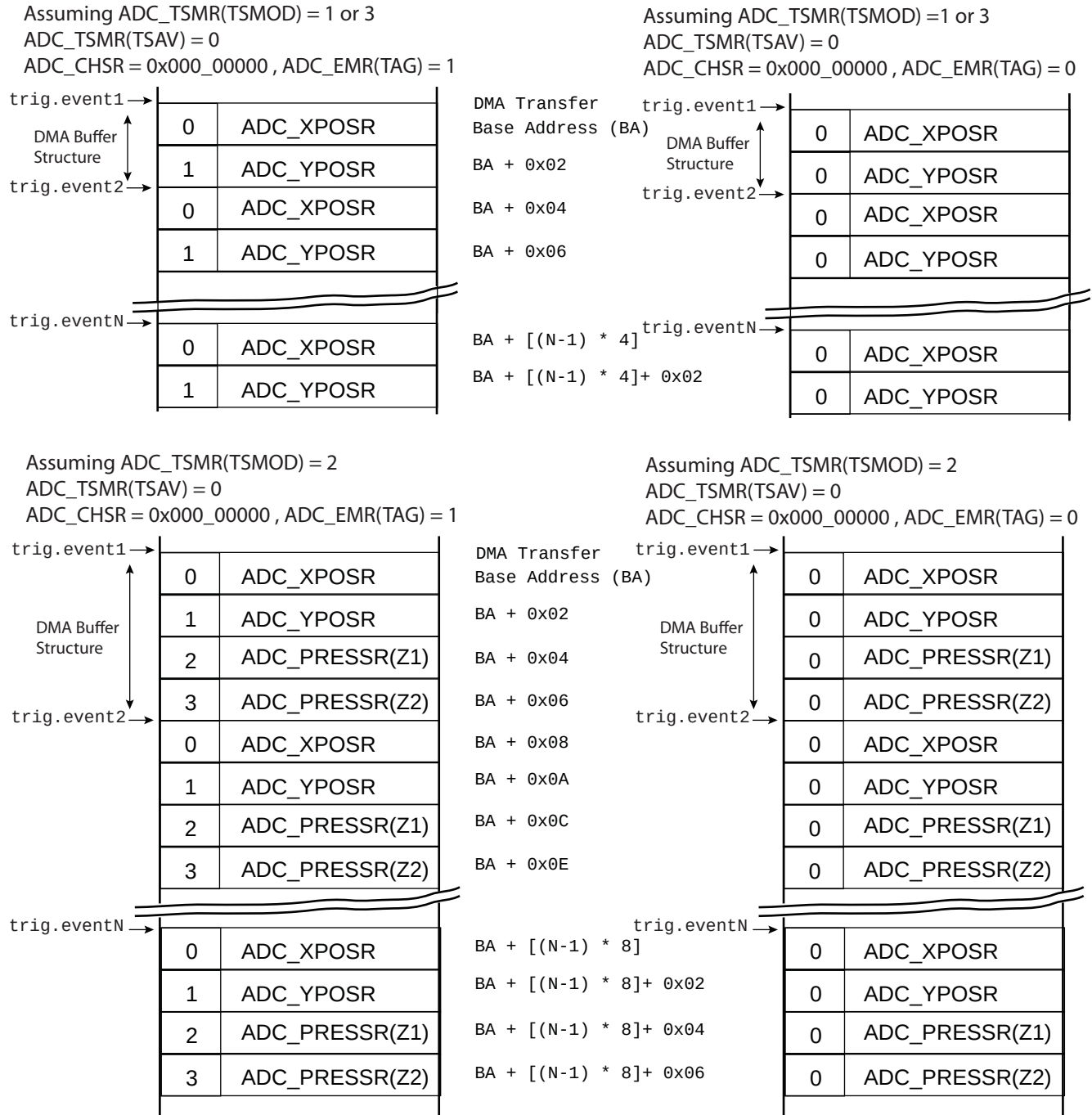
Figure 49-16. Buffer Structure when only touchscreen channels are enabled
