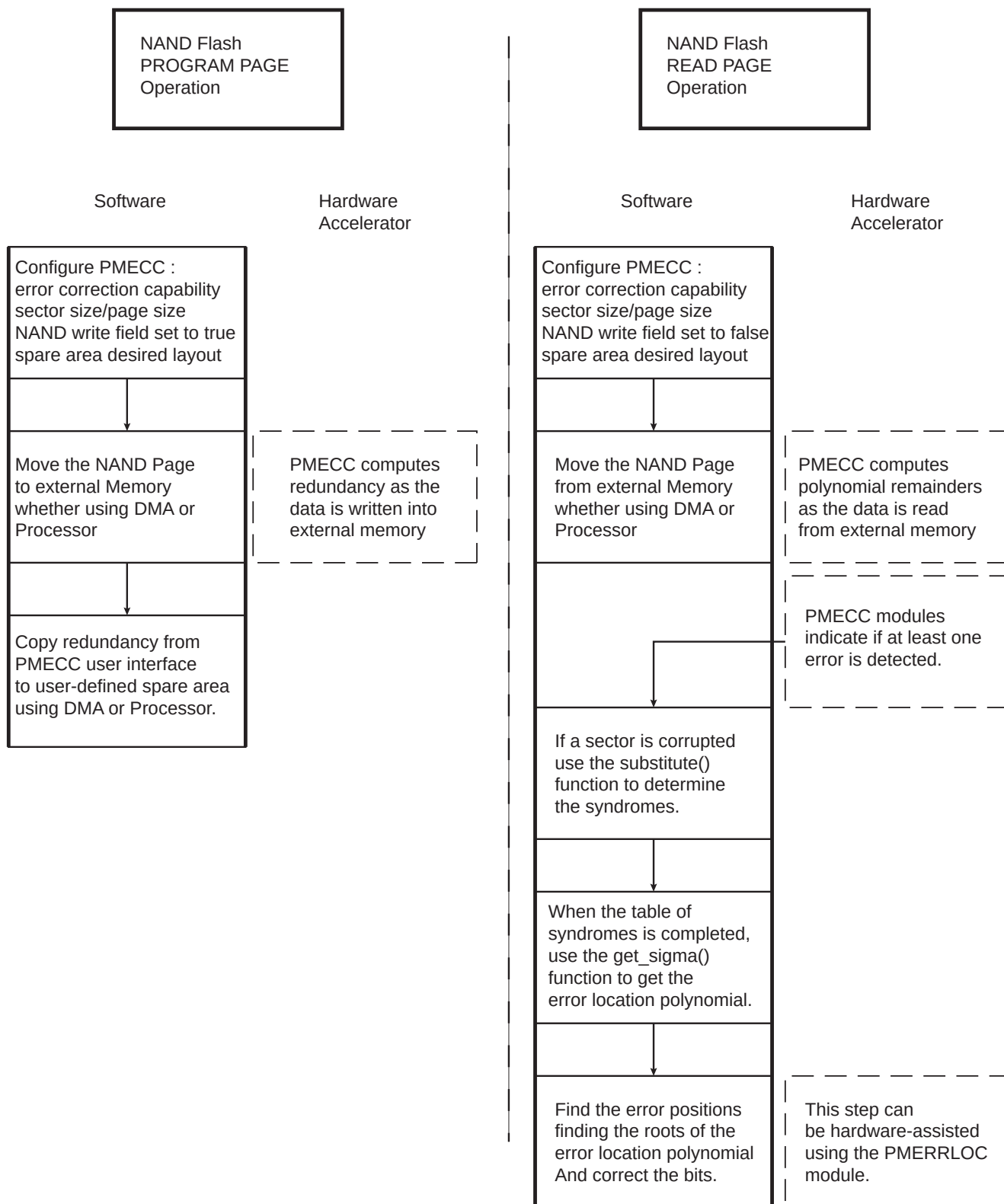
Figure 30-39. Software Hardware Multibit Error Correction Dataflow
