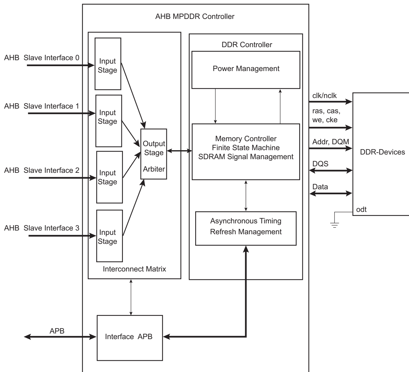
Figure 29-1. MPDDRC Module Diagram
