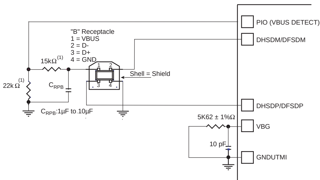
Figure 34-2. Board Schematic
