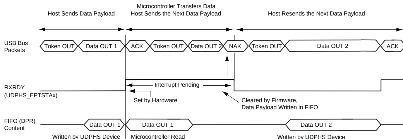
Figure 34-14.Data OUT Transfer for Endpoint with One Bank
