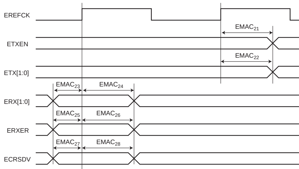
Figure 54-28.EMAC RMII Timings
