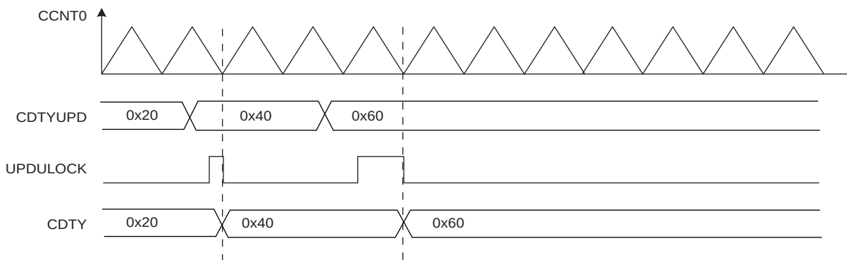
Figure 48-10. Method 1 (UPDM = 0)
